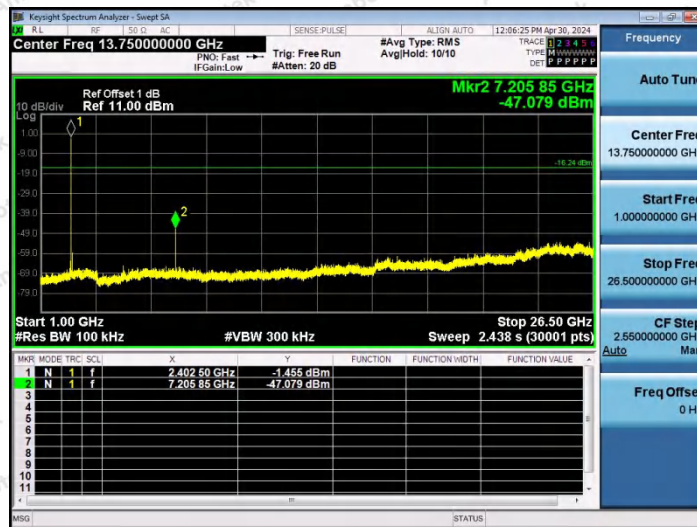
2DH5-Ant0-2402-1000~26500-PASS
