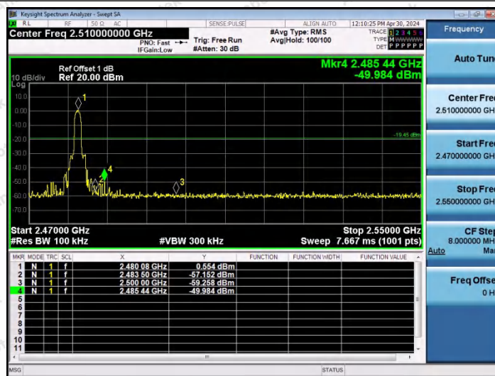
2DH5-Ant0-2480-PASS
