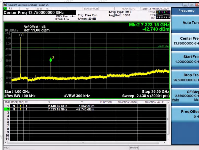
3DH5-Ant0-2441-1000~26500-PASS
