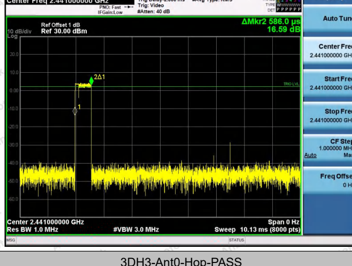
3DH3-Ant0-Hop-PASS
