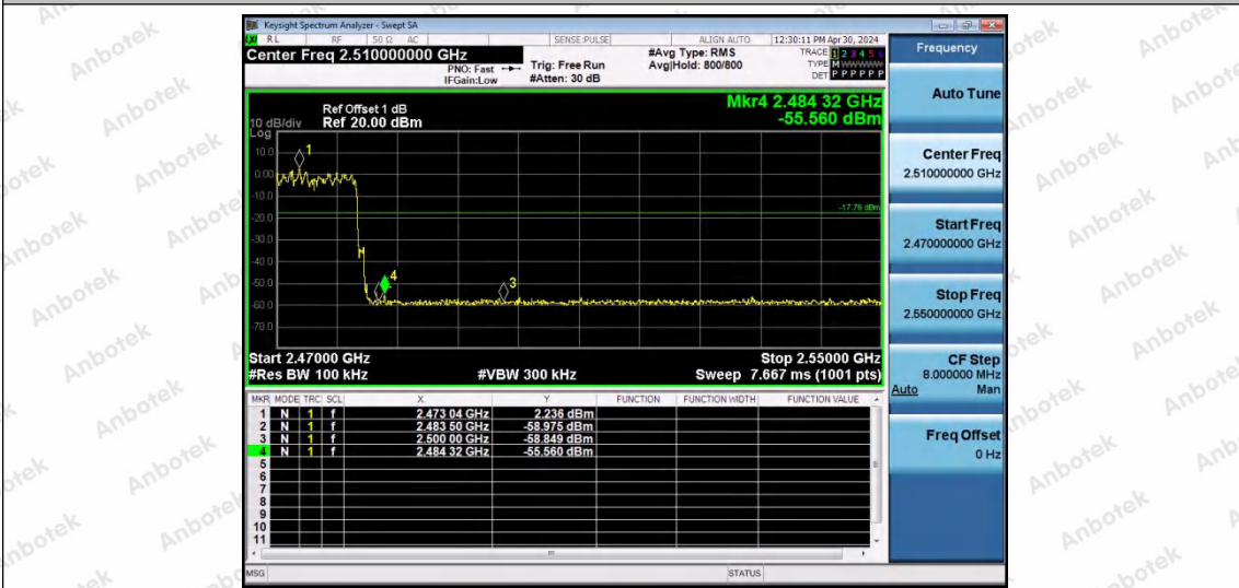
2DH5-Ant0-Hop_2480-PASS
