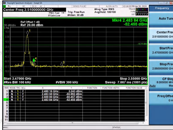
3DH5-Ant0-2480-PASS
