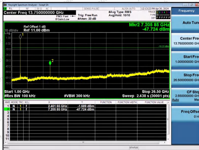
3DH5-Ant0-2402-1000~26500-PASS
