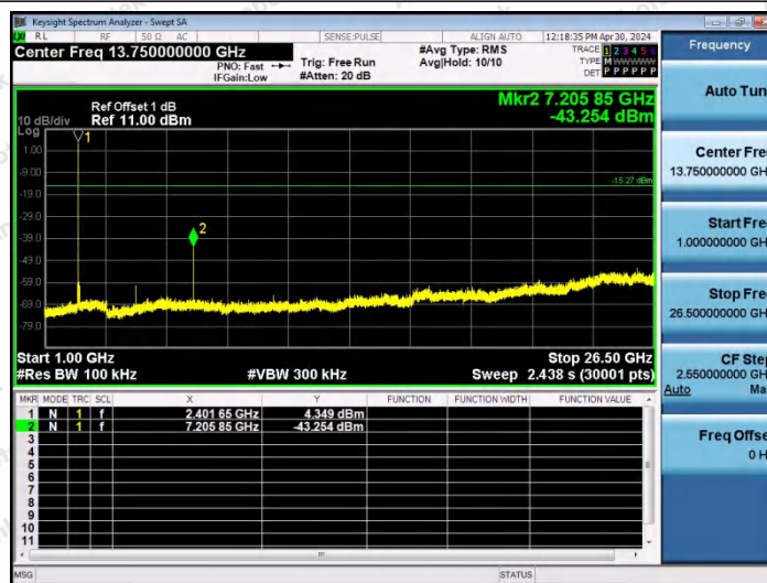
DH5-Ant0-2402-1000~26500-PASS
