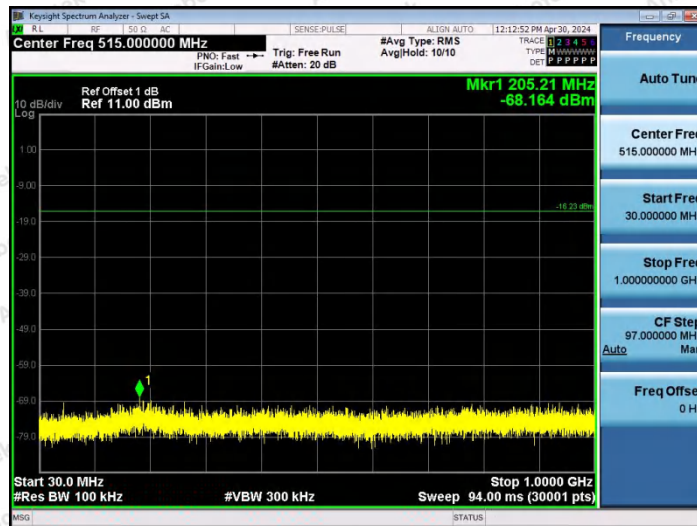
3DH5-Ant0-2402-30~1000-PASS
