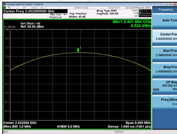
3DH5-Ant0-2402-PASS
