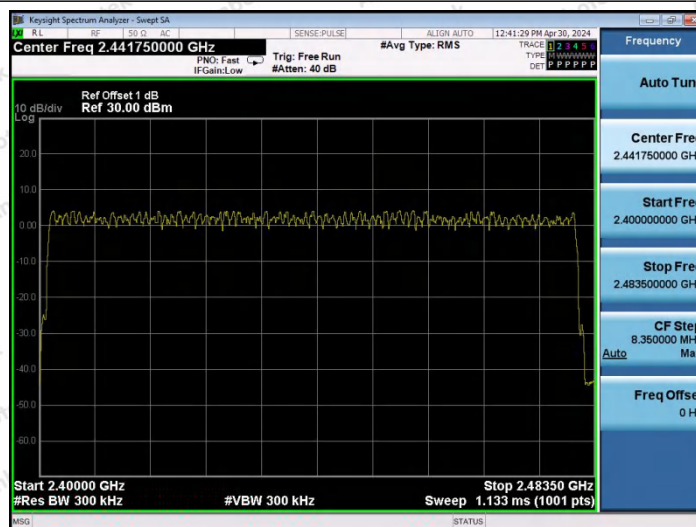
3DH5-Ant0-Hop-PASS
