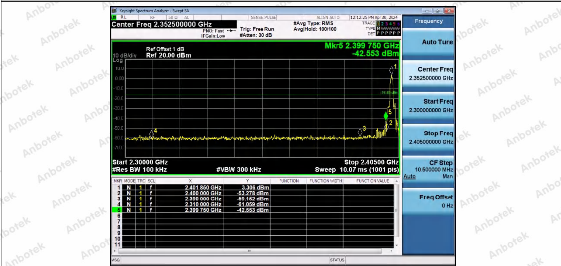
3DH5-Ant0-2402-PASS
