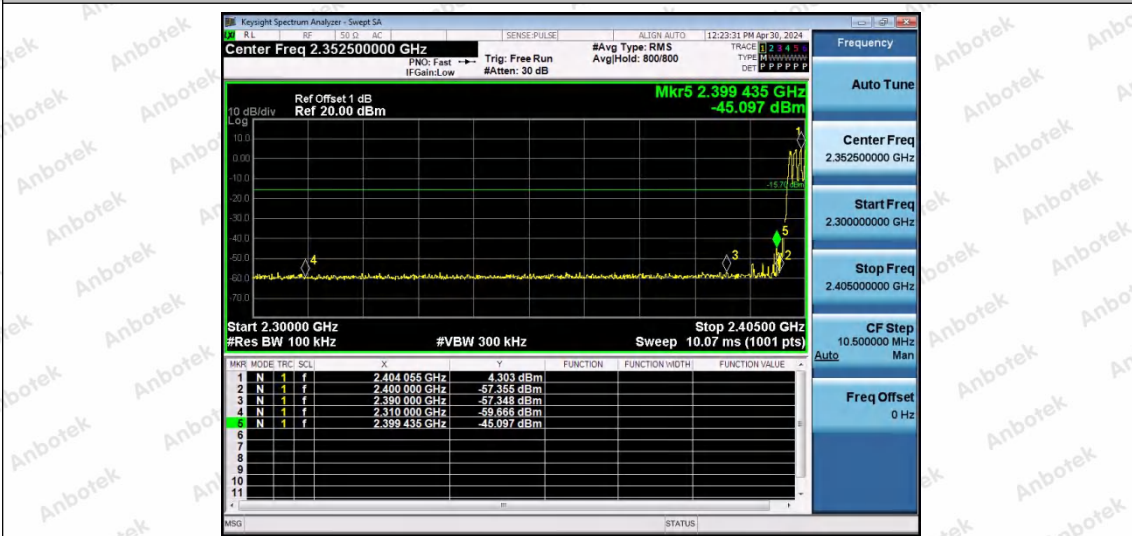
DH5-Ant0-Hop_2402-PASS
