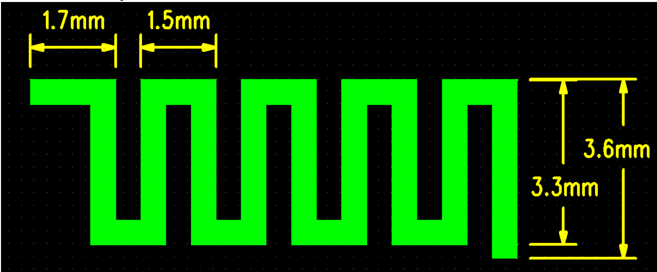
Antenna shape
