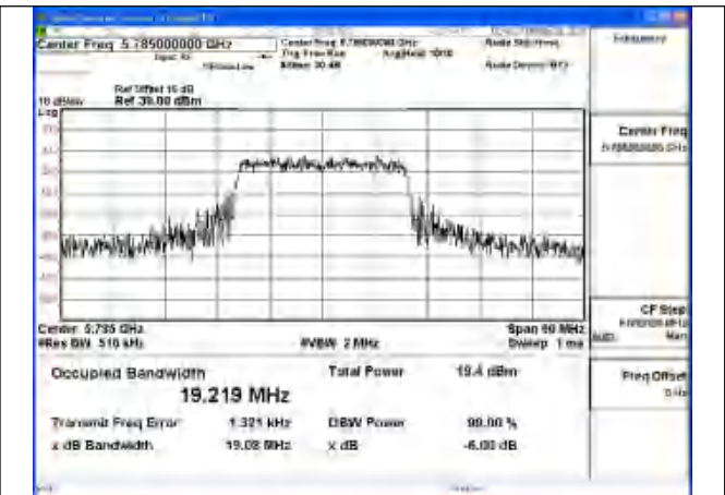
Mode:802.11ax HE20 Frequency:5785MHz Ant:Chain0
