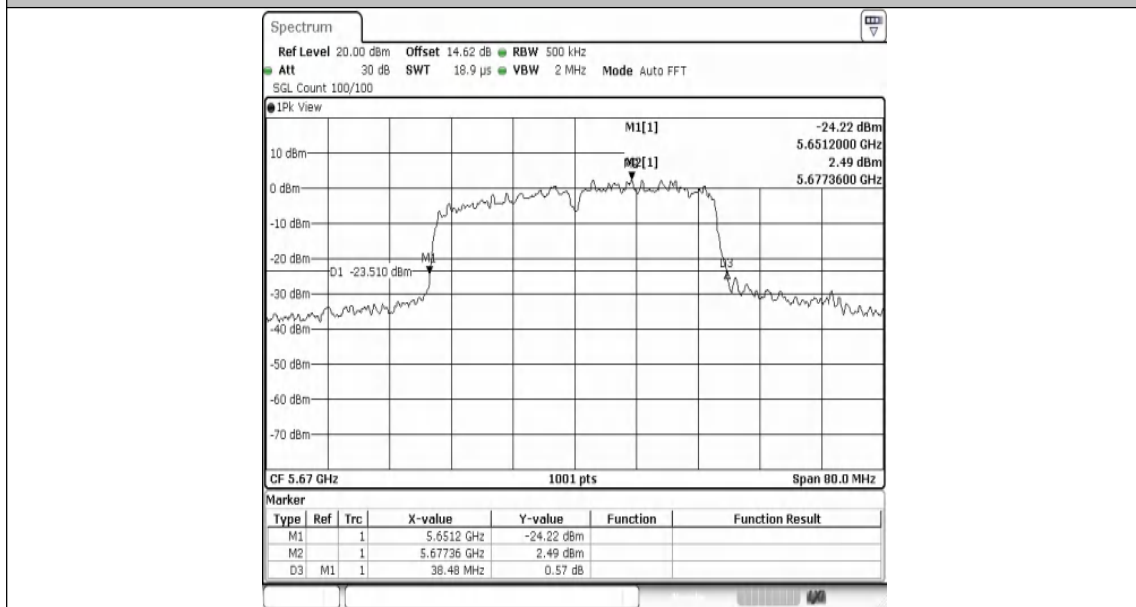
11AC40MIMO-Ant1-5670
