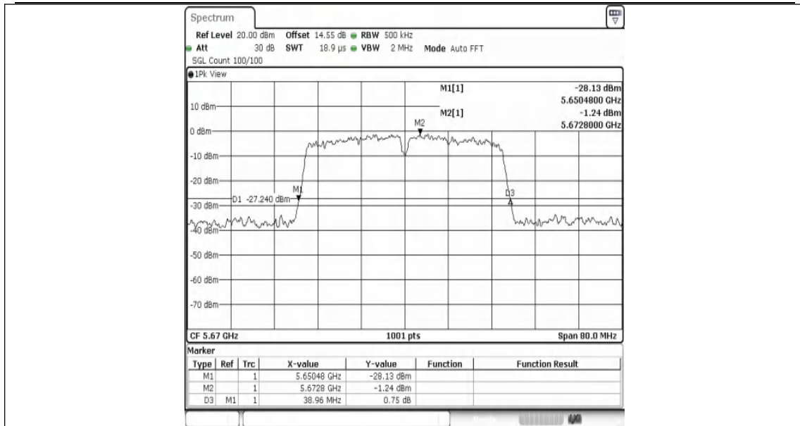
11N40MIMO-Ant1-5670
