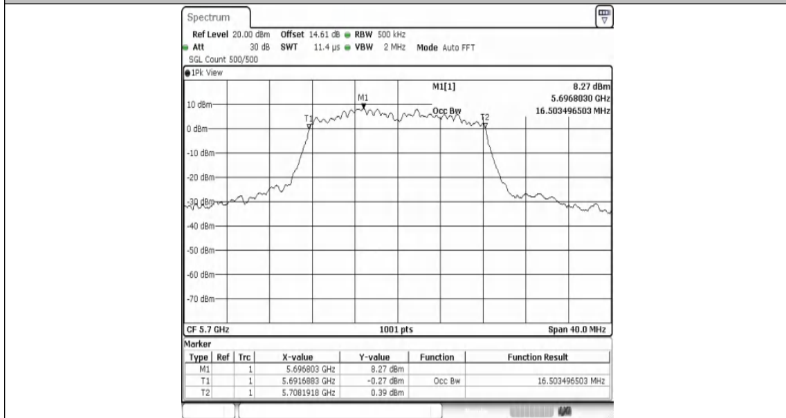
11A-Ant2-5700
