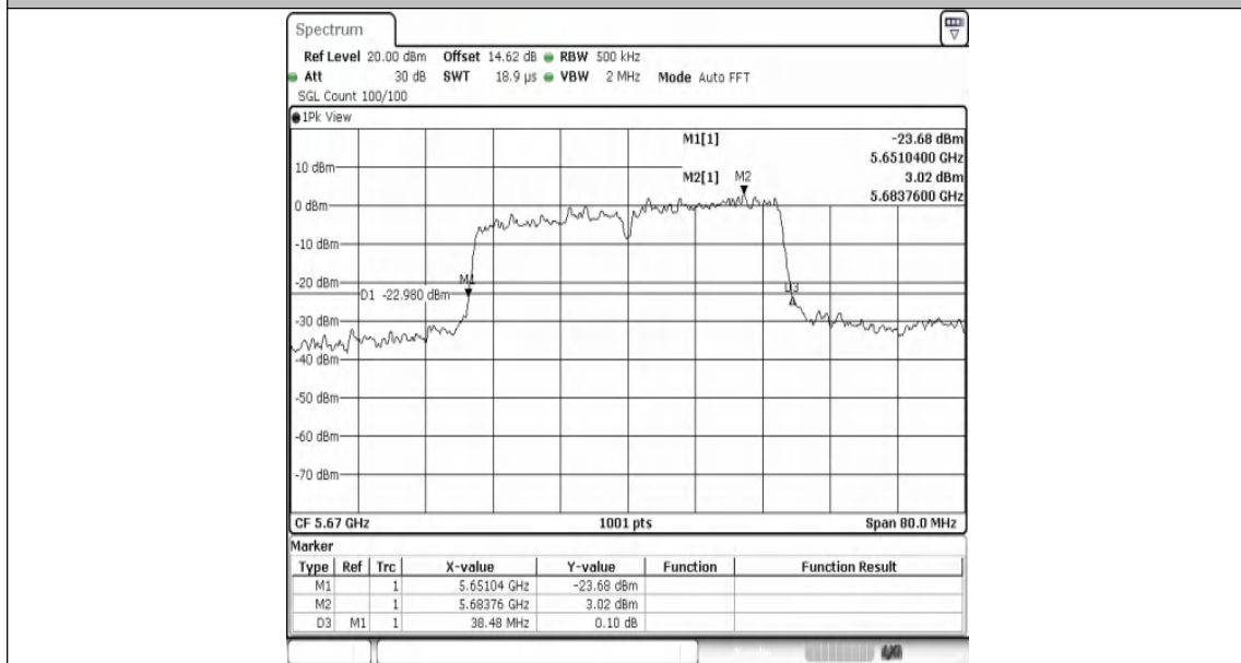
11N40MIMO-Ant1-5670
