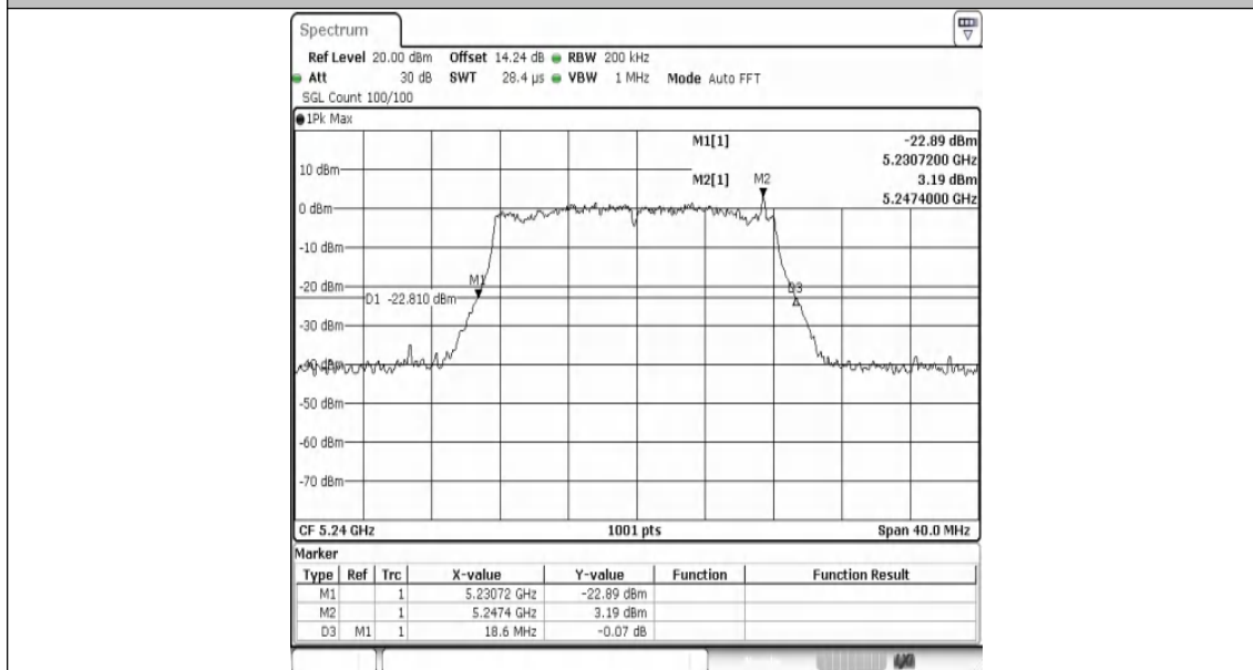
11A-Ant1-5240
