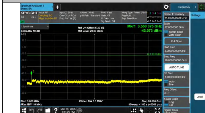
Band66-5MHz-QPSK-132647-1RB#0-3000~20000-PASS
