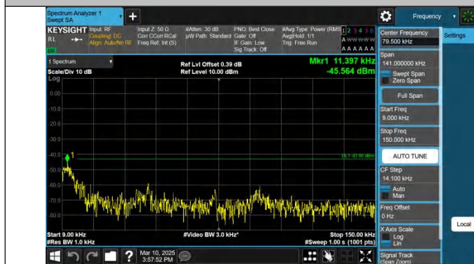
Band66-5MHz-QPSK-131997-1RB#0-0.009~0.15-PASS
