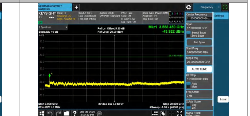
Band66-15MHz-QPSK-132597-1RB#74-3000~20000-PASS
