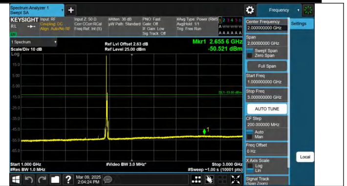
Band66-10MHz-QPSK-132622-1RB#0-1000~3000-PASS
