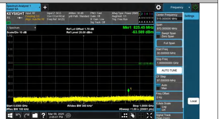
Band66-10MHz-QPSK-132622-1RB#49-30~1000-PASS
