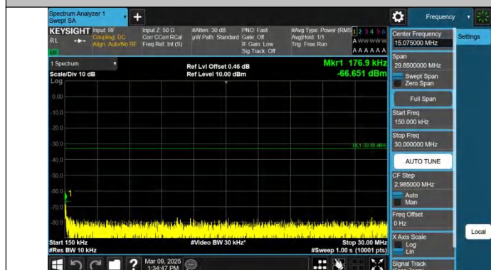
Band66-5MHz-QPSK-132647-1RB#24-0.15~30-PASS
