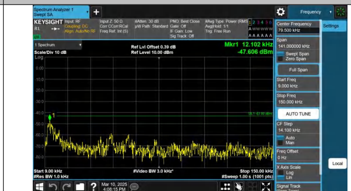
Band66-20MHz-QPSK-132322-1RB#99-0.009~0.15-PASS
