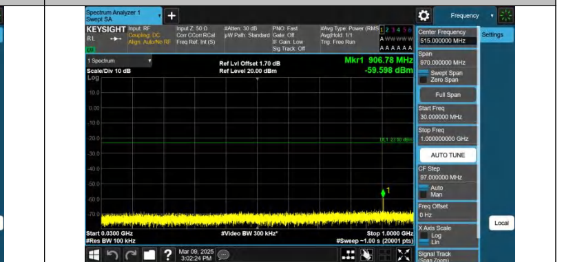
Band66-15MHz-QPSK-132597-1RB#74-30~1000-PASS
