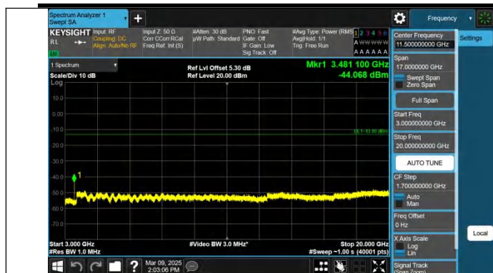
Band66-10MHz-QPSK-132322-1RB#0-3000~20000-PASS
