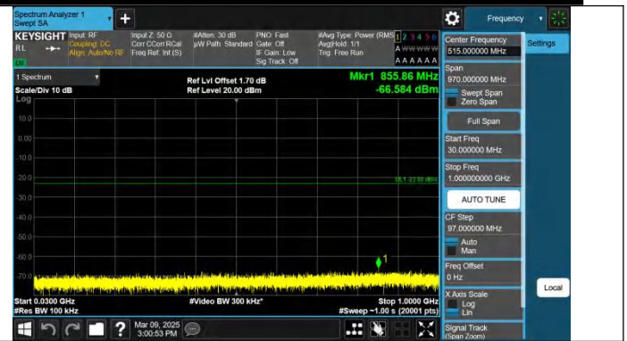
Band66-15MHz-QPSK-132322-1RB#74-30~1000-PASS
