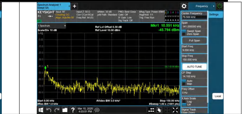
Band66-15MHz-QPSK-132597-1RB#74-0.009~0.15-PASS
