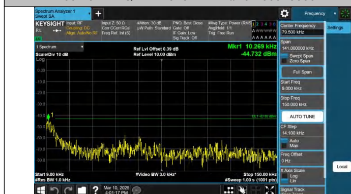
Band66-10MHz-QPSK-132622-1RB#0-0.009~0.15-PASS
