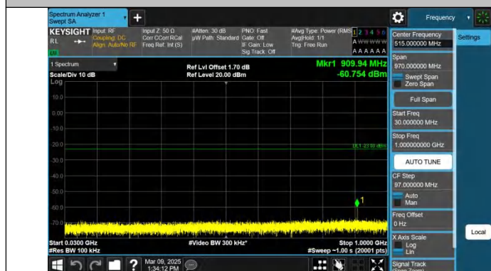
Band66-5MHz-QPSK-132647-1RB#0-30~1000-PASS
