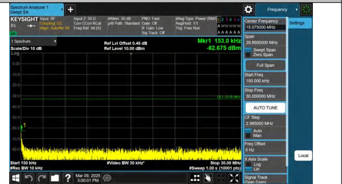
Band66-15MHz-QPSK-132322-1RB#0-0.15~30-PASS
