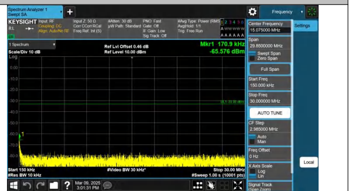
Band66-15MHz-QPSK-132597-1RB#0-0.15~30-PASS
