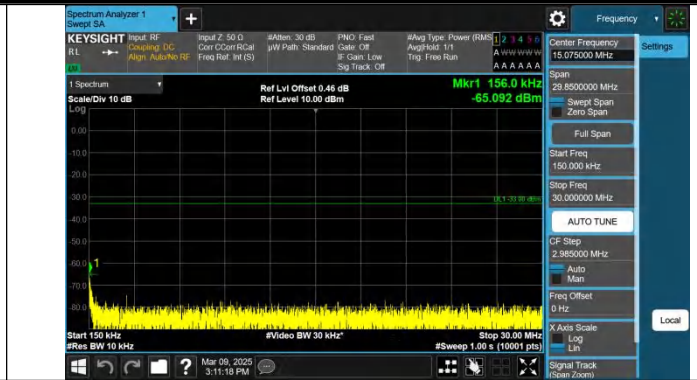
Band66-20MHz-QPSK-132322-1RB#0-0.15~30-PASS
