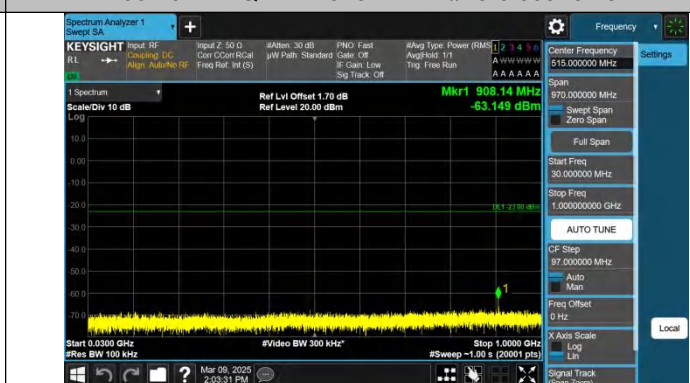
Band66-10MHz-QPSK-132322-1RB#49-30~1000-PASS
