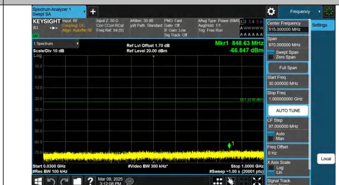
Band66-20MHz-QPSK-132322-1RB#99-30~1000-PASS
