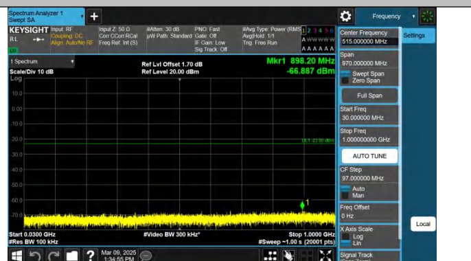
Band66-5MHz-QPSK-132647-1RB#24-30~1000-PASS
