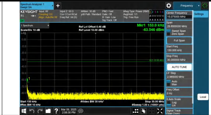
Band66-15MHz-QPSK-132047-1RB#0-0.15~30-PASS
