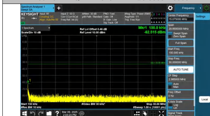
Band66-10MHz-QPSK-132322-1RB#49-0.15~30-PASS
