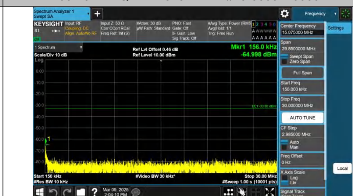
Band66-10MHz-QPSK-132622-1RB#0-0.15~30-PASS
