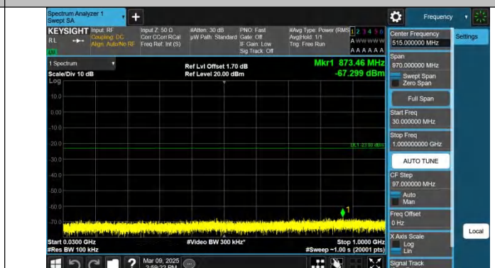
Band66-15MHz-QPSK-132047-1RB#74-30~1000-PASS
