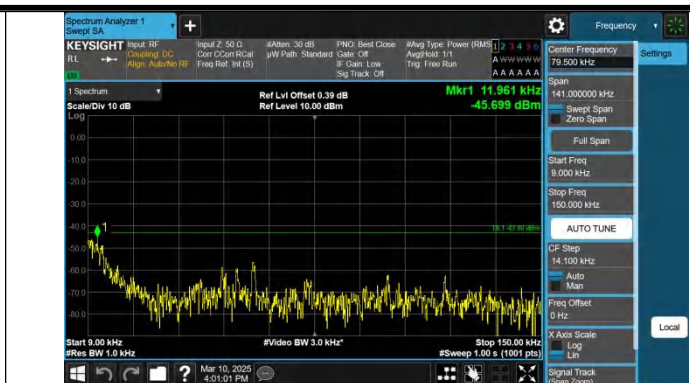
Band66-10MHz-QPSK-132322-1RB#49-0.009~0.15-PASS
