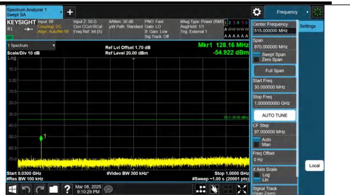
Band41-10MHz-QPSK-41540-1RB#49-30~1000-PASS
