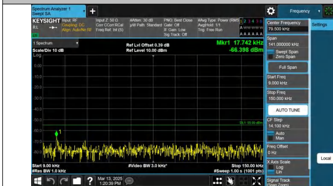
Band41-20MHz-QPSK-39750-1RB#0-0.009~0.15-PASS
