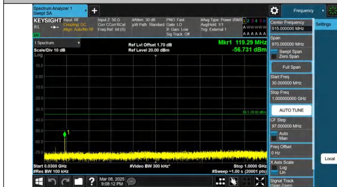
Band41-10MHz-QPSK-41540-1RB#0-30~1000-PASS
