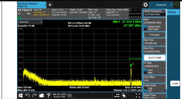
Band41-10MHz-QPSK-40620-1RB#0-0.15~30-PASS
