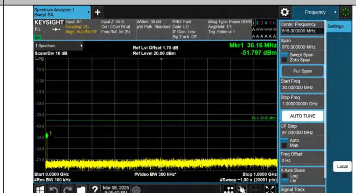
Band41-10MHz-QPSK-40620-1RB#49-30~1000-PASS
