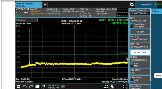
Band41-20MHz-QPSK-39750-1RB#99-1000~20000-PASS
