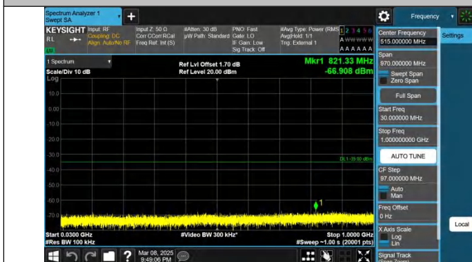
Band41-20MHz-QPSK-39750-1RB#0-30~1000-PASS
