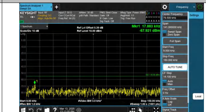
Band41-10MHz-QPSK-40620-1RB#49-0.009~0.15-PASS
