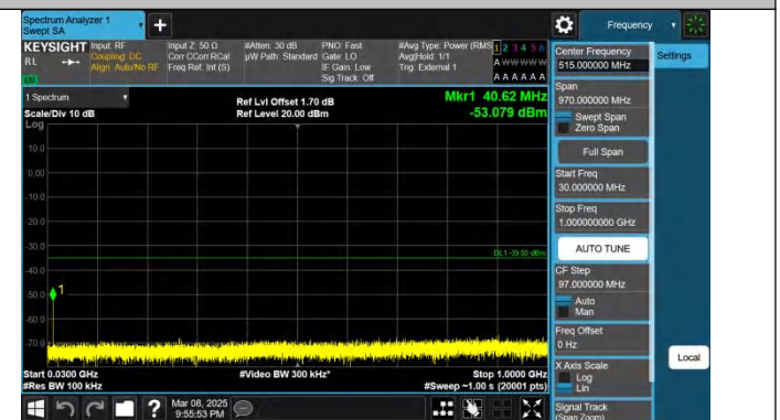
Band41-20MHz-QPSK-40620-1RB#99-30~1000-PASS
