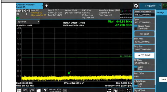
Band41-20MHz-QPSK-40620-1RB#0-30~1000-PASS
