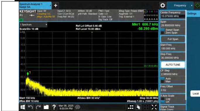
Band41-20MHz-QPSK-39750-1RB#99-0.15~30-PASS
