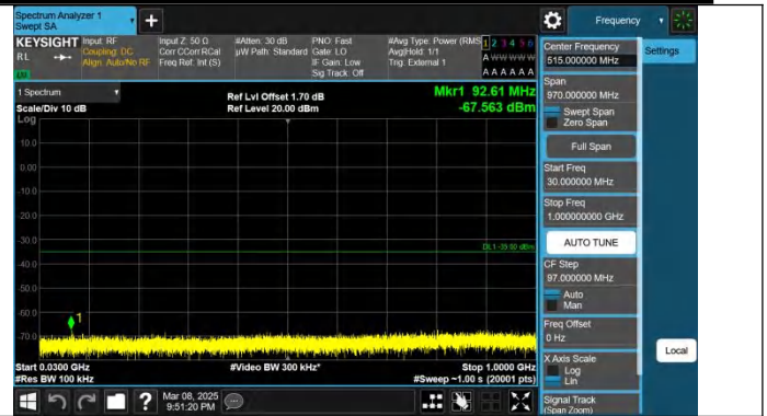
Band41-20MHz-QPSK-39750-1RB#99-30~1000-PASS
