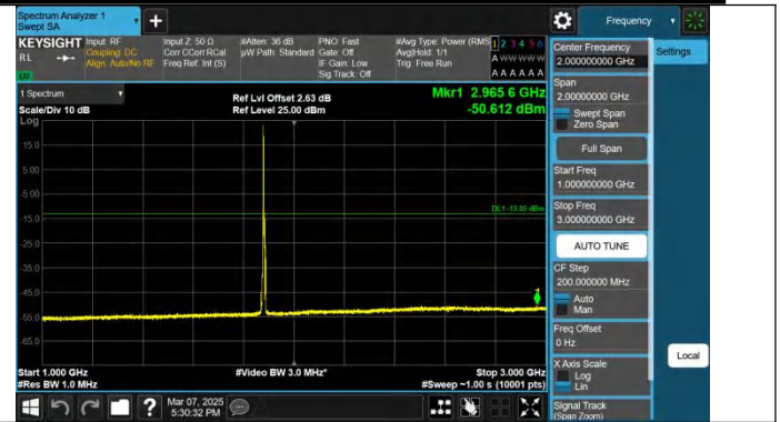
Band2-5MHz-QPSK-18900-1RB#0-1000~3000-PASS
