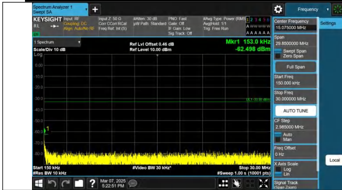
Band2-3MHz-QPSK-19185-1RB#14-0.15~30-PASS
