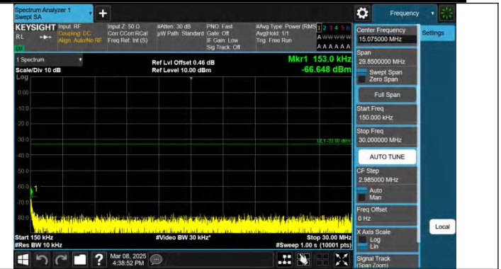
Band2-15MHz-QPSK-18675-1RB#0-0.15~30-PASS
