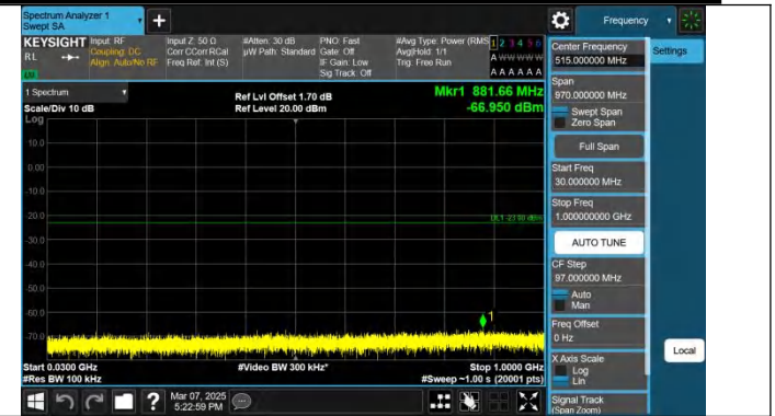
Band2-3MHz-QPSK-19185-1RB#14-30~1000-PASS
