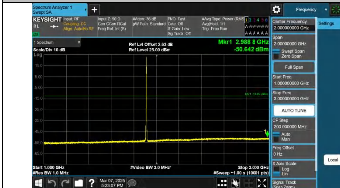
Band2-3MHz-QPSK-19185-1RB#14-1000~3000-PASS
