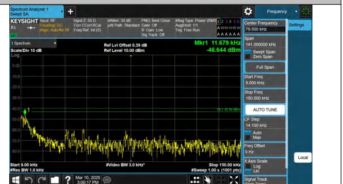
Band2-15MHz-QPSK-18675-1RB#74-0.009~0.15-PASS
