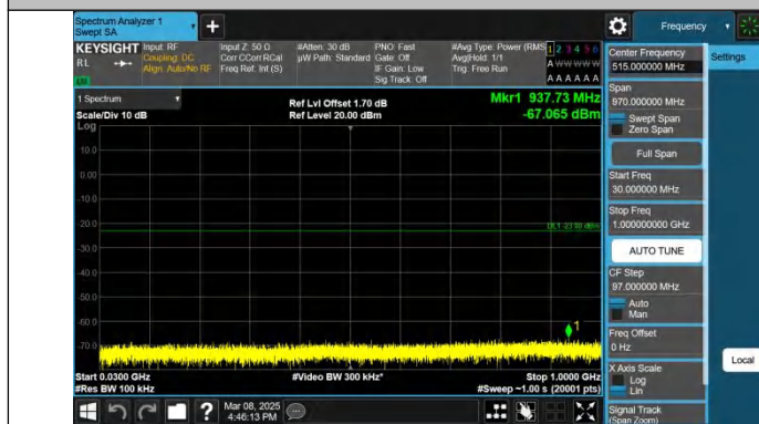
Band2-20MHz-QPSK-19100-1RB#0-30~1000-PASS
