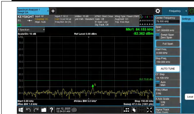
48-48-20MHz-20MHz-QPSK-QPSK-56442-56640-1RB#0-0RB#0- 0.009~0.15MHz-PASS
