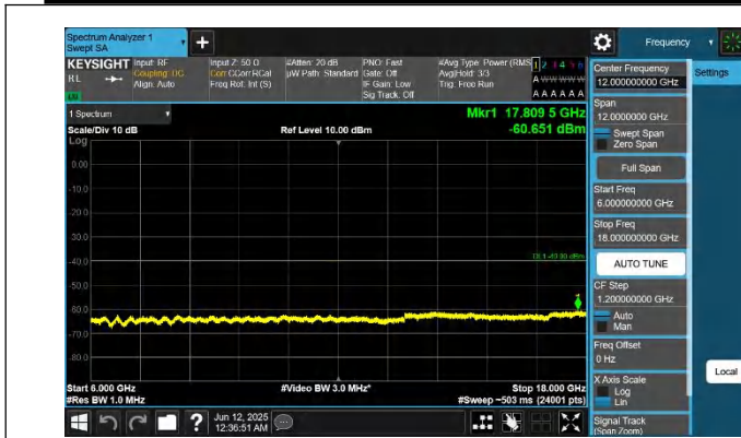
48-48-20MHz-20MHz-QPSK-QPSK-56442-56640-1RB#0-1RB#9 9-6000~18000MHz-PASS
