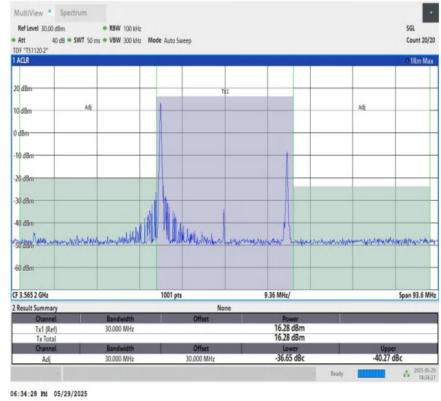
48-48-10MHz-20MHz-64QAM-64QAM-55295-55439-1RB#0-1RB#9 9-PASS
