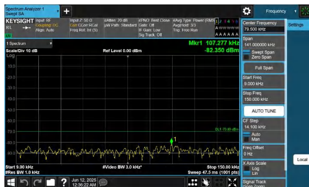
48-48-20MHz-20MHz-QPSK-QPSK-56442-56640-1RB#0-1RB#9 9-0.009~0.15MHz-PASS
