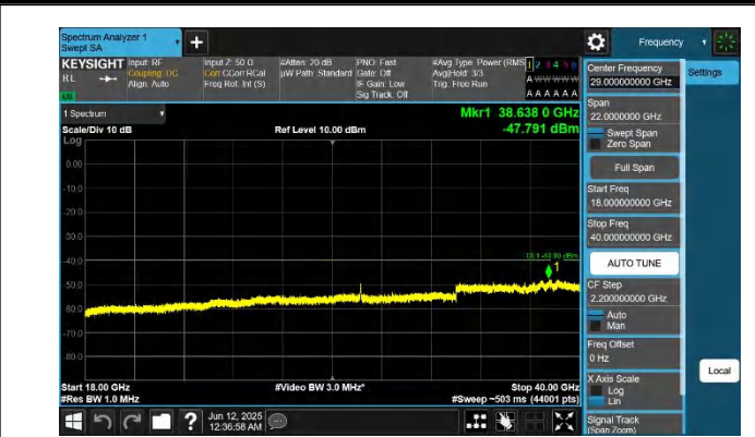
48-48-20MHz-20MHz-QPSK-QPSK-56442-56640-1RB#0-1RB#9 9-18000~40000MHz-PASS
