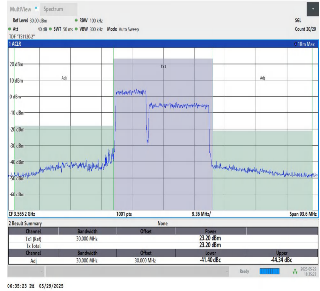
48-48-10MHz-20MHz-64QAM-64QAM-55295-55439-50RB#0-100R B#0-PASS
