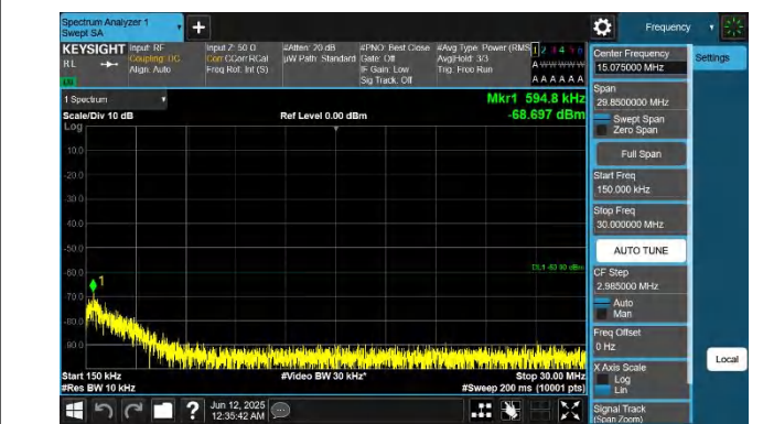
48-48-20MHz-20MHz-QPSK-QPSK-56442-56640-1RB#99-0RB# 0-0.15~30MHz-PASS
