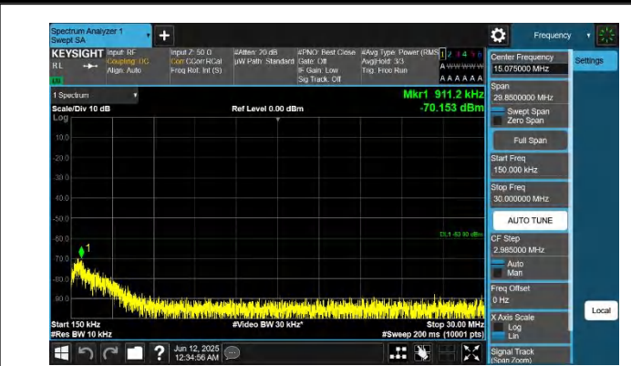
48-48-20MHz-20MHz-QPSK-QPSK-56442-56640-1RB#0-0RB#0- 0.15~30MHz-PASS
