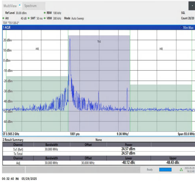
48-48-10MHz-20MHz-64QAM-64QAM-55295-55439-1RB#0-0R B#0-PASS
