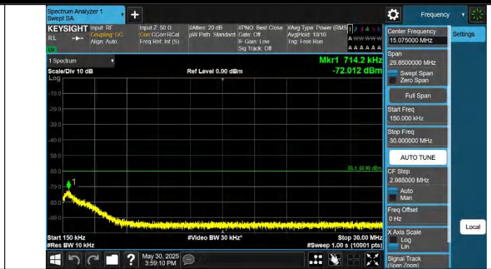
Band48-20MHz-QPSK-55340-1RB#0-0.15~30-PASS
