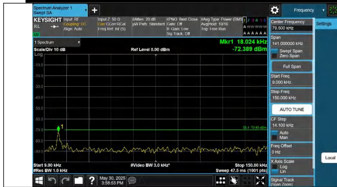
Band48-20MHz-QPSK-55340-1RB#0-0.009~0.15-PASS
