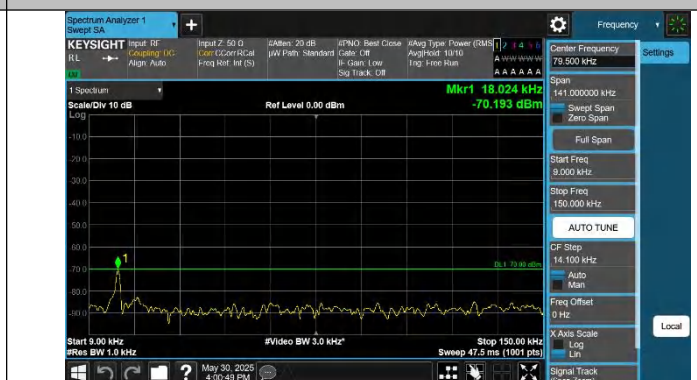
Band48-20MHz-QPSK-55340-1RB#99-0.009~0.15-PASS
