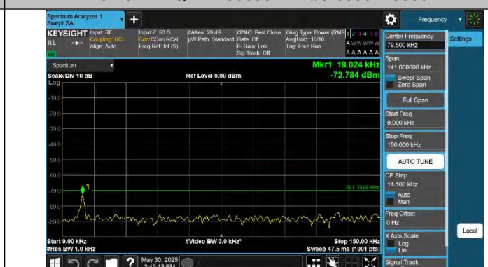
Band48-10MHz-QPSK-56690-1RB#49-0.009~0.15-PASS
