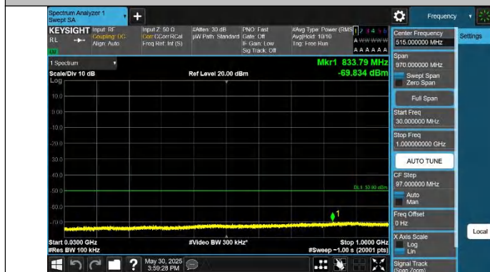
Band48-20MHz-QPSK-55340-1RB#0-30~1000-PASS
