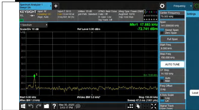
Band48-10MHz-QPSK-56690-1RB#0-0.009~0.15-PASS
