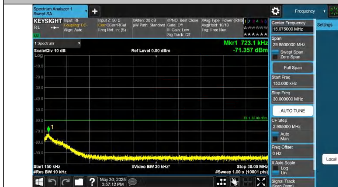
Band48-15MHz-QPSK-56665-1RB#74-0.15~30-PASS
