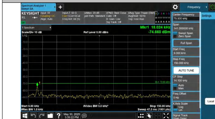
Band48-10MHz-QPSK-55990-1RB#0-0.009~0.15-PASS
