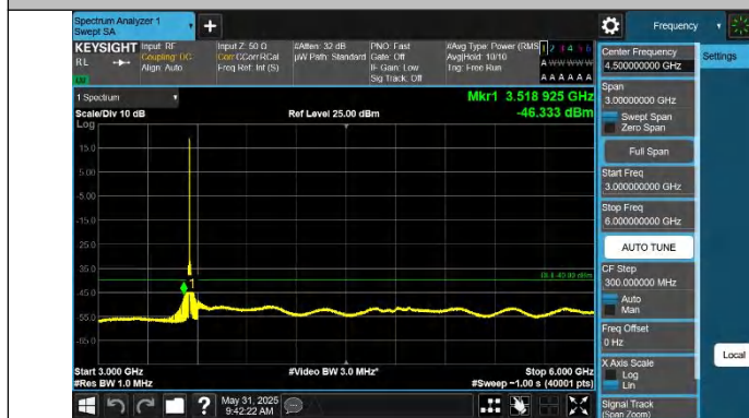
Band48-20MHz-QPSK-55340-1RB#0-3000~6000-PASS
