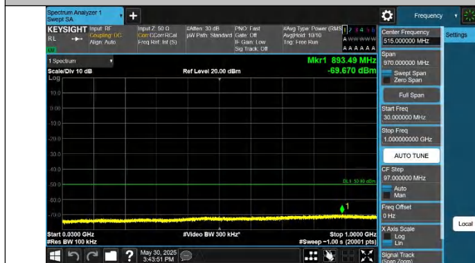
Band48-10MHz-QPSK-56690-1RB#0-30~1000-PASS
