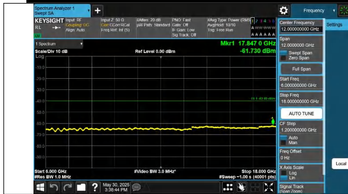
Band48-10MHz-QPSK-55290-1RB#49-6000~18000-PASS
