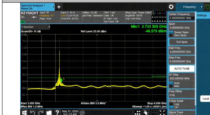
Band48-15MHz-QPSK-56665-1RB#0-3000~6000-PASS
