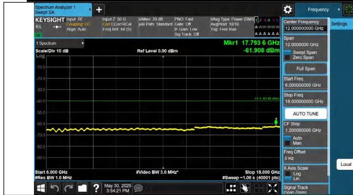
Band48-15MHz-QPSK-55990-1RB#74-6000~18000-PASS
