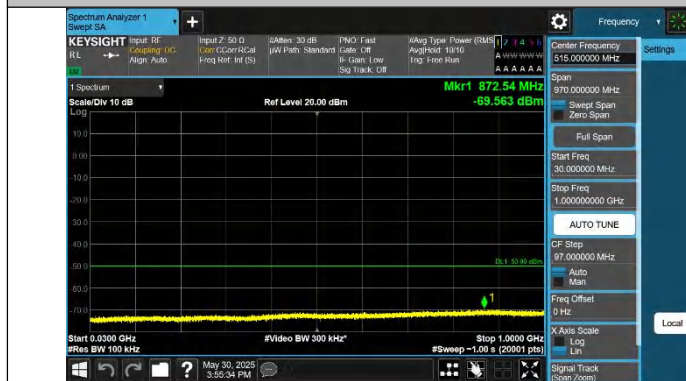
Band48-15MHz-QPSK-56665-1RB#0-30~1000-PASS
