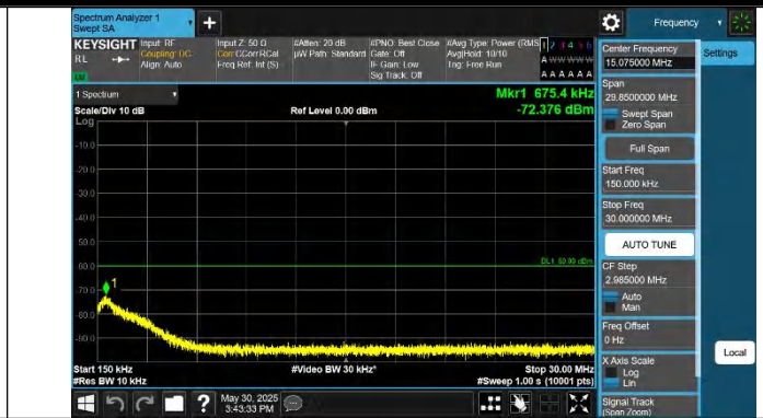
Band48-10MHz-QPSK-56690-1RB#0-0.15~30-PASS
