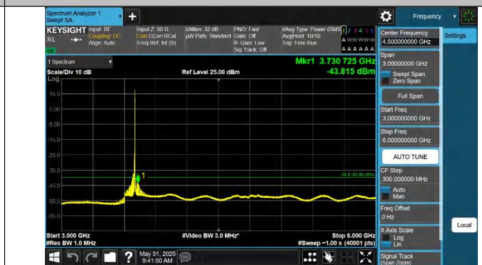
Band48-15MHz-QPSK-56665-1RB#74-3000~6000-PASS
