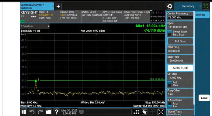
Band48-15MHz-QPSK-56665-1RB#74-0.009~0.15-PASS
