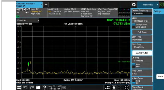
Band48-15MHz-QPSK-56665-1RB#0-0.009~0.15-PASS
