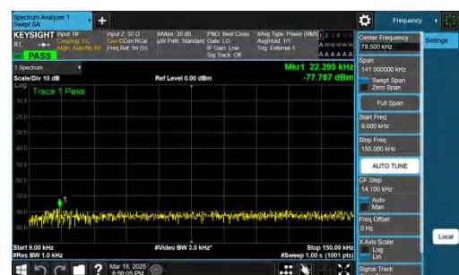
NTNV-n48-PC3-30-20-M-DFT-BPSK-Inner_1RB_Right-0.009-0.15-PASS
