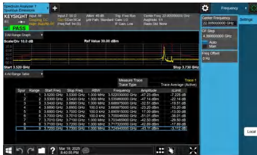
NTNV-n48-PC3-30-10-H-DFT-BPSK-Edge_1RB_Left-PASS
