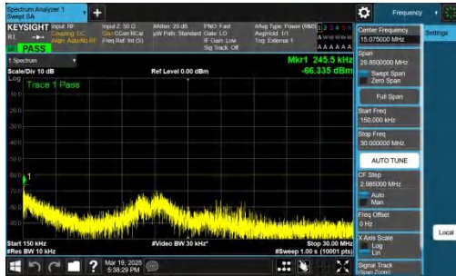
NTNV-n48-PC3-30-10-L-DFT-BPSK-Inner_1RB_Right-0.15-30-P ASS
