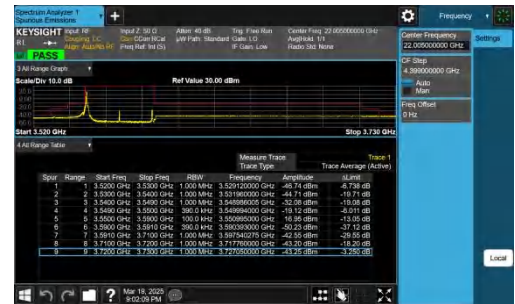
NTNV-n48-PC3-30-40-L-DFT-BPSK-Edge_1RB_Left-PASS
