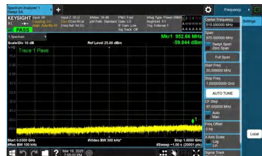
NTNV-n48-PC3-30-40-M-DFT-BPSK-Inner_1RB_Right-30-1000-PASS
