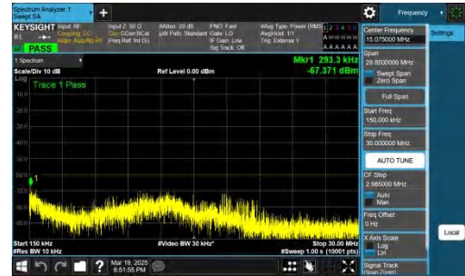
NTNV-n48-PC3-30-20-M-DFT-BPSK-Inner_1RB_Left-0.15-30-PASS
