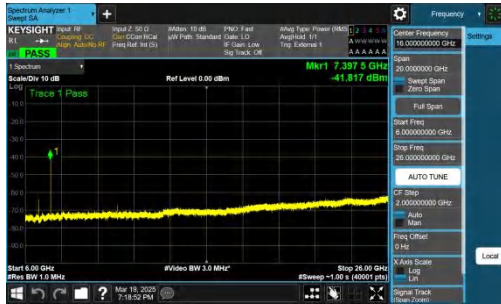
NTNV-n48-PC3-30-20-H-DFT-BPSK-Inner_1RB_Right-6000-26000-PASS
