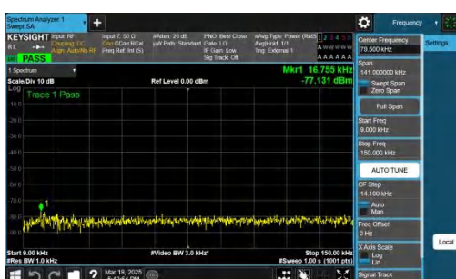
NTNV-n48-PC3-30-10-L-DFT-QPSK-Inner_1RB_Left-0.009-0.15- PASS
