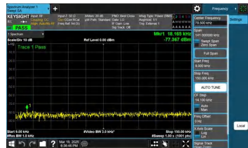
NTNV-n48-PC3-30-20-L-DFT-BPSK-Inner_1RB_Right-0.009-0.15-PASS
