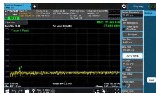
NTNV-n48-PC3-30-40-L-DFT-BPSK-Inner_1RB_Right-0.009-0.15-PASS
