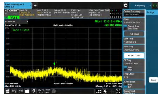
NTNV-n48-PC3-30-20-H-DFT-QPSK-Inner_1RB_Left-0.15-30-PASS
