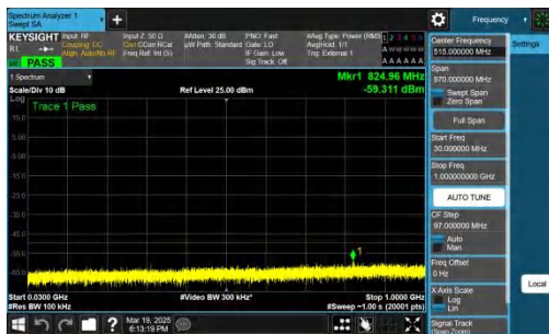
NTNV-n48-PC3-30-10-H-DFT-BPSK-Inner_1RB_Left-30-1000-PASS
