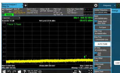
NTNV-n48-PC3-30-40-M-DFT-BPSK-Inner_1RB_Left-30-1000-P ASS
