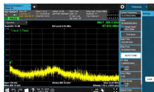
NTNV-n48-PC3-30-40-L-DFT-QPSK-Inner_1RB_Left-0.15-30-PAS S
