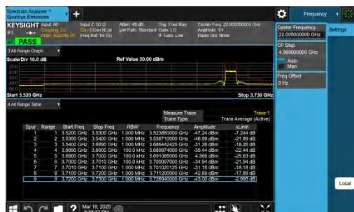
NTNV-n48-PC3-30-10-H-DFT-BPSK-Outer Full-PASS
