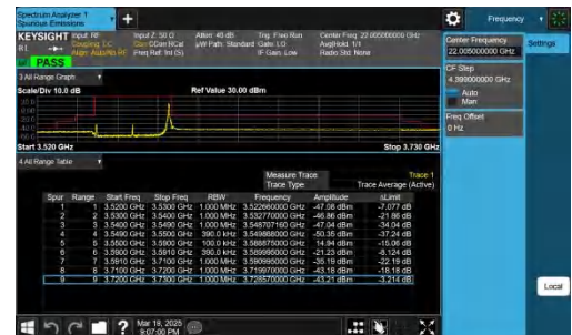
NTNV-n48-PC3-30-40-L-DFT-QPSK-Edge_1RB_Right-PASS
