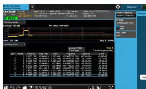
NTNV-n48-PC3-30-10-L-DFT-QPSK-Outer Full-PASS
