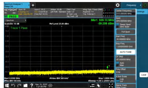
NTNV-n48-PC3-30-20-H-DFT-QPSK-Inner_1RB_Right-30-1000-P ASS
