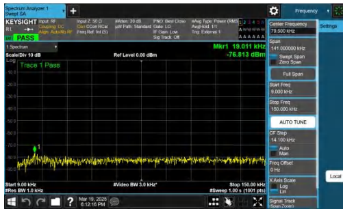
NTNV-n48-PC3-30-10-H-DFT-BPSK-Inner_1RB_Left-0.009-0.15-PASS
