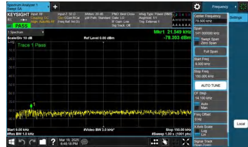
NTNV-n48-PC3-30-20-L-DFT-QPSK-Inner_1RB_Right-0.009-0.15- PASS
