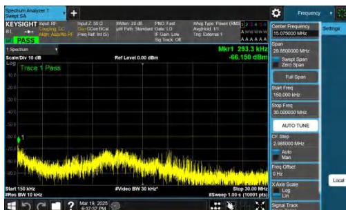
NTNV-n48-PC3-30-20-L-DFT-BPSK-Inner_1RB_Right-0.15-30-PASS
