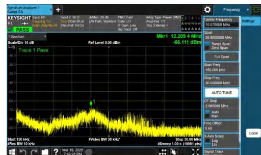
NTNV-n48-PC3-30-40-M-DFT-BPSK-Inner_1RB_Left-0.15-30-PAS S
