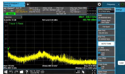
NTNV-n48-PC3-30-10-M-DFT-QPSK-Inner_1RB_Left-0.15-30-PA-SS
