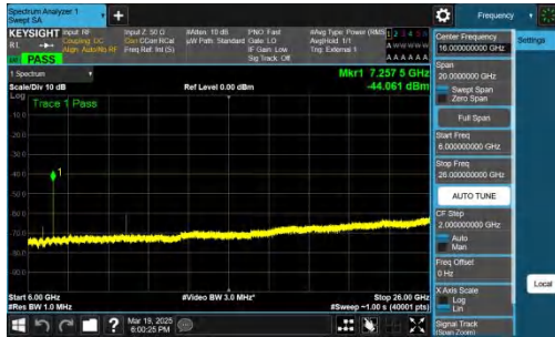
NTNV-n48-PC3-30-10-M-DFT-BPSK-Inner_1RB_Right-6000-26000-PASS
