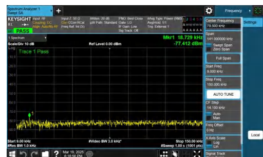
NTNV-n48-PC3-30-10-H-DFT-BPSK-Inner_1RB_Right-0.009-0.15-PASS
