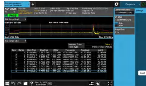
NTNV-n48-PC3-30-10-H-DFT-QPSK-Edge_1RB_Left-PASS
