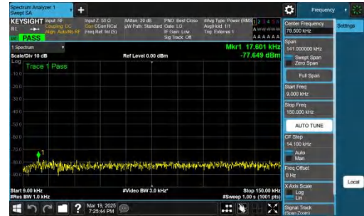
NTNV-n48-PC3-30-20-H-DFT-QPSK-Inner_1RB_Right-0.009-0.15 -PASS
