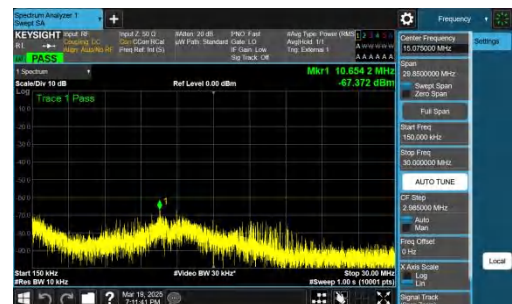
NTNV-n48-PC3-30-20-H-DFT-BPSK-Inner_1RB_Left-0.15-30-PAS S
