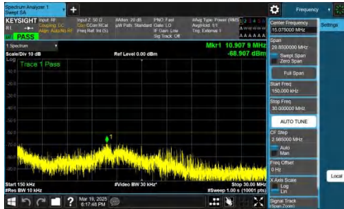
NTNV-n48-PC3-30-10-H-DFT-BPSK-Inner_1RB_Right-0.15-30-P ASS
