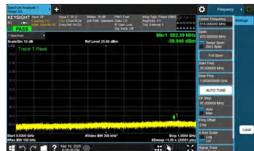
NTNV-n48-PC3-30-20-L-DFT-BPSK-Inner_1RB_Right-30-1000-PASS
