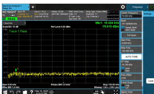
NTNV-n48-PC3-30-10-H-DFT-QPSK-Inner_1RB_Left-0.009-0.15- PASS
