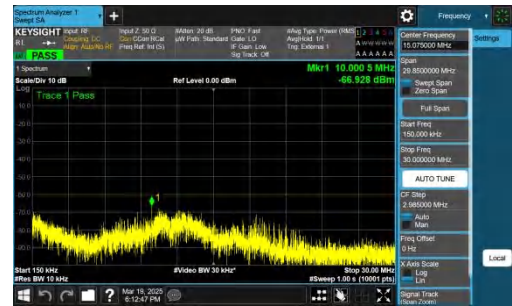
NTNV-n48-PC3-30-10-H-DFT-BPSK-Inner_1RB_Left-0.15-30-PASS
