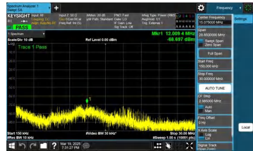
NTNV-n48-PC3-30-40-L-DFT-BPSK-Inner_1RB_Left-0.15-30-PASS
