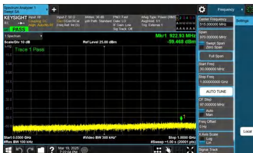
NTNV-n48-PC3-30-20-H-DFT-QPSK-Inner_1RB_Left-30-1000-PASS
