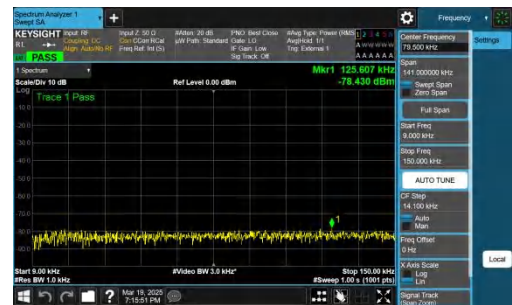
NTNV-n48-PC3-30-20-H-DFT-BPSK-Inner_1RB_Right-0.009-0.15-PASS
