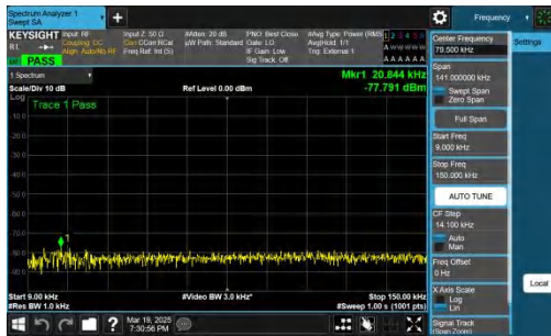
NTNV-n48-PC3-30-40-L-DFT-BPSK-Inner_1RB_Left-0.009-0.15-PASS
