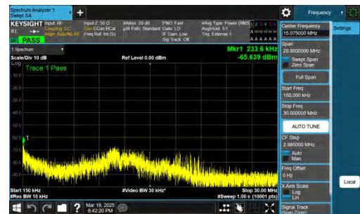
NTNV-n48-PC3-30-20-L-DFT-QPSK-Inner_1RB_Left-0.15-30-PAS S
