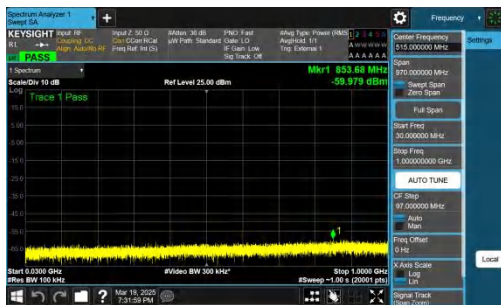
NTNV-n48-PC3-30-40-L-DFT-BPSK-Inner_1RB_Left-30-1000-PASS
