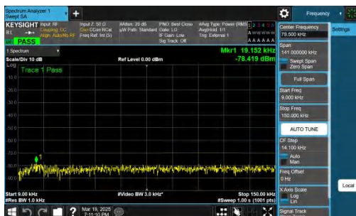
NTNV-n48-PC3-30-20-H-DFT-BPSK-Inner_1RB_Left-0.009-0.15- PASS
