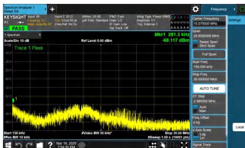
NTNV-n48-PC3-30-40-M-DFT-BPSK-Inner_1RB_Right-0.15-30-PASS
