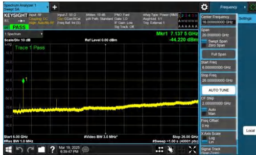
NTNV-n48-PC3-30-20-L-DFT-BPSK-Inner_1RB_Right-6000-2600 0-PASS
