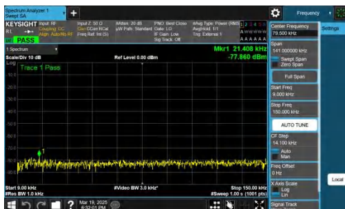
NTNV-n48-PC3-30-20-L-DFT-BPSK-Inner_1RB_Left-0.009-0.15- PASS
