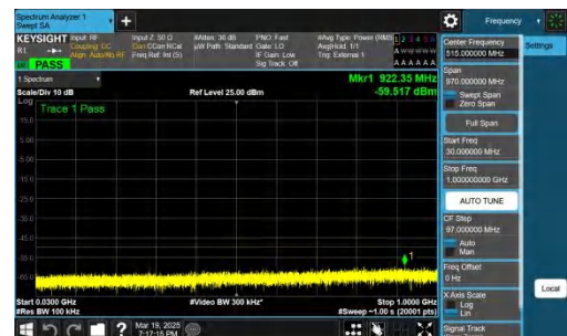
NTNV-n48-PC3-30-20-H-DFT-BPSK-Inner_1RB_Right-30-1000-PASS
