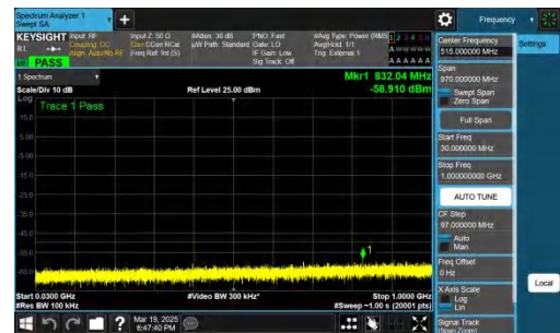
NTNV-n48-PC3-30-20-L-DFT-QPSK-Inner_1RB_Right-30-1000-P ASS
