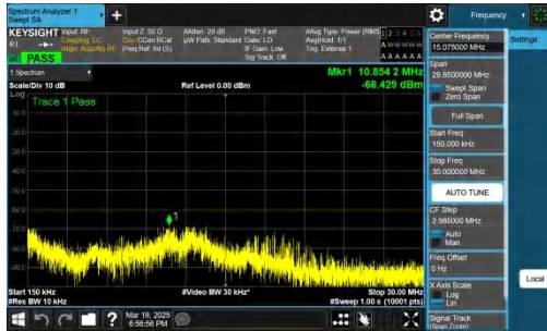
NTNV-n48-PC3-30-20-M-DFT-BPSK-Inner_1RB_Right-0.15-30-P ASS
