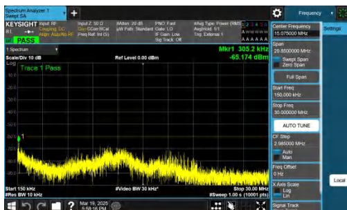
NTNV-n48-PC3-30-10-M-DFT-BPSK-Inner_1RB_Right-0.15-30-PASS
