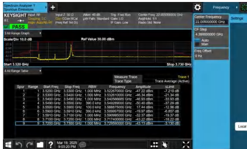
NTNV-n48-PC3-30-40-L-DFT-BPSK-Edge_1RB_Right-PASS
