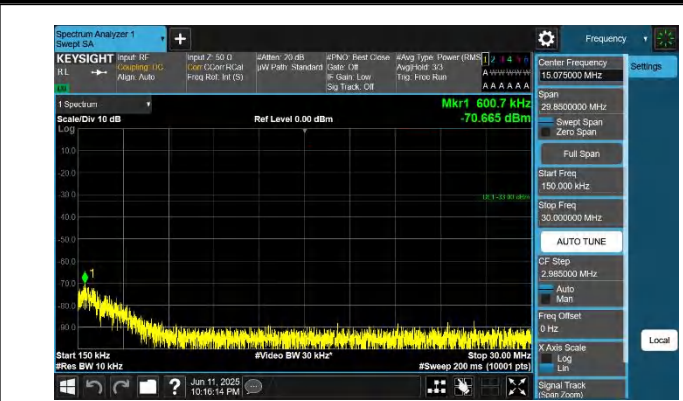
42-42-20MHz-15MHz-QPSK-QPSK-42516-42687-1RB#0-0RB#0- 0.15~30MHz-PASS
