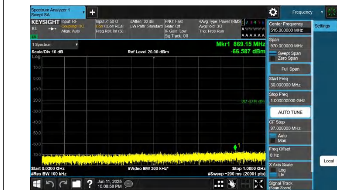
42-42-20MHz-20MHz-QPSK-QPSK-42190-42388-1RB#0-0RB#0- 30~1000MHz-PASS
