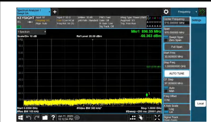
42-42-20MHz-5MHz-QPSK-QPSK-42940-43057-1RB#99-0RB#0- 30~1000MHz-PASS
