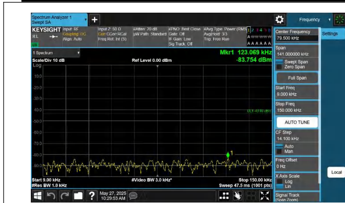
42-42-20MHz-10MHz-QPSK-QPSK-42190-42334-1RB#0-0RB#0- 0.009~0.15MHz-PASS
