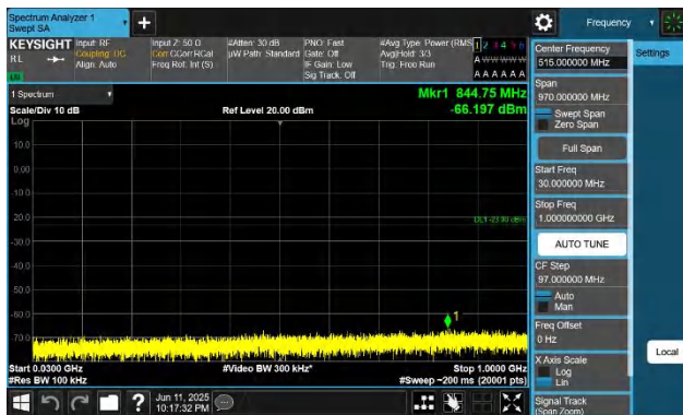
42-42-20MHz-15MHz-QPSK-QPSK-42841-43012-1RB#0-1RB#7 4-30~1000MHz-PASS
