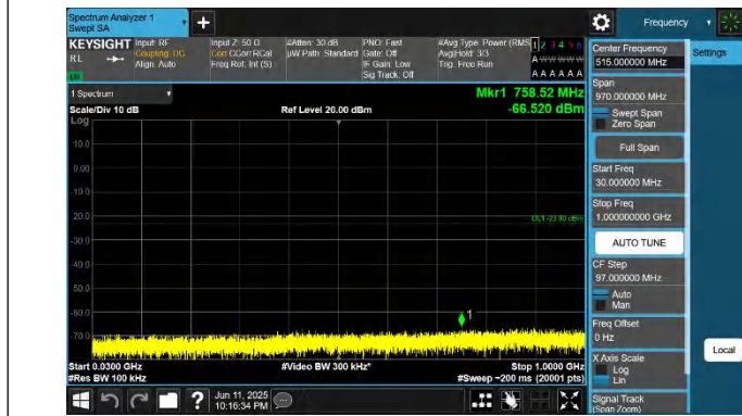
42-42-20MHz-15MHz-QPSK-QPSK-42516-42687-1RB#99-0RB# 0-30~1000MHz-PASS
