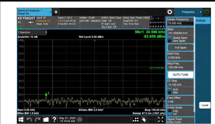
42-42-20MHz-20MHz-QPSK-QPSK-42190-42388-1RB#0-1RB#9 9-0.009~0.15MHz-PASS
