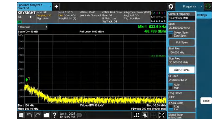
42-42-20MHz-15MHz-QPSK-QPSK-42190-42361-1RB#0-1RB#7 4-0.15~30MHz-PASS
