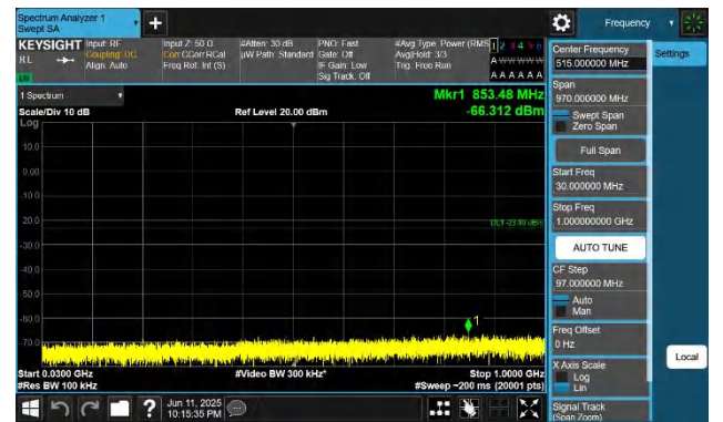
42-42-20MHz-15MHz-QPSK-QPSK-42190-42361-1RB#0-0RB#0- 30~1000MHz-PASS
