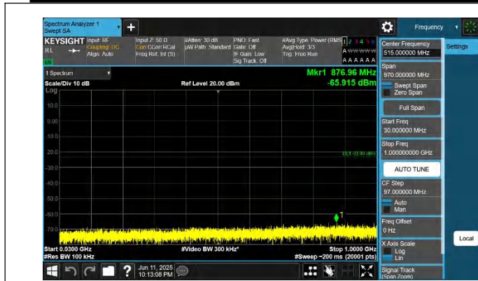
42-42-20MHz-5MHz-QPSK-QPSK-42940-43057-1RB#0-1RB#24- 30~1000MHz-PASS
