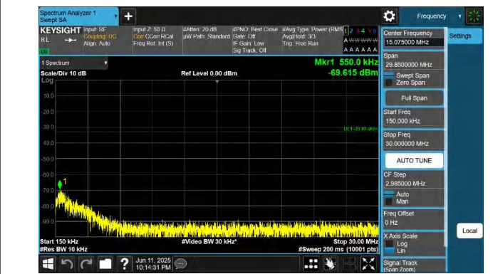
42-42-20MHz-10MHz-QPSK-QPSK-42541-42685-1RB#0-1RB#4 9-0.15~30MHz-PASS
