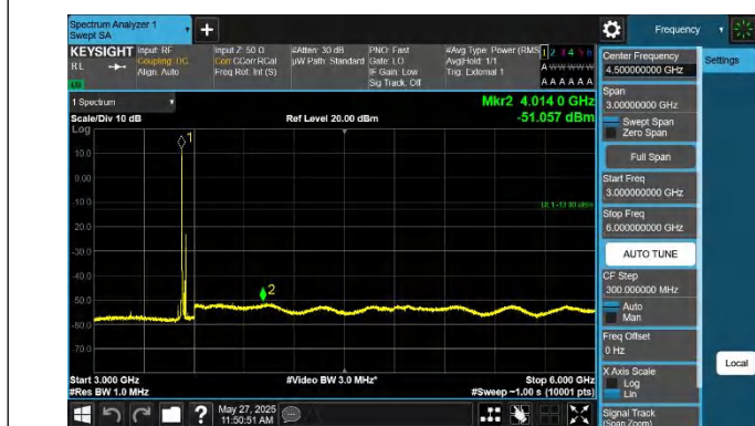
42-42-20MHz-5MHz-QPSK-QPSK-42940-43057-1RB#0-1RB#24- 3000~6000MHz-PASS
