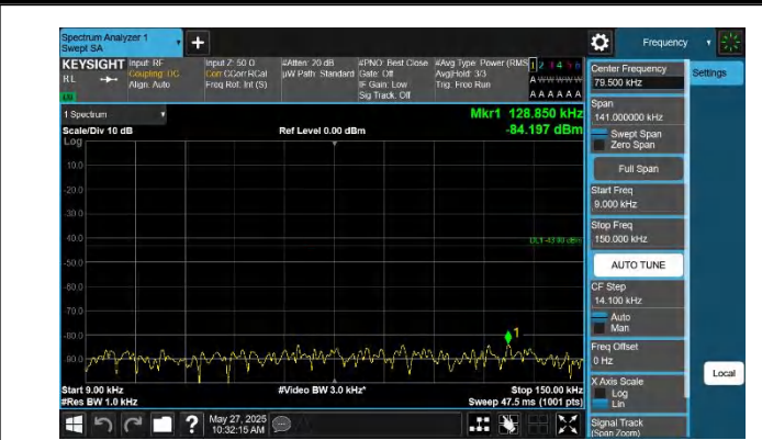
42-42-20MHz-10MHz-QPSK-QPSK-42190-42334-1RB#0-1RB#4 9-0.009~0.15MHz-PASS
