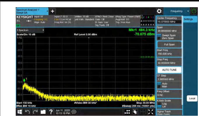
42-42-20MHz-10MHz-QPSK-QPSK-42190-42334-1RB#0-0RB#0- 0.15~30MHz-PASS
