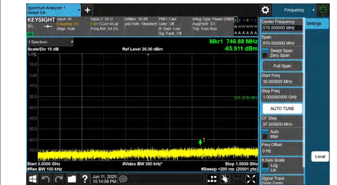
42-42-20MHz-10MHz-QPSK-QPSK-42541-42685-1RB#0-0RB#- 30~1000MHz-PASS
