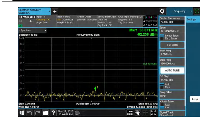
42-42-20MHz-15MHz-QPSK-QPSK-42516-42687-1RB#0-0RB#0- 0.009~0.15MHz-PASS
