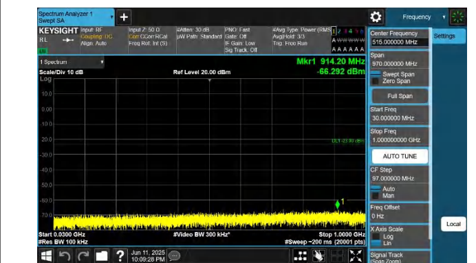
42-42-20MHz-20MHz-QPSK-QPSK-42190-42388-1RB#0-1RB#9 9-30~1000MHz-PASS
