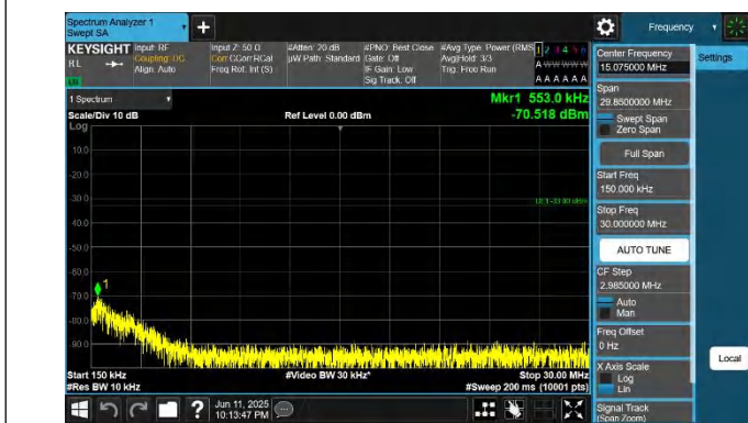
42-42-20MHz-10MHz-QPSK-QPSK-42190-42334-1RB#0-1RB#4 9-0.15~30MHz-PASS
