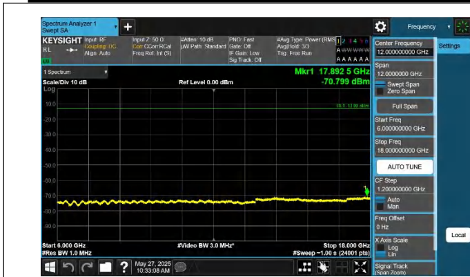
42-42-20MHz-10MHz-QPSK-QPSK-42190-42334-1RB#0-1RB#4 9-6000~18000MHz-PASS
