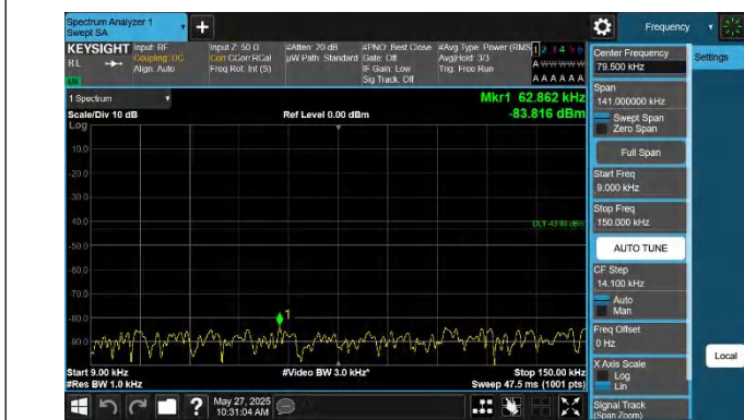
42-42-20MHz-10MHz-QPSK-QPSK-42190-42334-1RB#99-0RB# 0-0.009~0.15MHz-PASS
