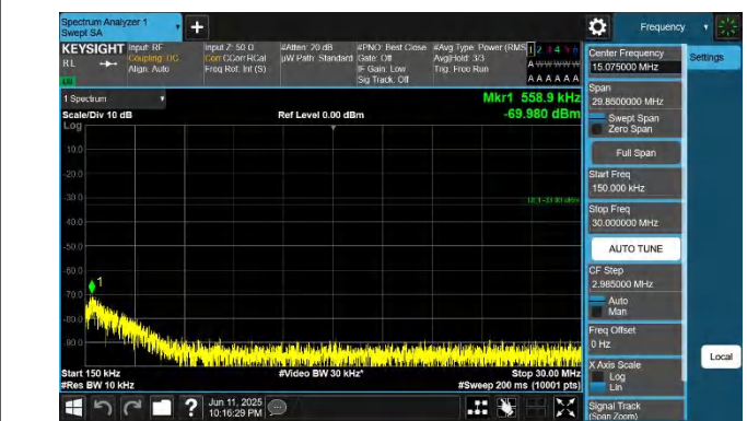
42-42-20MHz-15MHz-QPSK-QPSK-42516-42687-1RB#99-0RB# 0-0.15~30MHz-PASS
