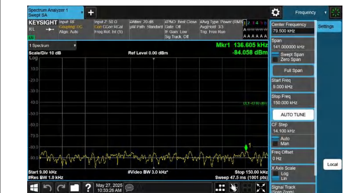
42-42-20MHz-10MHz-QPSK-QPSK-42541-42685-1RB#0-0RB#- 0.009~0.15MHz-PASS
