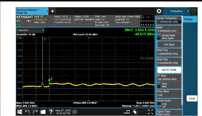
42-42-20MHz-15MHz-QPSK-QPSK-42190-42361-1RB#0-0RB#0- 3000~6000MHz-PASS
