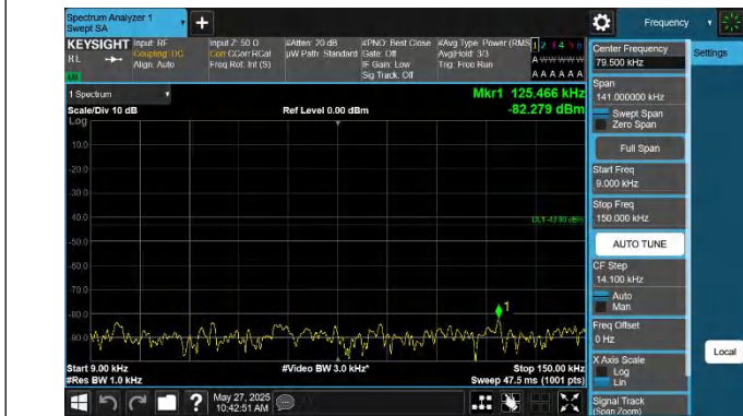
42-42-20MHz-15MHz-QPSK-QPSK-42190-42361-1RB#0-1RB#7 4-0.009~0.15MHz-PASS
