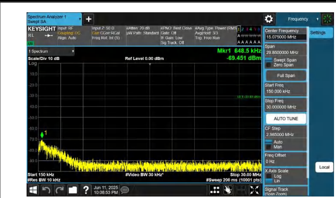
42-42-20MHz-20MHz-QPSK-QPSK-42190-42388-1RB#0-0RB#0- 0.15~30MHz-PASS
