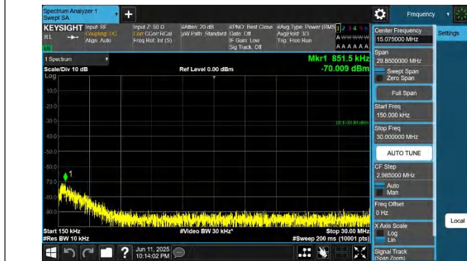
42-42-20MHz-10MHz-QPSK-QPSK-42541-42685-1RB#0-0RB#- 0.15~30MHz-PASS
