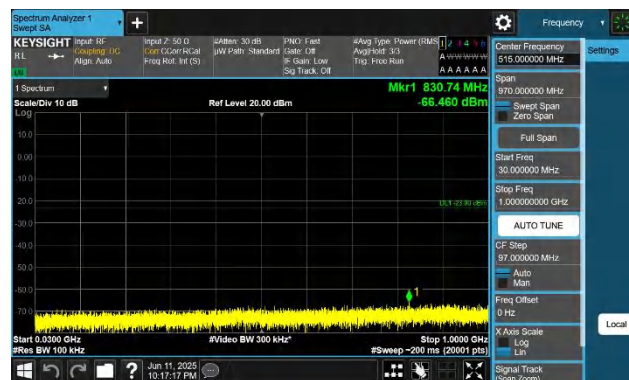
42-42-20MHz-15MHz-QPSK-QPSK-42841-43012-1RB#99-0RB# 0-30~1000MHz-PASS
