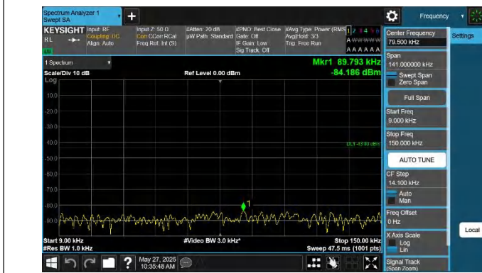
42-42-20MHz-10MHz-QPSK-QPSK-42541-42685-1RB#0-1RB#4 9-0.009~0.15MHz-PASS
