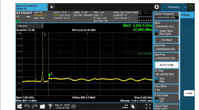
42-42-20MHz-15MHz-QPSK-QPSK-42190-42361-1RB#99-0RB# 0-3000~6000MHz-PASS
