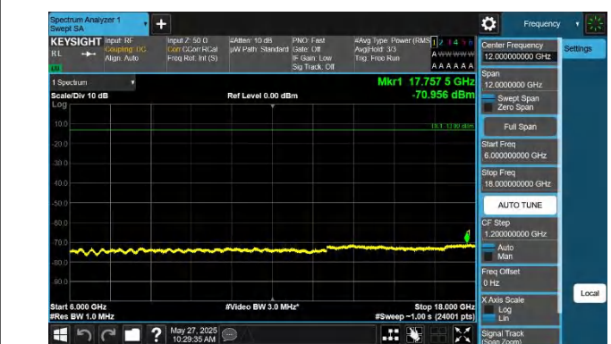
42-42-20MHz-5MHz-QPSK-QPSK-42940-43057-1RB#0-1RB#24- 6000~18000MHz-PASS
