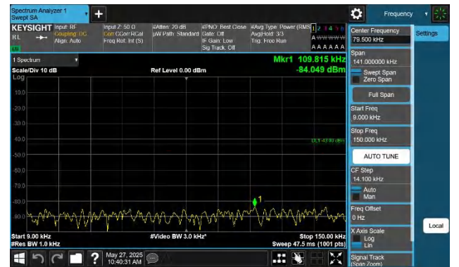
42-42-20MHz-15MHz-QPSK-QPSK-42190-42361-1RB#0-0RB#0- 0.009~0.15MHz-PASS
