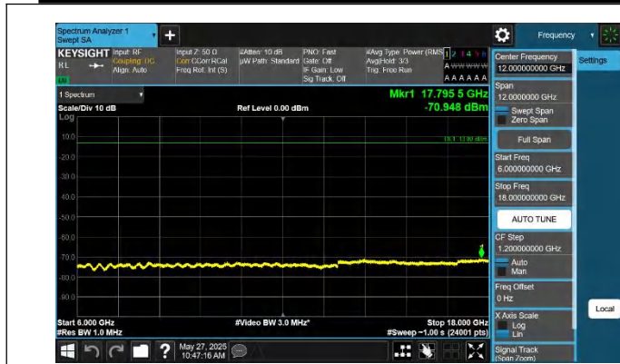
42-42-20MHz-15MHz-QPSK-QPSK-42516-42687-1RB#0-1RB#7 4-6000~18000MHz-PASS
