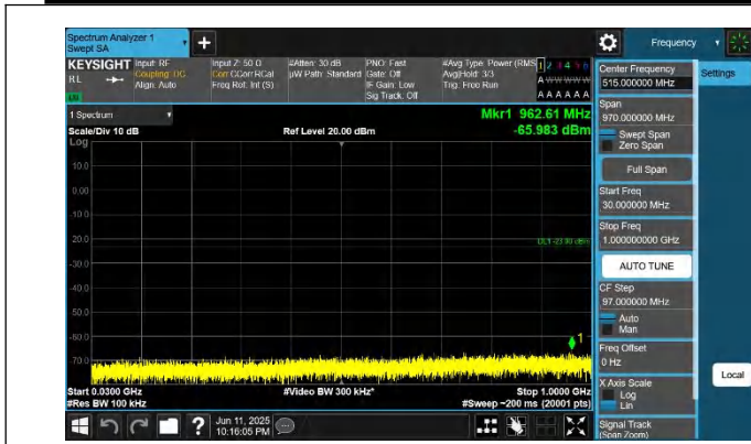
42-42-20MHz-15MHz-QPSK-QPSK-42190-42361-1RB#0-1RB#7 4-30~1000MHz-PASS
