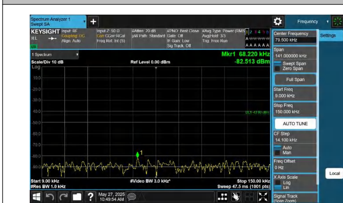
42-42-20MHz-15MHz-QPSK-QPSK-42841-43012-1RB#0-1RB#7 4-0.009~0.15MHz-PASS
