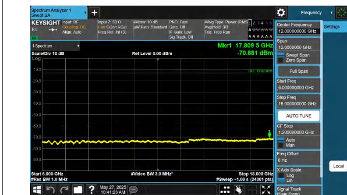
42-42-20MHz-15MHz-QPSK-QPSK-42190-42361-1RB#0-0RB#0- 6000~18000MHz-PASS
