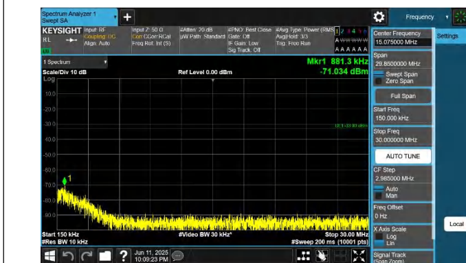
42-42-20MHz-20MHz-QPSK-QPSK-42190-42388-1RB#0-1RB#9 9-0.15~30MHz-PASS
