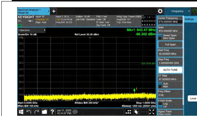
42-42-20MHz-10MHz-QPSK-QPSK-42541-42685-1RB#0-1RB#4 9-30~1000MHz-PASS
