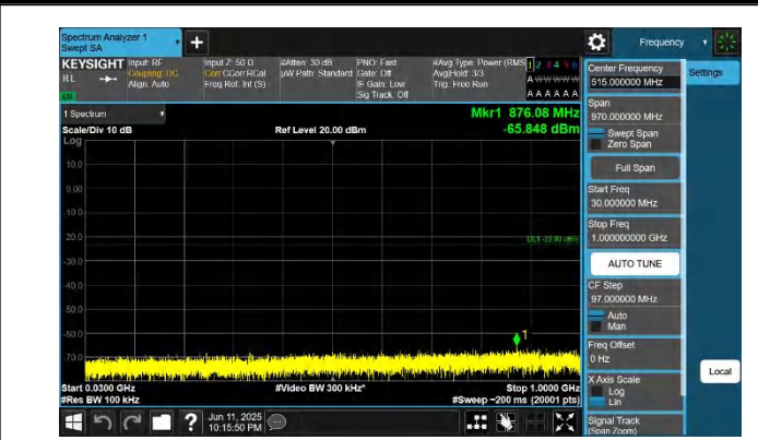
42-42-20MHz-15MHz-QPSK-QPSK-42190-42361-1RB#99-0RB# 0-30~1000MHz-PASS
