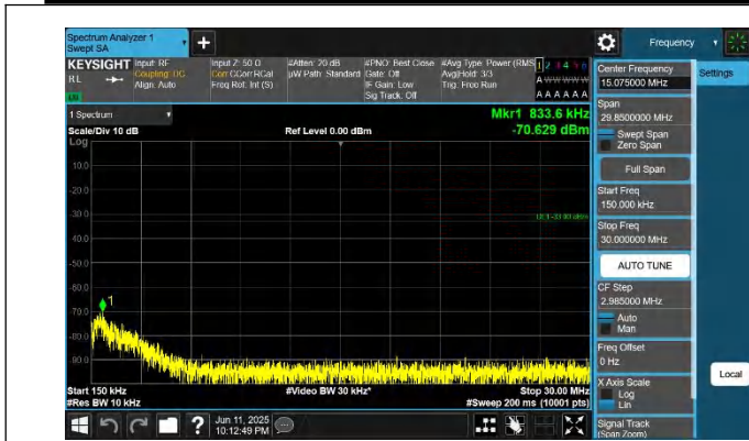
42-42-20MHz-5MHz-QPSK-QPSK-42940-43057-1RB#99-0RB#0- 0.15~30MHz-PASS
