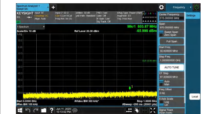
42-42-20MHz-10MHz-QPSK-QPSK-42190-42334-1RB#0-1RB#4 9-30~1000MHz-PASS
