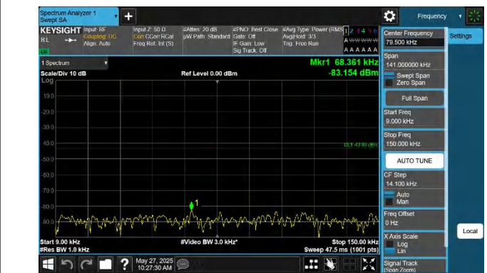
42-42-20MHz-5MHz-QPSK-QPSK-42940-43057-1RB#99-0RB#0- 0.009~0.15MHz-PASS
