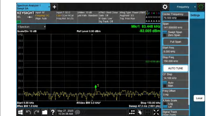
42-42-20MHz-10MHz-QPSK-QPSK-42541-42685-1RB#99-0RB# 0-0.009~0.15MHz-PASS
