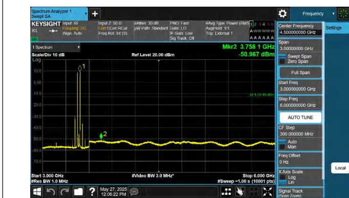
42-42-20MHz-15MHz-QPSK-QPSK-42190-42361-1RB#0-1RB#7 4-3000~6000MHz-PASS
