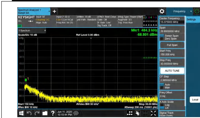
42-42-20MHz-15MHz-QPSK-QPSK-42190-42361-1RB#99-0RB# 0-0.15~30MHz-PASS
