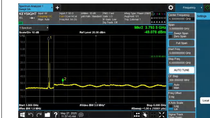
42-42-20MHz-10MHz-QPSK-QPSK-42541-42685-1RB#0-1RB#4 9-3000~6000MHz-PASS
