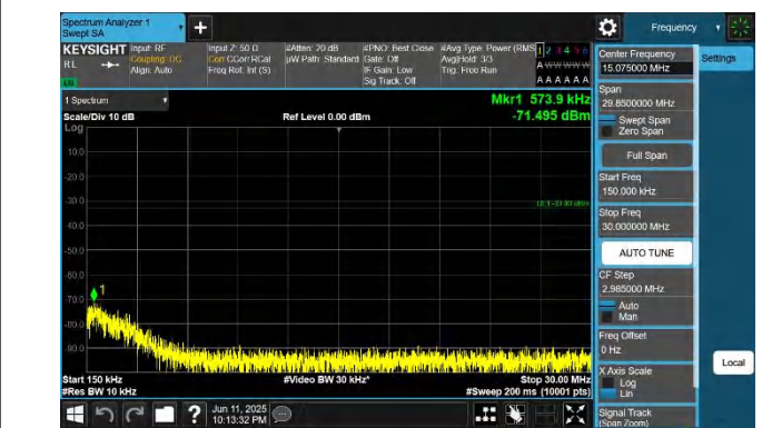
42-42-20MHz-10MHz-QPSK-QPSK-42190-42334-1RB#99-0RB# 0-0.15~30MHz-PASS
