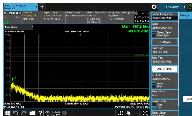
42-42-20MHz-5MHz-QPSK-QPSK-42940-43057-1RB#0-1RB#24- 0.15~30MHz-PASS
