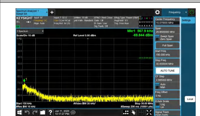
42-42-20MHz-15MHz-QPSK-QPSK-42841-43012-1RB#0-1RB#7 4-0.15~30MHz-PASS
