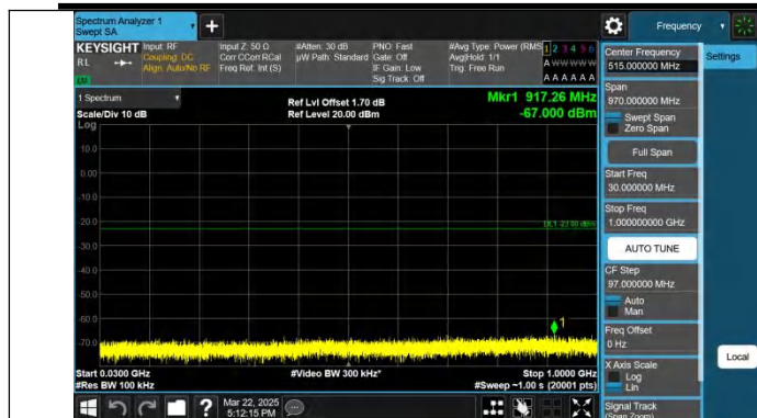
Band66-20MHz-QPSK-132072-1RB#0-30~1000-PASS
