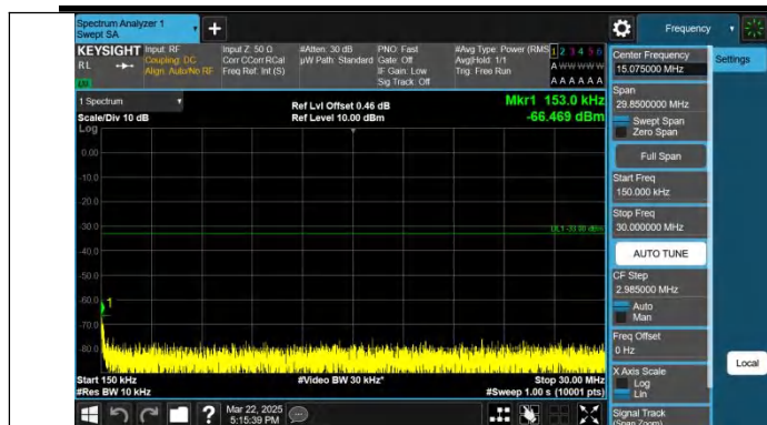
Band66-20MHz-QPSK-132572-1RB#99-0.15~30-PASS
