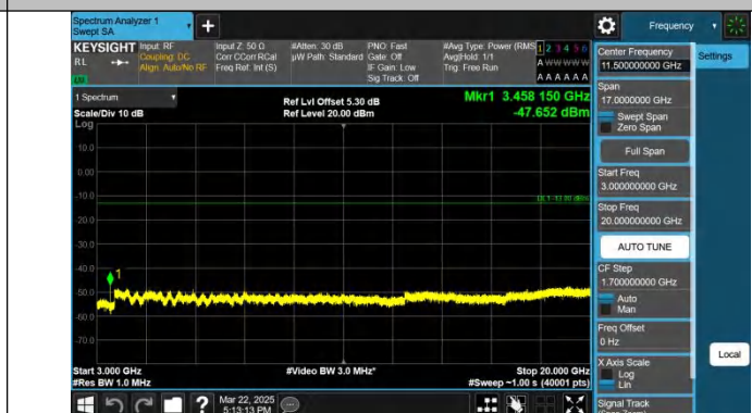
Band66-20MHz-QPSK-132072-1RB#99-3000~20000-PASS
