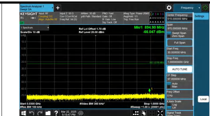
Band66-20MHz-QPSK-132572-1RB#99-30~1000-PASS
