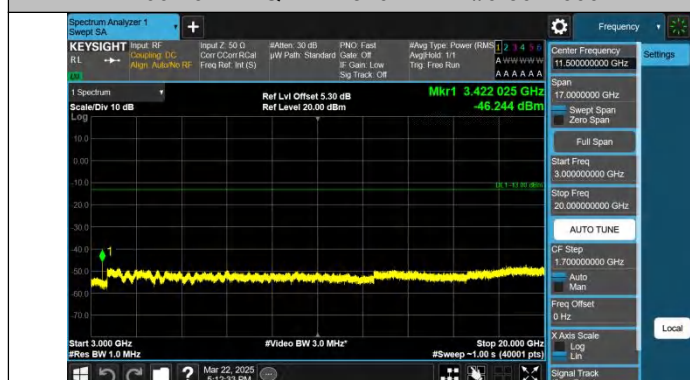
Band66-20MHz-QPSK-132072-1RB#0-3000~20000-PASS
