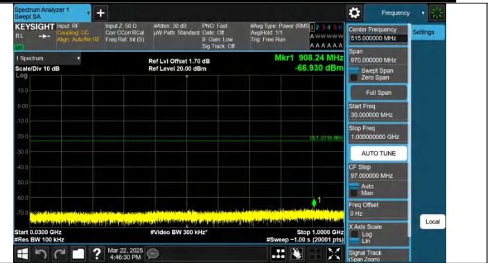
Band66-10MHz-QPSK-132022-1RB#49-30~1000-PASS
