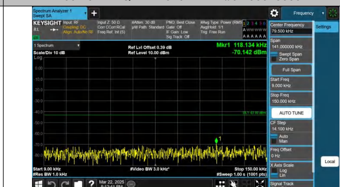
Band66-20MHz-QPSK-132072-1RB#99-0.009~0.15-PASS
