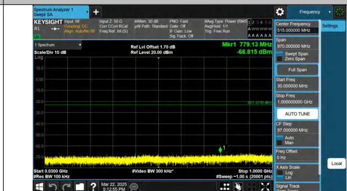
Band66-20MHz-QPSK-132072-1RB#99-30~1000-PASS
