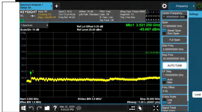
Band66-15MHz-QPSK-132597-1RB#0-3000~20000-PASS
