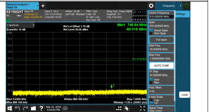
Band66-15MHz-QPSK-132597-1RB#74-30~1000-PASS
