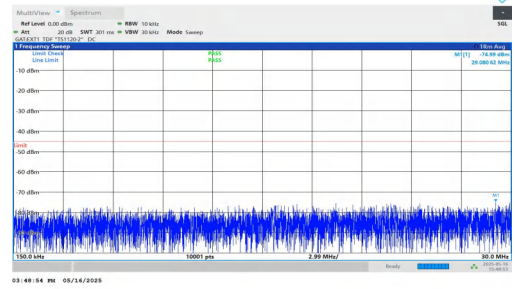
NTNV-DC_2A-n41A-PC2-30-5+50-M+M-QPSK-IDLE-DFT-BPSK-Inter_1RB_Left-0.15-30-PASS
