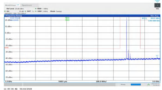
NTNV-DC_2A-n41A-PC2-30-5+50-M+M-QPSK-IDLE-DFT-QPSK-In ner_1RB_Left-1000-3000-PASS
