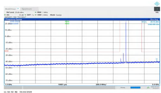
NTNV-DC_2A-n41A-PC2-30-5+70-M+L-QPSK-IDLE-DFT-QPSK-Inner_1RB_Right-1000-3000-PASS
