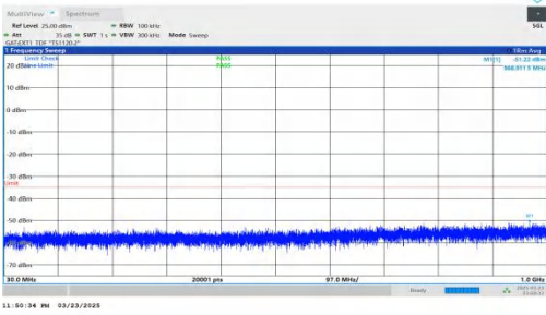
NTNV-DC_2A-n41A-PC2-30-5+70-M+L-QPSK-IDLE-DFT-BPSK-Inner_1RB_Right-30-1000-PASS
