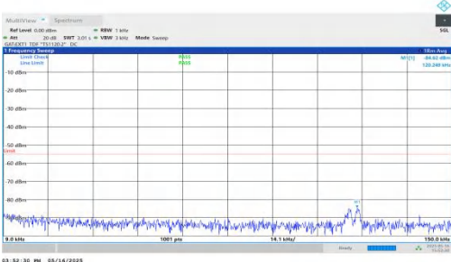
NTNV-DC_2A-n41A-PC2-30-5+50-M+H-QPSK-IDLE-DFT-QPSK-Inter_1RB_Right-0.009-0.15-PASS
