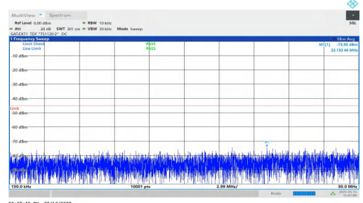
NTVN-DC_2A-n41A-PC2-30-5+50-M+L-QPSK-IDLE-DFT-QPSK-Inner_1RB_Left-0.15-30-PASS
