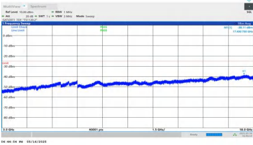
NTNV-DC_2A-n41A-PC2-30-5+60-M+L-QPSK-IDLE-DFT-QPSK-Inner_1RB_Left-3000-18000-PASS
