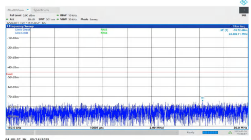
NTNV-DC_2A-n41A-PC2-30-5+70-M+L-QPSK-IDLE-DFT-BPSK-Inner_1RB_Right-0.15-30-PASS
