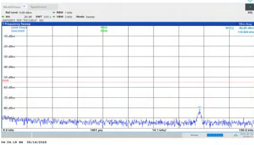
NTNV-DC_2A-n41A-PC2-30-5+70-M+H-QPSK-IDLE-DFT-BPSK-Inner_1RB_Right-0.009-0.15-PASS
