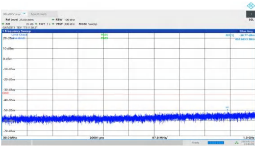
NTNV-DC_2A-n41A-PC2-30-5+60-M+M-QPSK-IDLE-DFT-QPSK-In ner_1RB_Left-30-1000-PASS
