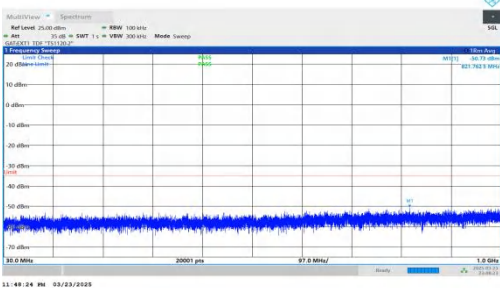
NTNV-DC_2A-n41A-PC2-30-5+60-M+H-QPSK-IDLE-DFT-QPSK-Inter_1RB_Right-30-1000-PASS
