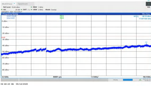
NTNV-DC_2A-n41A-PC2-30-5+60-M+M-QPSK-IDLE-DFT-QPSK-Inner_1RB_Left-3000-18000-PASS
