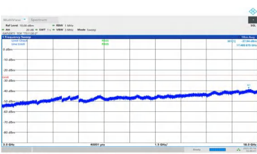
NTNV-DC_2A-n41A-PC2-30-5+70-M+L-QPSK-IDLE-DFT-QPSK-Inner_1RB_Right-3000-18000-PASS
