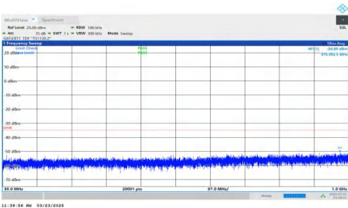
NTNV-DC_2A-n41A-PC2-30-5+60-M+L-QPSK-IDLE-DFT-QPSK-Inner_1RB_Right-30-1000-PASS
