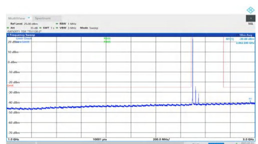
NTVN-DC_2A-n41A-PC2-30-5+50-M+L-QPSK-IDLE-DFT-QPSK-Inner_1RB_Left-1000-3000-PASS
