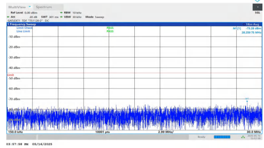
NTNV-DC_2A-n41A-PC2-30-5+60-M+H-QPSK-IDLE-DFT-BPSK-Inner_1RB_Right-0.15-30-PASS
