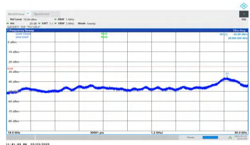
NTNV-DC_2A-n41A-PC2-30-5+60-M+M-QPSK-IDLE-DFT-BPSK-In ner_1RB_Left-18000-30000-PASS
