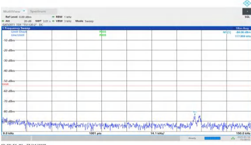
NTNV-DC_2A-n41A-PC2-30-5+60-M+H-QPSK-IDLE-DFT-QPSK-Inter_1RB_Right-0.009-0.15-PASS
