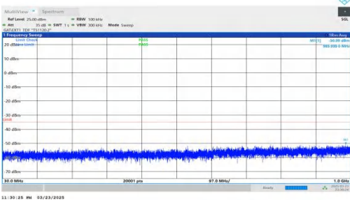
NTNV-DC_2A-n41A-PC2-30-5+50-M+M-QPSK-IDLE-DFT-QPSK-In ner_1RB_Left-30-1000-PASS
