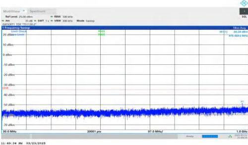
NTNV-DC_2A-n41A-PC2-30-5+70-M+L-QPSK-IDLE-DFT-BPSK-Inner_1RB_Left-30-1000-PASS
