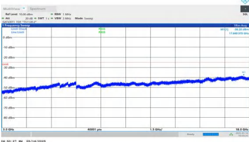
NTNV-DC_2A-n41A-PC2-30-5+70-M+M-QPSK-IDLE-DFT-BPSK-In ner_1RB_Right-3000-18000-PASS
