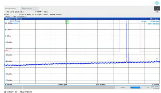
NTNV-DC_2A-n41A-PC2-30-5+50-M+M-QPSK-IDLE-DFT-BPSK-Inter_1RB_Left-1000-3000-PASS
