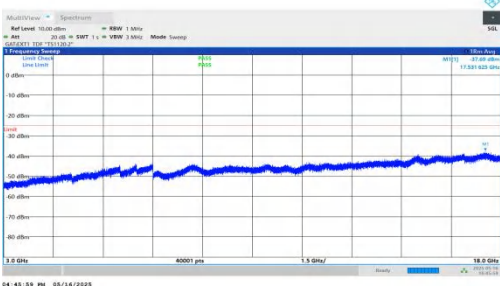
NTNV-DC_2A-n41A-PC2-30-5+60-M+M-QPSK-IDLE-DFT-BPSK-In ner_1RB_Right-3000-18000-PASS
