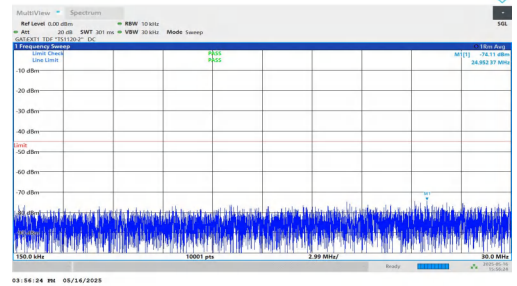
NTNV-DC_2A-n41A-PC2-30-5+60-M+M-QPSK-IDLE-DFT-QPSK-In ner_1RB_Left-0.15-30-PASS
