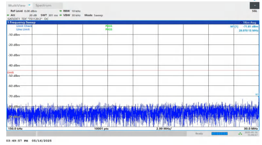
NTNV-DC_2A-n41A-PC2-30-5+50-M+M-QPSK-IDLE-DFT-QPSK-In ner_1RB_Left-0.15-30-PASS
