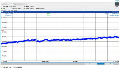
NTNV-DC_2A-n41A-PC2-30-5+50-M+M-QPSK-IDLE-DFT-QPSK-Inner_1RB_Right-3000-18000-PASS
