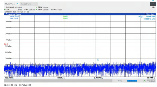
NTNV-DC_2A-n41A-PC2-30-5+70-M+H-QPSK-IDLE-DFT-BPSK-Inner_1RB_Left-0.15-30-PASS
