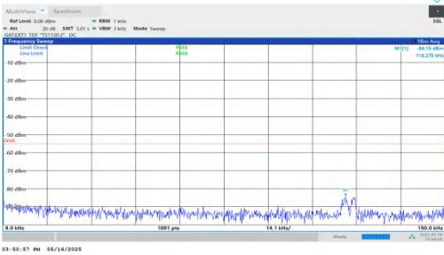
NTNV-DC_2A-n41A-PC2-30-5+50-M+H-QPSK-IDLE-DFT-BPSK-Inner_1RB_Left-0.009-0.15-PASS
