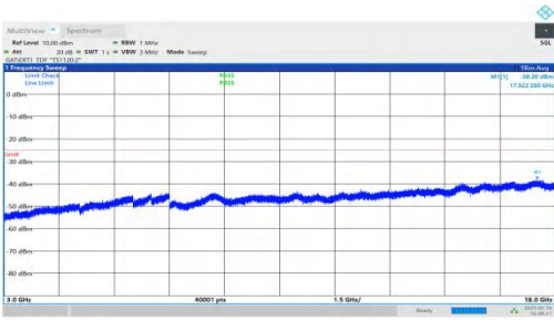
NTNV-DC_2A-n41A-PC2-30-5+60-M+H-QPSK-IDLE-DFT-QPSK-Inter_1RB_Right-3000-18000-PASS
