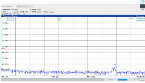
NTVN-DC_2A-n41A-PC2-30-5+60-M+L-QPSK-IDLE-DFT-QPSK-Inner_1RB_Left-0.009-0.15-PASS
