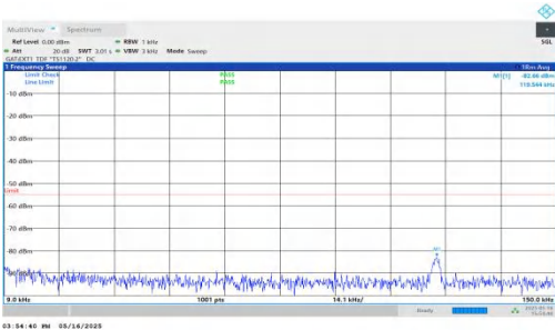
NTNV-DC_2A-n41A-PC2-30-5+60-M+L-QPSK-IDLE-DFT-QPSK-Inner_1RB_Right-0.009-0.15-PASS
