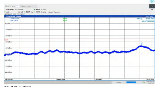
NTNV-DC_2A-n41A-PC2-30-5+70-M+H-QPSK-IDLE-DFT-QPSK-In ner_1RB_Right-18000-30000-PASS
