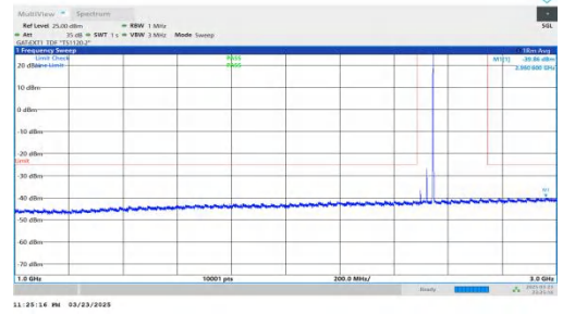
NTVN-DC_2A-n41A-PC2-30-5+50-M+L-QPSK-IDLE-DFT-BPSK-Inner_1RB_Right-1000-3000-PASS
