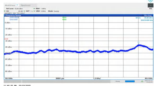
NTNV-DC_2A-n41A-PC2-30-5+60-M+M-QPSK-IDLE-DFT-BPSK-In ner_1RB_Right-18000-30000-PASS
