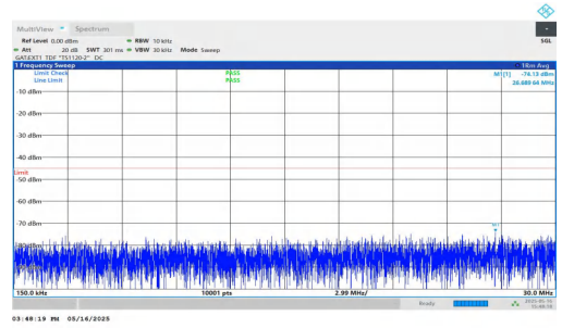
NTNV-DC_2A-n41A-PC2-30-5+50-M+L-QPSK-IDLE-DFT-QPSK-Inner_1RB_Right-0.15-30-PASS
