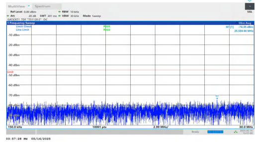
NTNV-DC_2A-n41A-PC2-30-5+60-M+H-QPSK-IDLE-DFT-BPSK-Inner_1RB_Left-0.15-30-PASS
