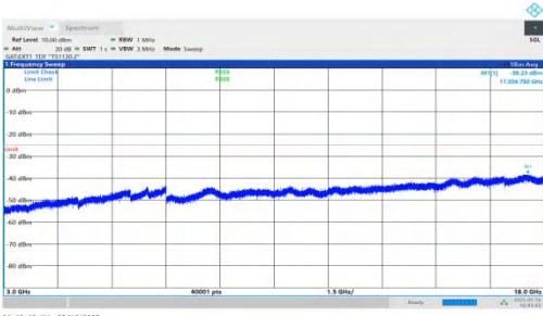
NTNV-DC_2A-n41A-PC2-30-5+50-M+H-QPSK-IDLE-DFT-QPSK-Inter_1RB_Right-3000-18000-PASS
