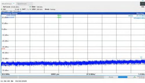
NTNV-DC_2A-n41A-PC2-30-5+70-M+M-QPSK-IDLE-DFT-BPSK-In ner_1RB_Right-30-1000-PASS
