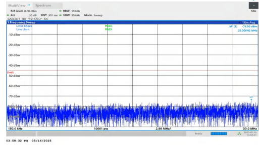
NTNV-DC_2A-n41A-PC2-30-5+60-M+H-QPSK-IDLE-DFT-QPSK-Inner_1RB_Left-0.15-30-PASS
