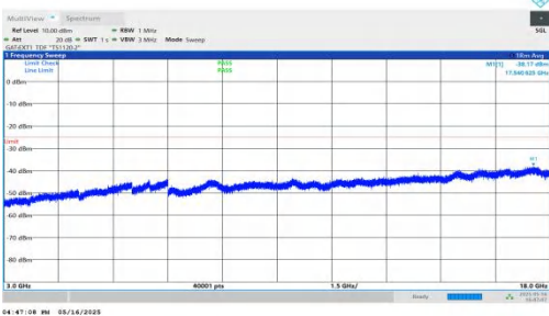
NTNV-DC_2A-n41A-PC2-30-5+60-M+H-QPSK-IDLE-DFT-BPSK-Inner_1RB_Left-3000-18000-PASS
