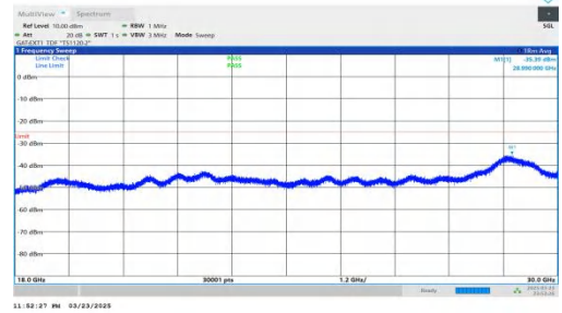
NTNV-DC_2A-n41A-PC2-30-5+70-M+L-QPSK-IDLE-DFT-QPSK-Inner_1RB_Left-18000-30000-PASS
