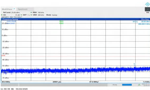
NTNV-DC_2A-n41A-PC2-30-5+70-M+M-QPSK-IDLE-DFT-QPSK-Inner_1RB_Right-30-1000-PASS
