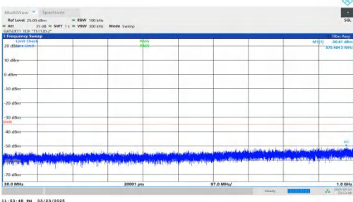
NTNV-DC_2A-n41A-PC2-30-5+70-M+M-QPSK-IDLE-DFT-BPSK-In ner_1RB_Left-30-1000-PASS
