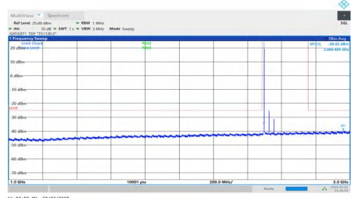
NTNV-DC_2A-n41A-PC2-30-5+60-M+L-QPSK-IDLE-DFT-BPSK-Inner_1RB_Left-1000-3000-PASS
