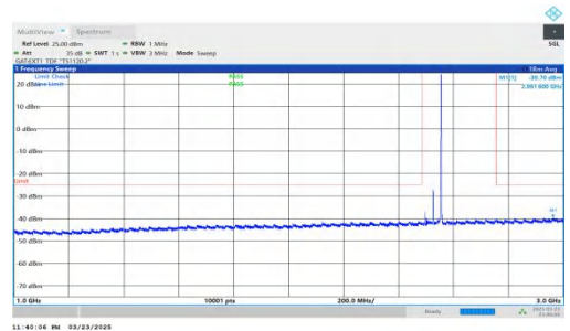
NTNV-DC_2A-n41A-PC2-30-5+60-M+L-QPSK-IDLE-DFT-QPSK-Inner_1RB_Right-1000-3000-PASS
