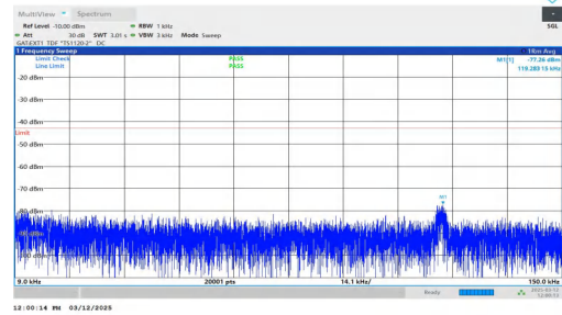
NTNV-n77(3700-3980)-PC2-30-80-M-DFT-QPSK-Inner_1RB_Righ t-0.009-0.15-PASS
