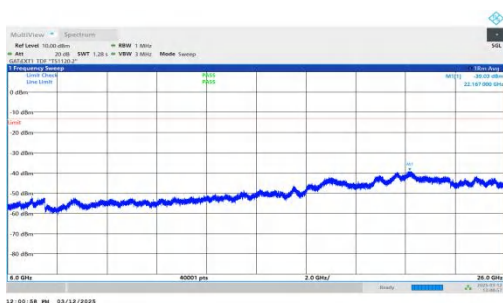
NTNV-n77(3700-3980)-PC2-30-80-M-DFT-QPSK-Inner_1RB_Rig ht-6000-26000-PASS
