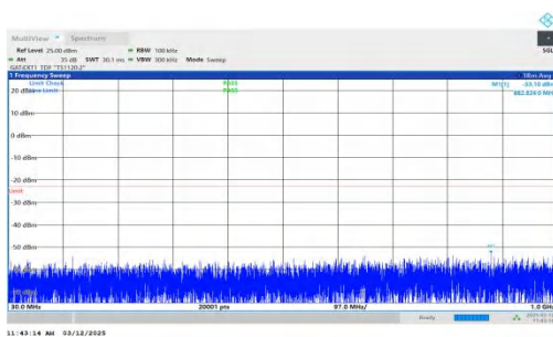
NTNV-n77(3700-3980)-PC2-30-60-H-DFT-BPSK-Inner_1RB_Left -30-1000-PASS
