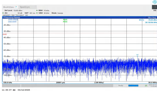
NTNV-n77(3700-3980)-PC2-30-60-L-DFT-QPSK-Inner_1RB_Rig ht-0.15-30-PASS
