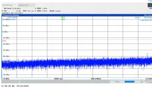
NTNV-n77(3700-3980)-PC2-30-60-H-DFT-BPSK-Inner_1RB_Rig ht-1000-3000-PASS
