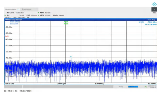
NTNV-n77(3700-3980)-PC2-30-100-L-DFT-BPSK-Inner_1RB_Left -0.15-30-PASS
