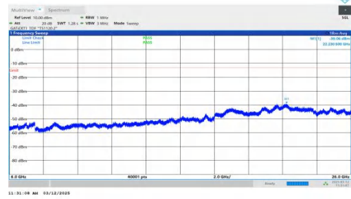
NTNV-n77(3700-3980)-PC2-30-60-L-DFT-BPSK-Inner_1RB_Left-6000-26000-PASS
