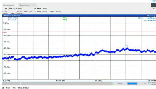
NTNV-n77(3700-3980)-PC2-30-60-L-DFT-QPSK-Inner_1RB_Rig ht-6000-26000-PASS
