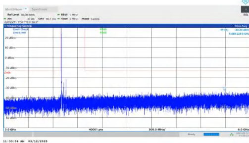
NTNV-n77(3700-3980)-PC2-30-60-L-DFT-QPSK-Inner_1RB_Left -3000-6000-PASS
