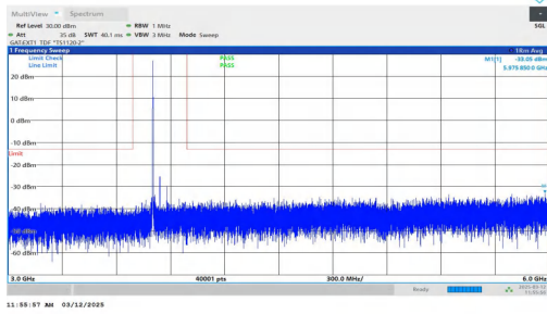
NTNV-n77(3700-3980)-PC2-30-80-M-DFT-BPSK-Inner_1RB_Left -3000-6000-PASS
