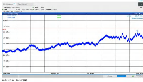
NTNV-n77(3700-3980)-PC2-30-60-L-DFT-QPSK-Inner_1RB_Left -26000-40000-PASS
