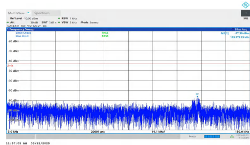
NTNV-n77(3700-3980)-PC2-30-80-M-DFT-BPSK-Inner_1RB_Right t-0.009-0.15-PASS
