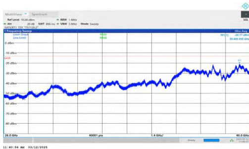
NTNV-n77(3700-3980)-PC2-30-60-M-DFT-QPSK-Inner_1RB_Lef t-26000-40000-PASS
