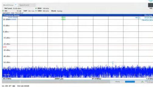
NTNV-n77(3700-3980)-PC2-30-80-M-DFT-BPSK-Inner_1RB_Left -30-1000-PASS
