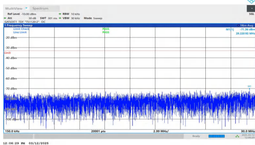
NTNV-n77(3700-3980)-PC2-30-80-H-DFT-QPSK-Inner_1RB_Rig ht-0.15-30-PASS
