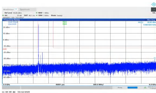
NTNV-n77(3700-3980)-PC2-30-80-L-DFT-BPSK-Inner_1RB_Left- 3000-6000-PASS
