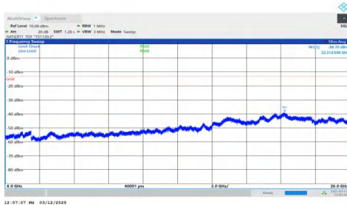
NTNV-n77(3700-3980)-PC2-30-80-H-DFT-QPSK-Inner_1RB_Rig ht-6000-26000-PASS
