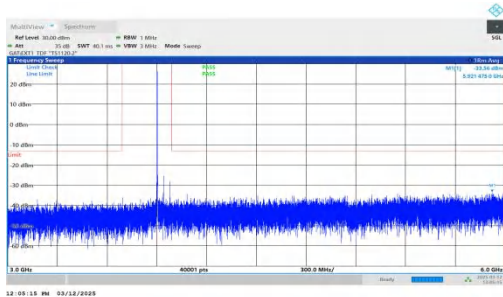
NTNV-n77(3700-3980)-PC2-30-80-H-DFT-QPSK-Inner_1RB_Left -3000-6000-PASS
