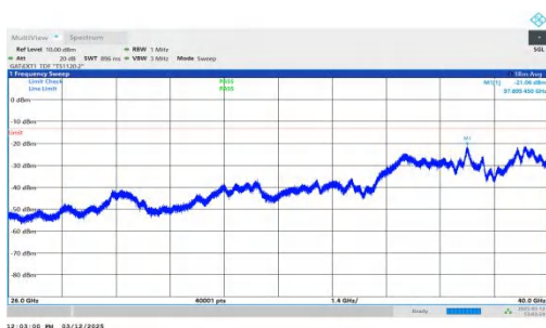
NTNV-n77(3700-3980)-PC2-30-80-H-DFT-BPSK-Inner_1RB_Left -26000-40000-PASS
