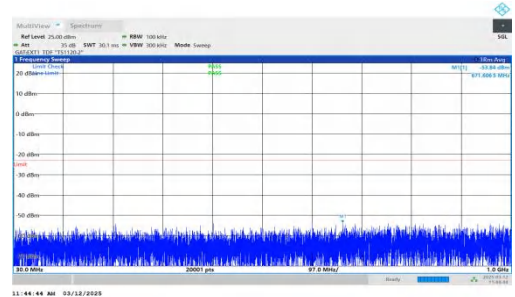
NTNV-n77(3700-3980)-PC2-30-60-H-DFT-BPSK-Inner_1RB_Right t-30-1000-PASS
