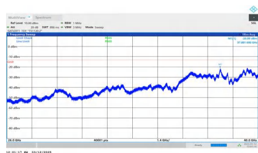
NTNV-n77(3700-3980)-PC2-30-80-M-DFT-QPSK-Inner_1RB_Righ t-26000-40000-PASS
