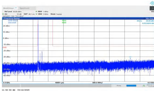
NTNV-n77(3700-3980)-PC2-30-80-L-DFT-QPSK-Inner_1RB_Left -3000-6000-PASS
