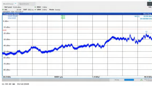
NTNV-n77(3700-3980)-PC2-30-80-M-DFT-QPSK-Inner_1RB_Lef t-26000-40000-PASS
