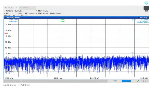
NTNV-n77(3700-3980)-PC2-30-60-H-DFT-QPSK-Inner_1RB_Left- 0.15-30-PASS
