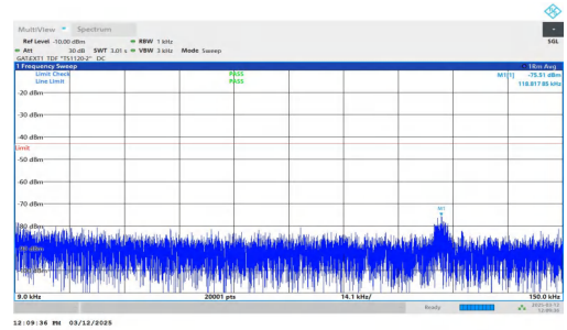
NTNV-n77(3700-3980)-PC2-30-100-L-DFT-BPSK-Inner_1RB_Rig ht-0.009-0.15-PASS
