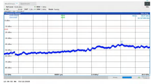
NTNV-n77(3700-3980)-PC2-30-100-L-DFT-BPSK-Inner_1RB_Left -6000-26000-PASS
