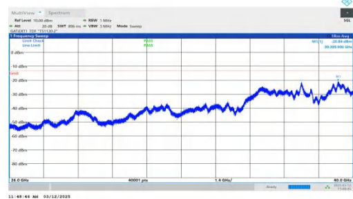
NTNV-n77(3700-3980)-PC2-30-60-H-DFT-QPSK-Inner_1RB_Right t.26000-40000-PASS
