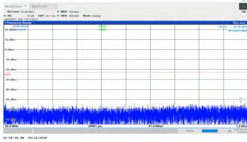
NTNV-n77(3700-3980)-PC2-30-80-H-DFT-QPSK-Inner_1RB_Left -30-1000-PASS
