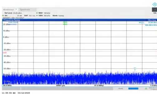
NTNV-n77(3700-3980)-PC2-30-80-M-DFT-QPSK-Inner_1RB_Lef t-30-1000-PASS
