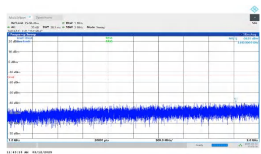
NTNV-n77(3700-3980)-PC2-30-60-H-DFT-BPSK-Inner_1RB_Left- 1000-3000-PASS
