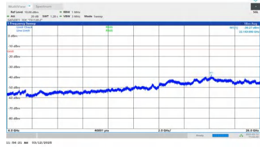
NTNV-n77(3700-3980)-PC2-30-80-M-DFT-BPSK-Inner_1RB_Left 6000-26000-PASS
