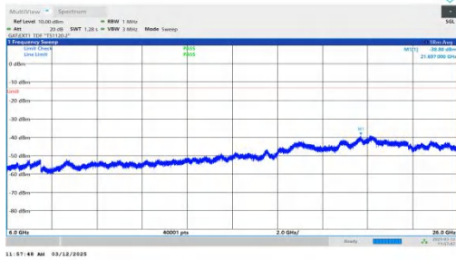
NTNV-n77(3700-3980)-PC2-30-80-M-DFT-BPSK-Inner_1RB_Rig ht-6000-26000-PASS
