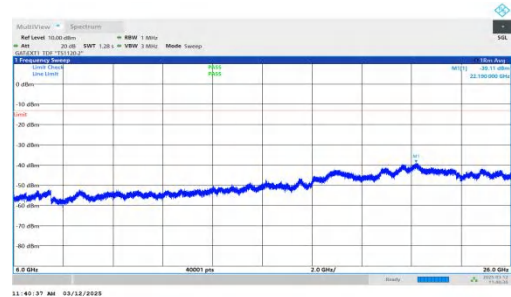
NTNV-n77(3700-3980)-PC2-30-60-M-DFT-QPSK-Inner_1RB_Left- 6000-26000-PASS
