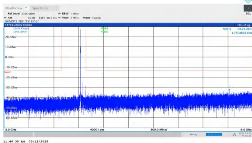
NTNV-n77(3700-3980)-PC2-30-60-H-DFT-QPSK-Inner_1RB_Left -3000-6000-PASS
