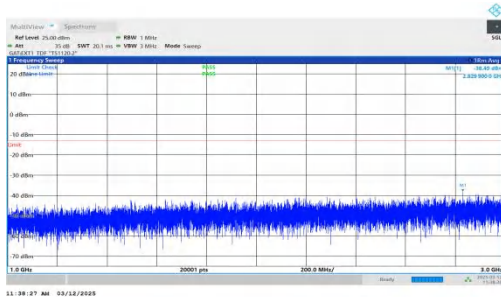
NTNV-n77(3700-3980)-PC2-30-60-M-DFT-BPSK-Inner_1RB_Rig ht-1000-3000-PASS
