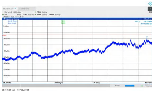
NTNV-n77(3700-3980)-PC2-30-80-L-DFT-QPSK-Inner_1RB_Left -26000-40000-PASS
