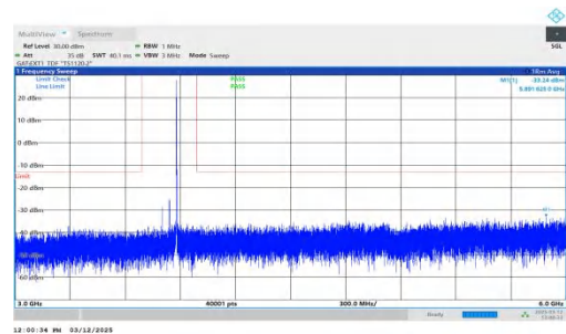
NTNV-n77(3700-3980)-PC2-30-80-M-DFT-QPSK-Inner_1RB_Righ t-3000-6000-PASS
