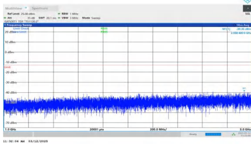
NTNV-n77(3700-3980)-PC2-30-60-L-DFT-BPSK-Inner_1RB_Rig ht-1000-3000-PASS
