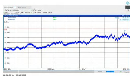
NTNV-n77(3700-3980)-PC2-30-80-L-DFT-BPSK-Inner_1RB_Right -26000-40000-PASS
