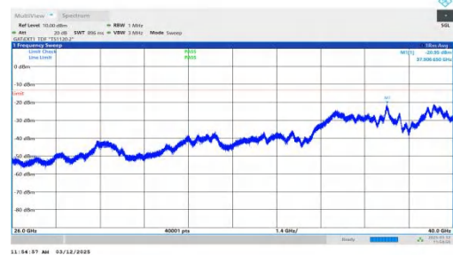
NTNV-n77(3700-3980)-PC2-30-80-L-DFT-QPSK-Inner_1RB_Right -26000-40000-PASS
