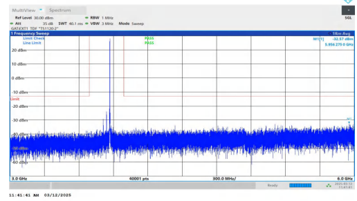
NTNV-n77(3700-3980)-PC2-30-60-M-DFT-QPSK-Inner_1RB_Righ t-3000-6000-PASS
