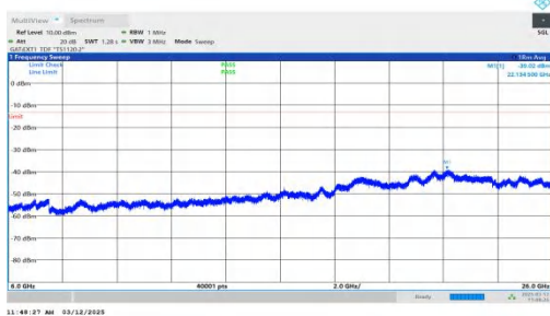
NTNV-n77(3700-3980)-PC2-30-60-H-DFT-QPSK-Inner_1RB_Right ht.6000-26000-PASS
