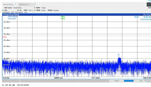
NTNV-n77(3700-3980)-PC2-30-60-M-DFT-BPSK-Inner_1RB_Left -0.009-0.15-PASS
