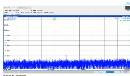
NTNV-n77(3700-3980)-PC2-30-80-M-DFT-BPSK-Inner_1RB_Right t-30-1000-PASS
