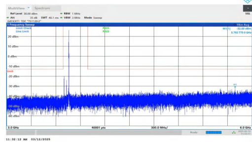
NTNV-n77(3700-3980)-PC2-30-60-L-DFT-BPSK-Inner_1RB_Right-3000-6000-PASS
