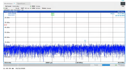
NTNV-n77(3700-3980)-PC2-30-80-L-DFT-BPSK-Inner_1RB_Left- 0.15-30-PASS
