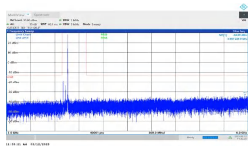
NTNV-n77(3700-3980)-PC2-30-60-L-DFT-QPSK-Inner_1RB_Right -3000-6000-PASS
