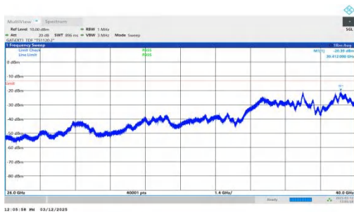
NTNV-n77(3700-3980)-PC2-30-80-H-DFT-QPSK-Inner_1RB_Left -26000-40000-PASS
