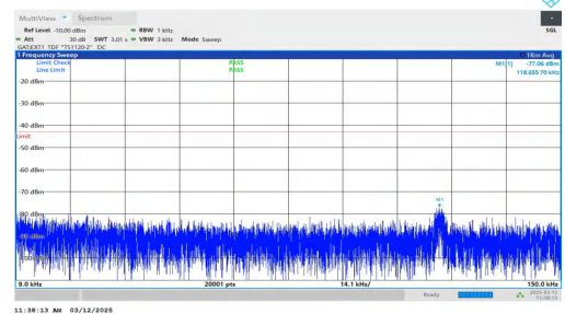
NTNV-n77(3700-3980)-PC2-30-60-M-DFT-BPSK-Inner_1RB_Right t-0.009-0.15-PASS
