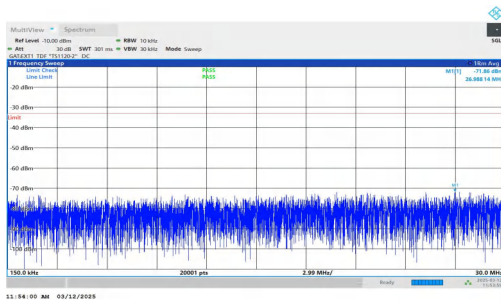
NTNV-n77(3700-3980)-PC2-30-80-L-DFT-QPSK-Inner_1RB_Rig ht-0.15-30-PASS
