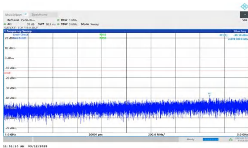
NTNV-n77(3700-3980)-PC2-30-80-L-DFT-BPSK-Inner_1RB_Rig ht-1000-3000-PASS
