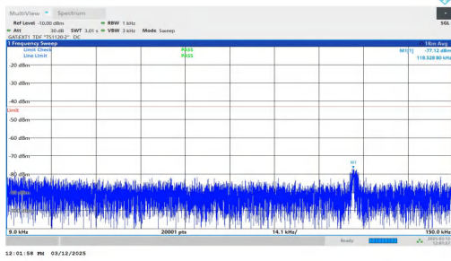
NTNV-n77(3700-3980)-PC2-30-80-H-DFT-BPSK-Inner_1RB_Left -0.009-0.15-PASS
