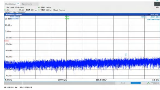
NTNV-n77(3700-3980)-PC2-30-80-H-DFT-QPSK-Inner_1RB_Left 1000-3000-PASS
