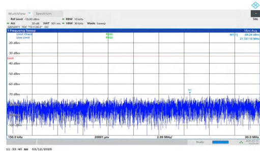
NTNV-n77(3700-3980)-PC2-30-60-L-DFT-QPSK-Inner_1RB_Left- 0.15-30-PASS
