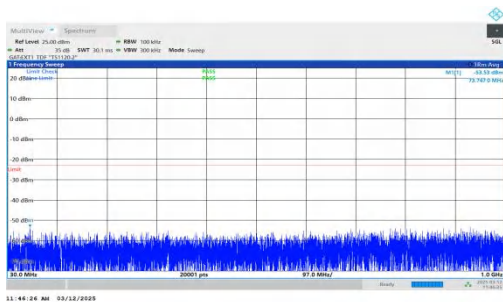
NTNV-n77(3700-3980)-PC2-30-60-H-DFT-QPSK-Inner_1RB_Left -30-1000-PASS
