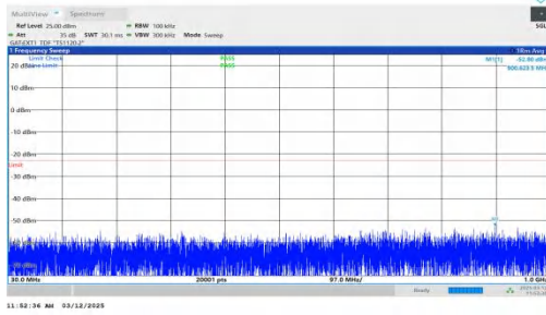
NTNV-n77(3700-3980)-PC2-30-80-L-DFT-QPSK-Inner_1RB_Left -30-1000-PASS
