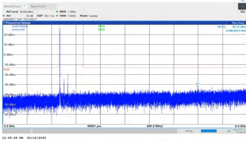
NTNV-n77(3700-3980)-PC2-30-100-L-DFT-BPSK-Inner_1RB_Lef t-3000-6000-PASS
