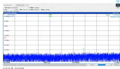
NTNV-n77(3700-3980)-PC2-30-60-L-DFT-BPSK-Inner_1RB_Right-30-1000-PASS
