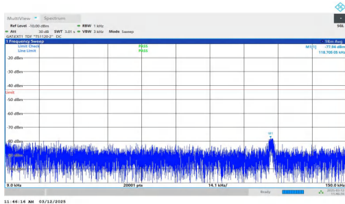
NTNV-n77(3700-3980)-PC2-30-60-H-DFT-QPSK-Inner_1RB_Left -0.009-0.15-PASS
