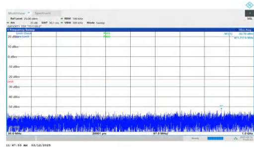
NTNV-n77(3700-3980)-PC2-30-60-H-DFT-QPSK-Inner_1RB_Right t.30-1000-PASS
