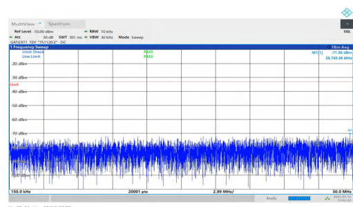
NTNV-n77(3700-3980)-PC2-30-80-L-DFT-QPSK-Inner_1RB_Left- 0.15-30-PASS
