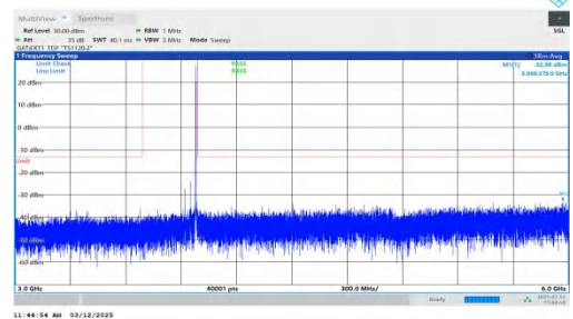
NTNV-n77(3700-3980)-PC2-30-60-H-DFT-BPSK-Inner_1RB_Right t-3000-6000-PASS
