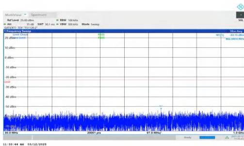
NTNV-n77(3700-3980)-PC2-30-60-L-DFT-QPSK-Inner_1RB_Left -30-1000-PASS
