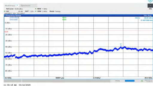
NTNV-n77(3700-3980)-PC2-30-60-L-DFT-QPSK-Inner_1RB_Left- 6000-26000-PASS
