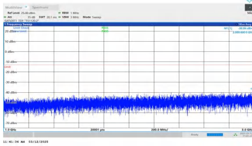
NTNV-n77(3700-3980)-PC2-30-60-M-DFT-QPSK-Inner_1RB_Rig ht-1000-3000-PASS
