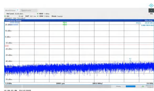
NTNV-n77(3700-3980)-PC2-30-100-L-DFT-BPSK-Inner_1RB_Left -1000-3000-PASS
