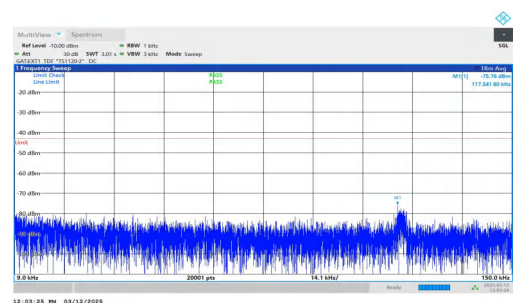
NTNV-n77(3700-3980)-PC2-30-80-H-DFT-BPSK-Inner_1RB_Right t-0.009-0.15-PASS
