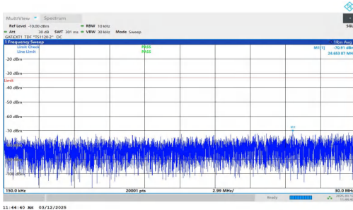
NTNV-n77(3700-3980)-PC2-30-60-H-DFT-BPSK-Inner_1RB_Rig ht-0.15-30-PASS
