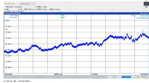
NTNV-n77(3700-3980)-PC2-30-60-H-DFT-BPSK-Inner_1RB_Righ t-26000-40000-PASS
