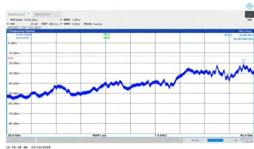
NTNV-n77(3700-3980)-PC2-30-80-H-DFT-BPSK-Inner_1RB_Righ t-26000-40000-PASS
