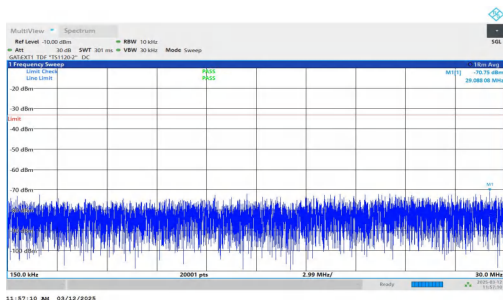
NTNV-n77(3700-3980)-PC2-30-80-M-DFT-BPSK-Inner_1RB_Right ht-0.15-30-PASS
