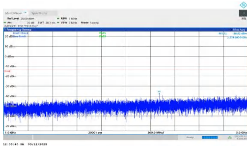
NTNV-n77(3700-3980)-PC2-30-80-H-DFT-BPSK-Inner_1RB_Rig ht-1000-3000-PASS
