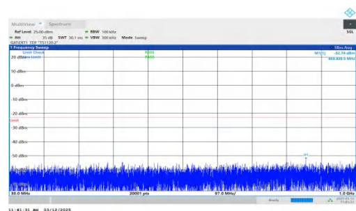
NTNV-n77(3700-3980)-PC2-30-60-M-DFT-QPSK-Inner_1RB_Right t-30-1000-PASS
