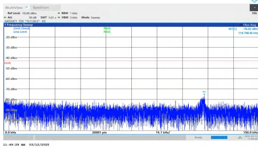
NTNV-n77(3700-3980)-PC2-30-80-L-DFT-BPSK-Inner_1RB_Left- 0.009-0.15-PASS
