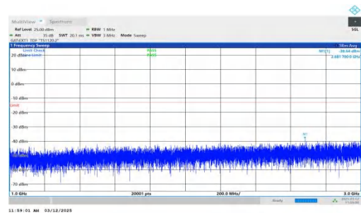
NTNV-n77(3700-3980)-PC2-30-80-M-DFT-QPSK-Inner_1RB_Left- 1000-3000-PASS
