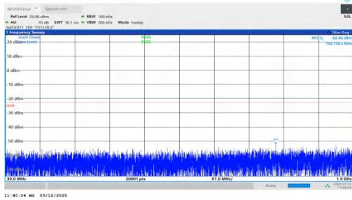
NTNV-n77(3700-3980)-PC2-30-60-M-DFT-QPSK-Inner_1RB_Lef t-30-1000-PASS
