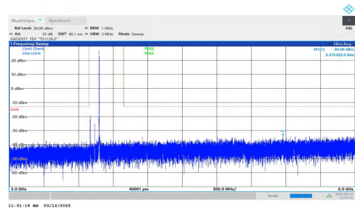
NTNV-n77(3700-3980)-PC2-30-80-L-DFT-BPSK-Inner_1RB_Right -3000-6000-PASS
