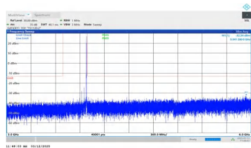
NTNV-n77(3700-3980)-PC2-30-60-H-DFT-QPSK-Inner_1RB_Right t.3000-6000-PASS
