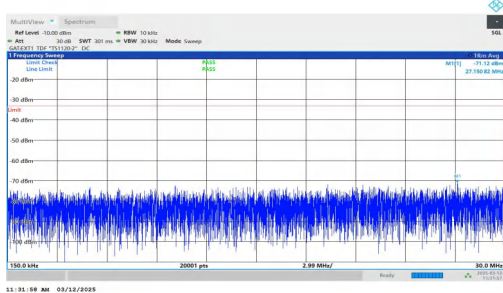
NTNV-n77(3700-3980)-PC2-30-60-L-DFT-BPSK-Inner_1RB_Rig ht-0.15-30-PASS
