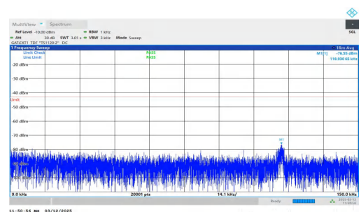
NTNV-n77(3700-3980)-PC2-30-80-L-DFT-BPSK-Inner_1RB_Right -0.009-0.15-PASS
