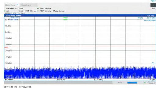
NTNV-n77(3700-3980)-PC2-30-80-H-DFT-QPSK-Inner_1RB_Right t-30-1000-PASS
