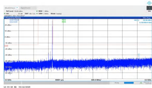
NTNV-n77(3700-3980)-PC2-30-80-H-DFT-BPSK-Inner_1RB_Righ t-3000-6000-PASS
