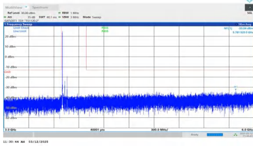
NTNV-n77(3700-3980)-PC2-30-60-L-DFT-BPSK-Inner_1RB_Left-3000-6000-PASS
