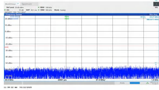
NTNV-n77(3700-3980)-PC2-30-60-M-DFT-BPSK-Inner_1RB_Righ t-30-1000-PASS
