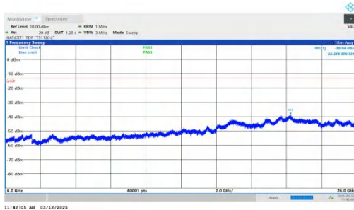
NTNV-n77(3700-3980)-PC2-30-60-M-DFT-QPSK-Inner_1RB_Rig ht-6000-26000-PASS
