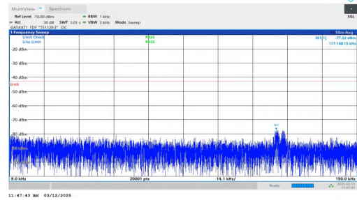
NTNV-n77(3700-3980)-PC2-30-60-H-DFT-QPSK-Inner_1RB_Right t.009-0.15-PASS
