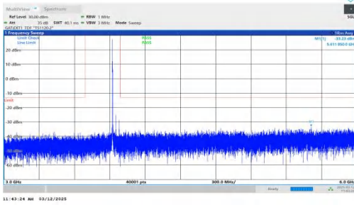
NTNV-n77(3700-3980)-PC2-30-60-H-DFT-BPSK-Inner_1RB_Left -3000-6000-PASS
