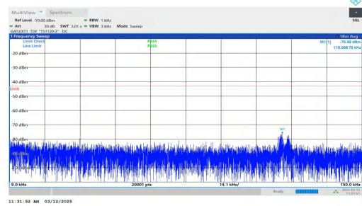
NTNV-n77(3700-3980)-PC2-30-60-L-DFT-BPSK-Inner_1RB_Right-0.009-0.15-PASS
