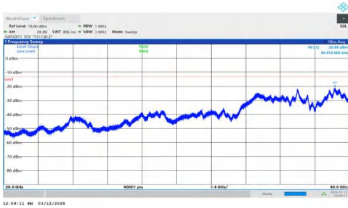
NTNV-n77(3700-3980)-PC2-30-100-L-DFT-BPSK-Inner_1RB_Lef t-26000-40000-PASS
