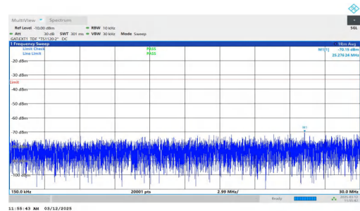
NTNV-n77(3700-3980)-PC2-30-80-M-DFT-BPSK-Inner_1RB_Left- 0.15-30-PASS
