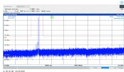
NTNV-n77(3700-3980)-PC2-30-60-M-DFT-BPSK-Inner_1RB_Righ t-3000-6000-PASS
