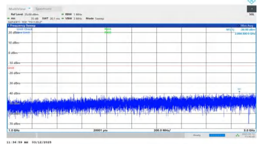
NTNV-n77(3700-3980)-PC2-30-60-M-DFT-BPSK-Inner_1RB_Left 1000-3000-PASS
