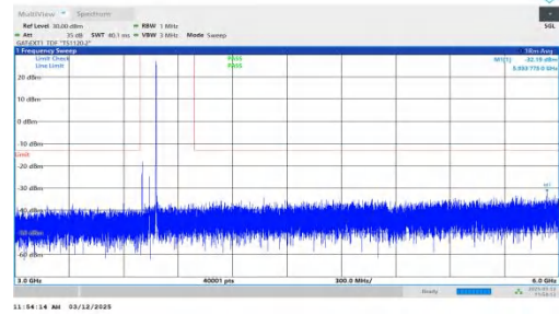
NTNV-n77(3700-3980)-PC2-30-80-L-DFT-QPSK-Inner_1RB_Right -3000-6000-PASS
