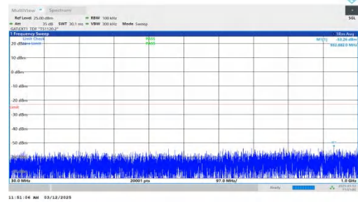
NTNV-n77(3700-3980)-PC2-30-80-L-DFT-BPSK-Inner_1RB_Right -30-1000-PASS
