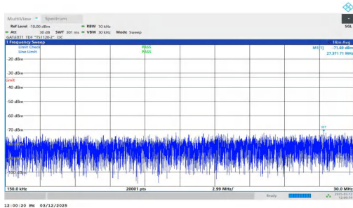
NTNV-n77(3700-3980)-PC2-30-80-M-DFT-QPSK-Inner_1RB_Rig ht-0.15-30-PASS
