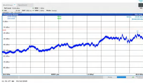
NTNV-n77(3700-3980)-PC2-30-60-L-DFT-BPSK-Inner_1RB_Left-26000-40000-PASS
