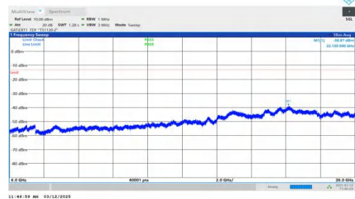
NTNV-n77(3700-3980)-PC2-30-60-H-DFT-QPSK-Inner_1RB_Left- 6000-26000-PASS
