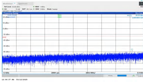
NTNV-n77(3700-3980)-PC2-30-80-H-DFT-QPSK-Inner_1RB_Rig ht-1000-3000-PASS
