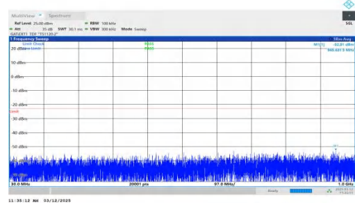
NTNV-n77(3700-3980)-PC2-30-60-L-DFT-QPSK-Inner_1RB_Right -30-1000-PASS
