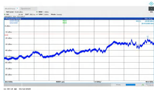
NTNV-n77(3700-3980)-PC2-30-60-M-DFT-BPSK-Inner_1RB_Righ t-26000-40000-PASS
