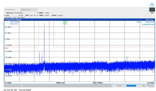
NTNV-n77(3700-3980)-PC2-30-100-L-DFT-BPSK-Inner_1RB_Rig ht-3000-6000-PASS
