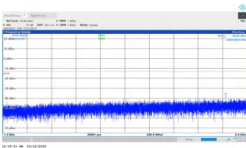
NTNV-n77(3700-3980)-PC2-30-100-L-DFT-BPSK-Inner_1RB_Ri ght-1000-3000-PASS
