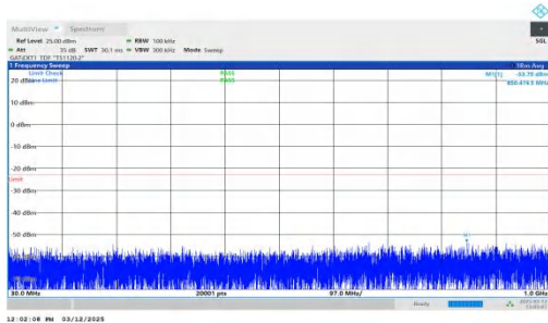
NTNV-n77(3700-3980)-PC2-30-80-H-DFT-BPSK-Inner_1RB_Left -30-1000-PASS
