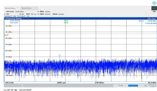
NTNV-n77(3700-3980)-PC2-30-80-M-DFT-QPSK-Inner_1RB_Left- 0.15-30-PASS
