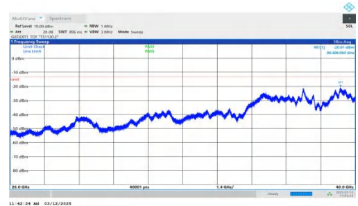
NTNV-n77(3700-3980)-PC2-30-60-M-DFT-QPSK-Inner_1RB_Righ t-26000-40000-PASS
