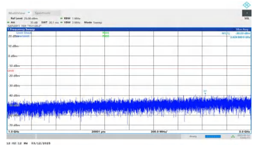
NTNV-n77(3700-3980)-PC2-30-80-H-DFT-BPSK-Inner_1RB_Left- 1000-3000-PASS
