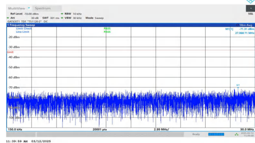
NTNV-n77(3700-3980)-PC2-30-60-M-DFT-QPSK-Inner_1RB_Left- 0.15-30-PASS
