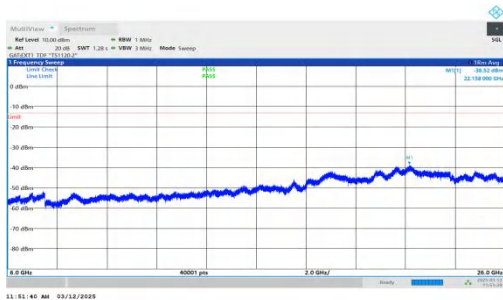
NTNV-n77(3700-3980)-PC2-30-80-L-DFT-BPSK-Inner_1RB_Rig ht-6000-26000-PASS
