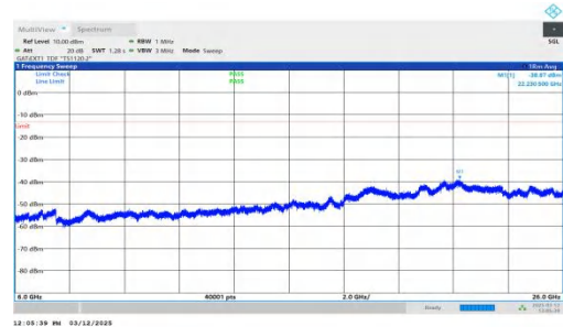
NTNV-n77(3700-3980)-PC2-30-80-H-DFT-QPSK-Inner_1RB_Left 6000-26000-PASS
