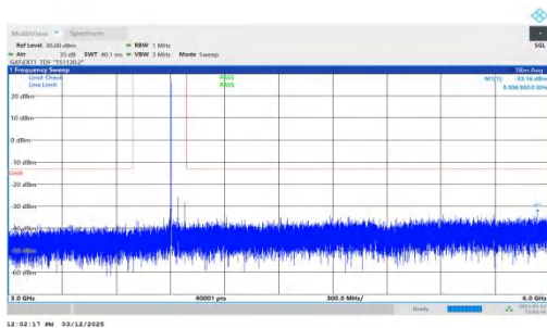
NTNV-n77(3700-3980)-PC2-30-80-H-DFT-BPSK-Inner_1RB_Left -3000-6000-PASS
