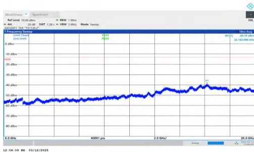
NTNV-n77(3700-3980)-PC2-30-80-H-DFT-BPSK-Inner_1RB_Rig ht-6000-26000-PASS
