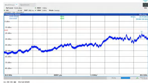
NTNV-n77(3700-3980)-PC2-30-60-L-DFT-QPSK-Inner_1RB_Right -26000-40000-PASS
