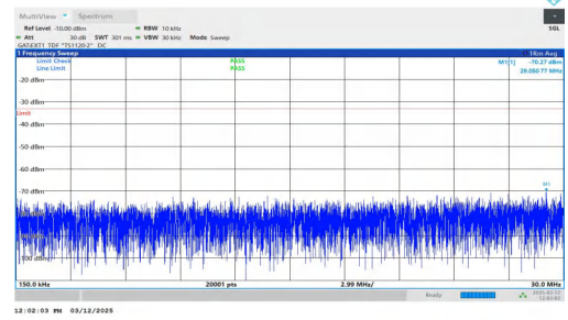
NTNV-n77(3700-3980)-PC2-30-80-H-DFT-BPSK-Inner_1RB_Left- 0.15-30-PASS
