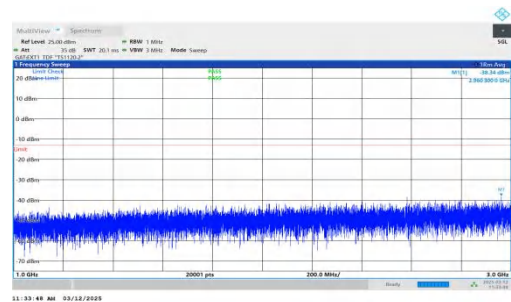
NTNV-n77(3700-3980)-PC2-30-60-L-DFT-QPSK-Inner_1RB_Left- 1000-3000-PASS
