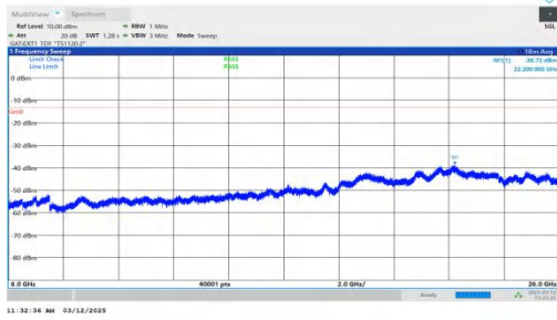
NTNV-n77(3700-3980)-PC2-30-60-L-DFT-BPSK-Inner_1RB_Rig ht-6000-26000-PASS
