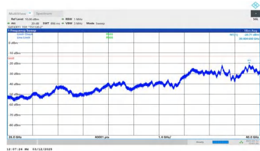
NTNV-n77(3700-3980)-PC2-30-80-H-DFT-QPSK-Inner_1RB_Righ t-26000-40000-PASS
