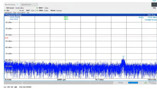
NTNV-n77(3700-3980)-PC2-30-60-L-DFT-QPSK-Inner_1RB_Right -0.009-0.15-PASS
