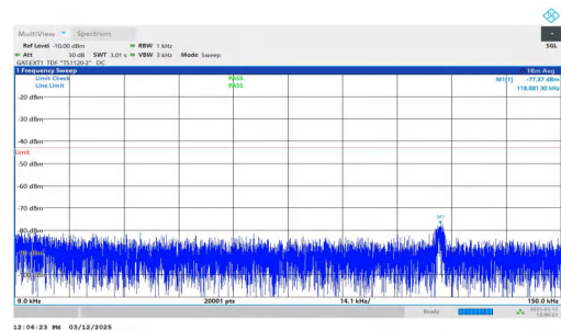
NTNV-n77(3700-3980)-PC2-30-80-H-DFT-QPSK-Inner_1RB_Right t-0.009-0.15-PASS
