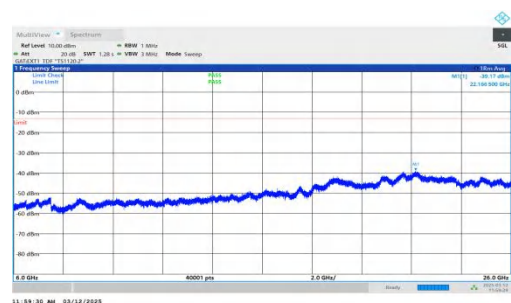
NTNV-n77(3700-3980)-PC2-30-80-M-DFT-QPSK-Inner_1RB_Left- 6000-26000-PASS
