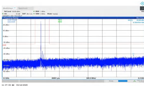
NTNV-n77(3700-3980)-PC2-30-60-M-DFT-BPSK-Inner_1RB_Left -3000-6000-PASS
