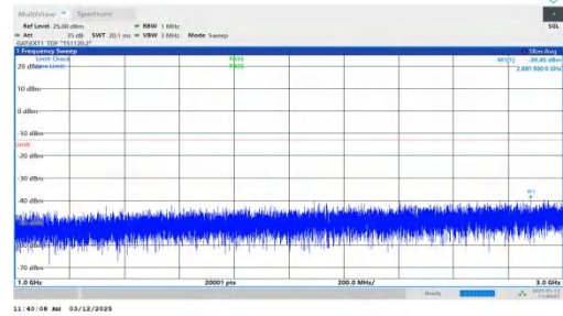
NTNV-n77(3700-3980)-PC2-30-60-M-DFT-QPSK-Inner_1RB_Left- 1000-3000-PASS
