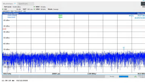
NTNV-n77(3700-3980)-PC2-30-60-M-DFT-BPSK-Inner_1RB_Rig ht-0.15-30-PASS
