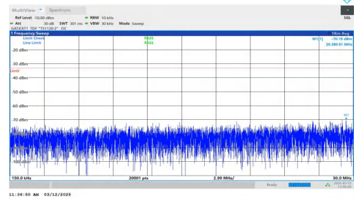
NTNV-n77(3700-3980)-PC2-30-60-M-DFT-BPSK-Inner_1RB_Left 0.15-30-PASS
