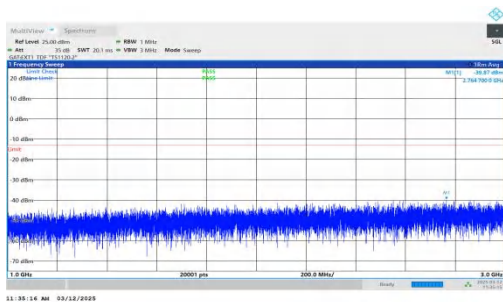
NTNV-n77(3700-3980)-PC2-30-60-L-DFT-QPSK-Inner_1RB_Rig ht-1000-3000-PASS
