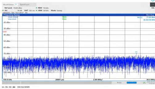
NTNV-n77(3700-3980)-PC2-30-80-L-DFT-BPSK-Inner_1RB_Rig ht-0.15-30-PASS
