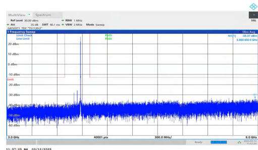
NTNV-n77(3700-3980)-PC2-30-80-M-DFT-BPSK-Inner_1RB_Right t-3000-6000-PASS
