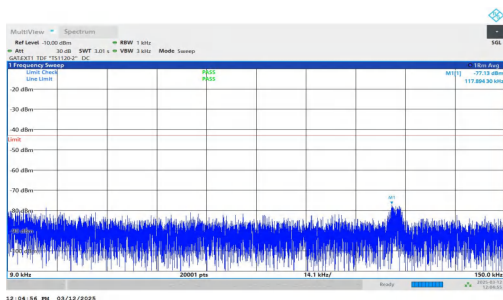
NTNV-n77(3700-3980)-PC2-30-80-H-DFT-QPSK-Inner_1RB_Left -0.009-0.15-PASS
