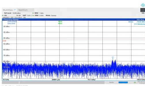
NTNV-n77(3700-3980)-PC2-30-80-L-DFT-QPSK-Inner_1RB_Left -0.009-0.15-PASS
