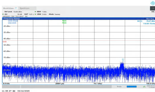
NTNV-n77(3700-3980)-PC2-30-80-M-DFT-QPSK-Inner_1RB_Lef t-0.009-0.15-PASS
