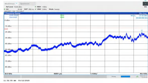
NTNV-n77(3700-3980)-PC2-30-60-L-DFT-BPSK-Inner_1RB_Right -26000-40000-PASS
