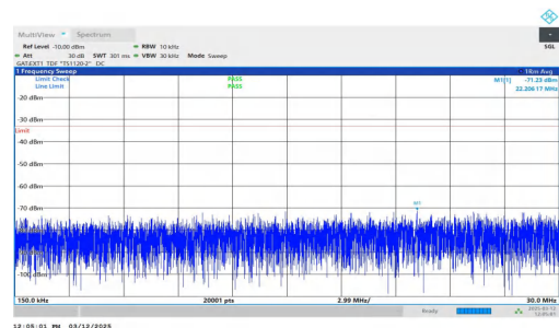
NTNV-n77(3700-3980)-PC2-30-80-H-DFT-QPSK-Inner_1RB_Left 0.15-30-PASS
