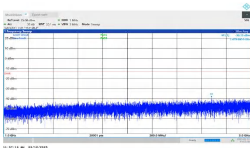
NTNV-n77(3700-3980)-PC2-30-80-M-DFT-BPSK-Inner_1RB_Right ht-1000-3000-PASS
