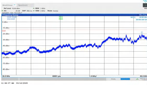
NTNV-n77(3700-3980)-PC2-30-60-H-DFT-BPSK-Inner_1RB_Left -26000-40000-PASS
