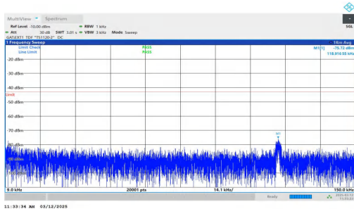
NTNV-n77(3700-3980)-PC2-30-60-L-DFT-QPSK-Inner_1RB_Left -0.009-0.15-PASS
