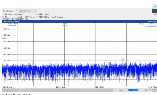
NTNV-n77(3700-3980)-PC2-30-60-M-DFT-QPSK-Inner_1RB_Rig ht-0.15-30-PASS
