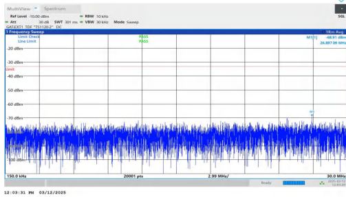
NTNV-n77(3700-3980)-PC2-30-80-H-DFT-BPSK-Inner_1RB_Rig ht-0.15-30-PASS
