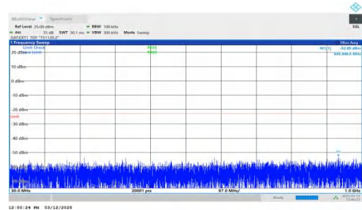
NTNV-n77(3700-3980)-PC2-30-80-M-DFT-QPSK-Inner_1RB_Righ t-30-1000-PASS
