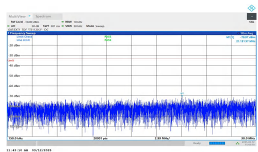
NTNV-n77(3700-3980)-PC2-30-60-H-DFT-BPSK-Inner_1RB_Left- 0.15-30-PASS
