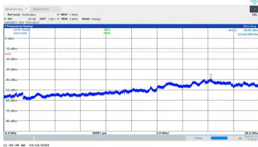
NTNV-n77(3700-3980)-PC2-30-80-L-DFT-QPSK-Inner_1RB_Rig ht-6000-26000-PASS
