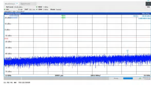
NTNV-n77(3700-3980)-PC2-30-80-L-DFT-QPSK-Inner_1RB_Left- 1000-3000-PASS
