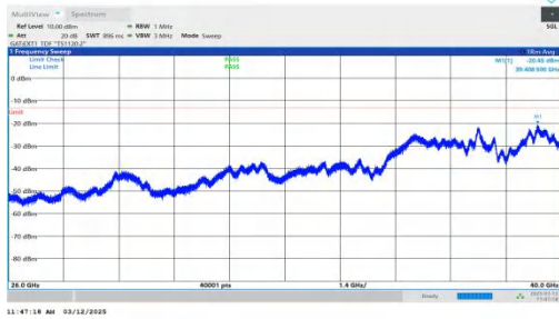
NTNV-n77(3700-3980)-PC2-30-60-H-DFT-QPSK-Inner_1RB_Left -26000-40000-PASS
