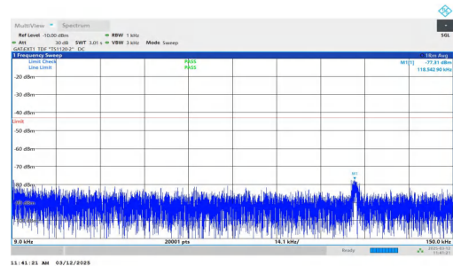
NTNV-n77(3700-3980)-PC2-30-60-M-DFT-QPSK-Inner_1RB_Right t-0.009-0.15-PASS
