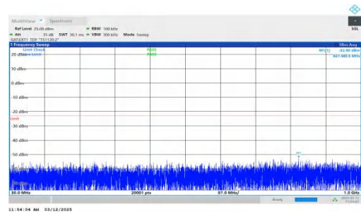
NTNV-n77(3700-3980)-PC2-30-80-L-DFT-QPSK-Inner_1RB_Right -30-1000-PASS
