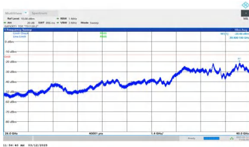
NTNV-n77(3700-3980)-PC2-30-80-M-DFT-BPSK-Inner_1RB_Left -26000-40000-PASS
