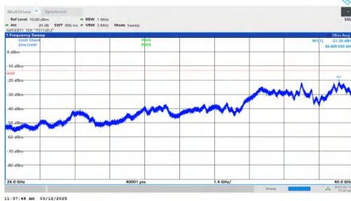
NTNV-n77(3700-3980)-PC2-30-60-M-DFT-BPSK-Inner_1RB_Left -26000-40000-PASS
