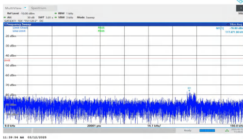
NTNV-n77(3700-3980)-PC2-30-60-M-DFT-QPSK-Inner_1RB_Lef t-0.009-0.15-PASS
