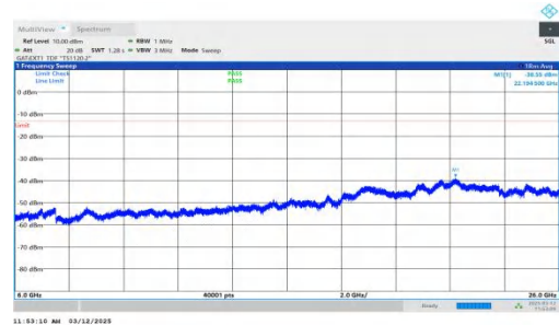
NTNV-n77(3700-3980)-PC2-30-80-L-DFT-QPSK-Inner_1RB_Left- 6000-26000-PASS
