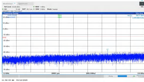
NTNV-n77(3700-3980)-PC2-30-80-L-DFT-QPSK-Inner_1RB_Rig ht-1000-3000-PASS
