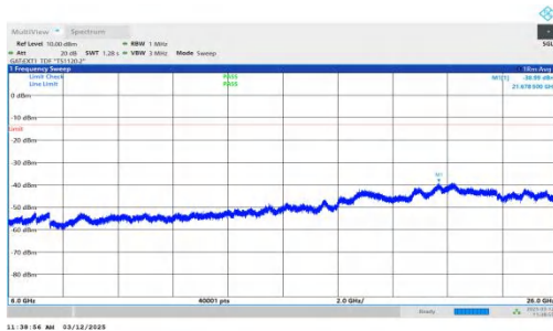
NTNV-n77(3700-3980)-PC2-30-60-M-DFT-BPSK-Inner_1RB_Rig ht-6000-26000-PASS
