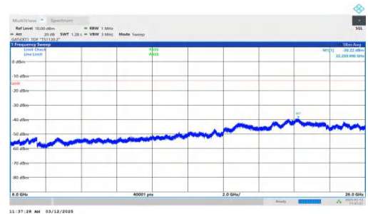
NTNV-n77(3700-3980)-PC2-30-60-M-DFT-BPSK-Inner_1RB_Left 6000-26000-PASS
