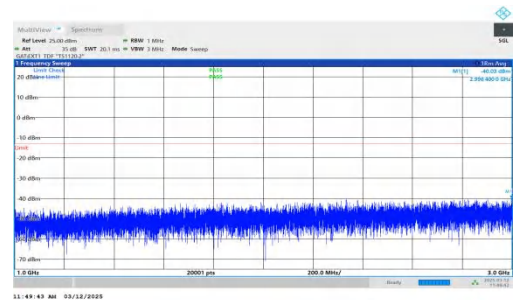
NTNV-n77(3700-3980)-PC2-30-80-L-DFT-BPSK-Inner_1RB_Left- 1000-3000-PASS
