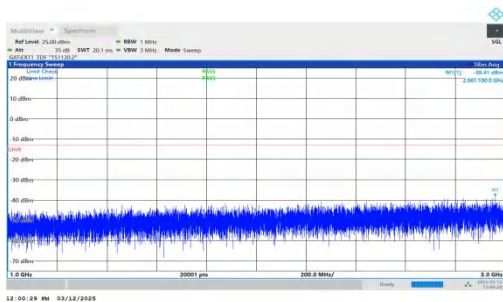
NTNV-n77(3700-3980)-PC2-30-80-M-DFT-QPSK-Inner_1RB_Rig ht-1000-3000-PASS
