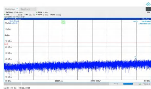
NTNV-n77(3700-3980)-PC2-30-60-H-DFT-QPSK-Inner_1RB_Left- 1000-3000-PASS
