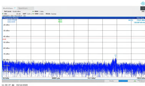
NTNV-n77(3700-3980)-PC2-30-80-M-DFT-BPSK-Inner_1RB_Left -0.009-0.15-PASS
