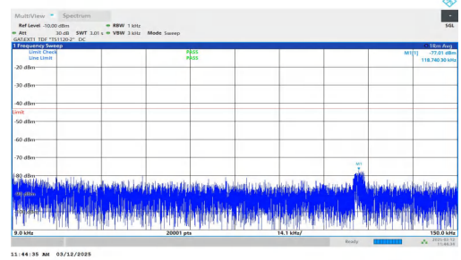
NTNV-n77(3700-3980)-PC2-30-60-H-DFT-BPSK-Inner_1RB_Right t-0.009-0.15-PASS
