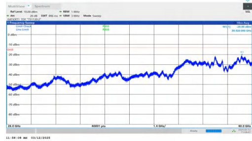
NTNV-n77(3700-3980)-PC2-30-80-M-DFT-BPSK-Inner_1RB_Righ t-26000-40000-PASS
