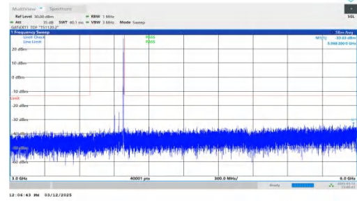
NTNV-n77(3700-3980)-PC2-30-80-H-DFT-QPSK-Inner_1RB_Righ t-3000-6000-PASS
