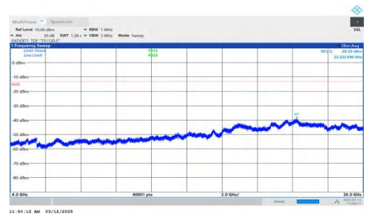
NTNV-n77(3700-3980)-PC2-30-80-L-DFT-BPSK-Inner_1RB_Left- 6000-26000-PASS
