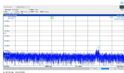
NTNV-n77(3700-3980)-PC2-30-80-L-DFT-QPSK-Inner_1RB_Right -0.009-0.15-PASS
