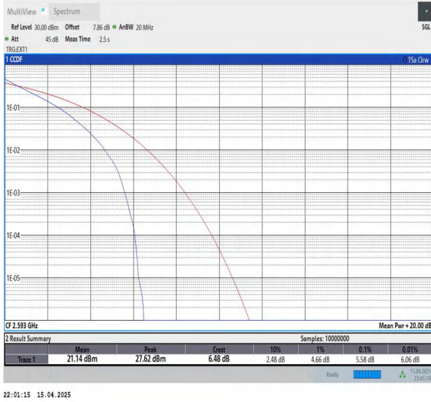
Band41-15MHz-QPSK-40620-75RB#0-PASS
