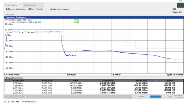
Band41-5MHz-QPSK-41565-25RB#0-PASS
