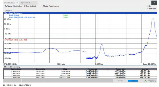
Band41-5MHz-QPSK-39675-1RB#24-PASS
