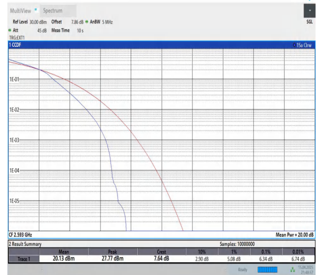
Band41-5MHz-16QAM-40620-25RB#0-PASS
