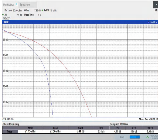
Band41-10MHz-QPSK-40620-50RB#0-PASS
