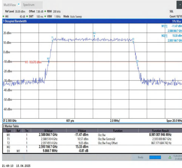
Band41-10MHz-QPSK-40620-50RB#0-PASS
