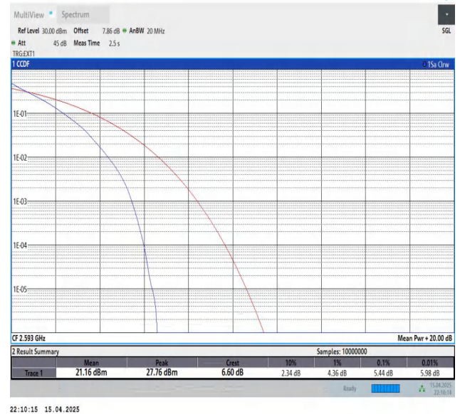
Band41-20MHz-QPSK-40620-100RB#0-PASS
