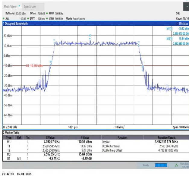
Band41-5MHz-QPSK-40620-25RB#0-PASS
