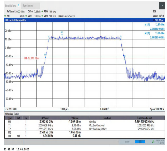
Band41-5MHz-16QAM-40620-25RB#0-PASS
