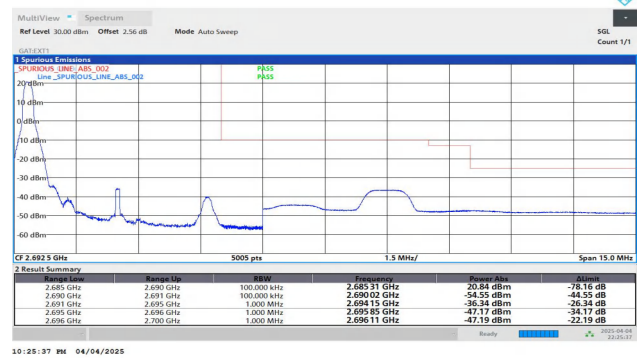
Band41-5MHz-QPSK-41565-1RB#0-PASS
