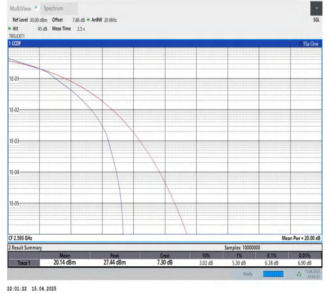
Band41-15MHz-16QAM-40620-75RB#0-PASS
