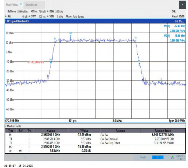
Band41-10MHz-16QAM-40620-50RB#0-PASS
