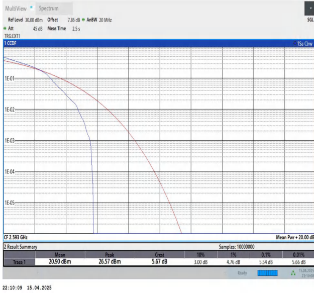
Band41-20MHz-16QAM-40620-1RB#0-PASS
