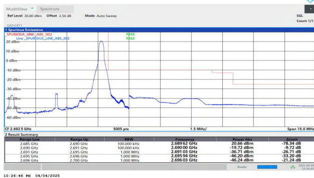
Band41-5MHz-QPSK-41565-1RB#24-PASS
