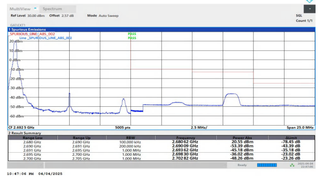
Band41-10MHz-QPSK-41540-1RB#0-PASS
