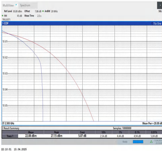
Band41-20MHz-QPSK-40620-1RB#0-PASS
