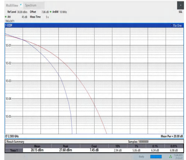
Band41-10MHz-16QAM-40620-50RB#0-PASS
