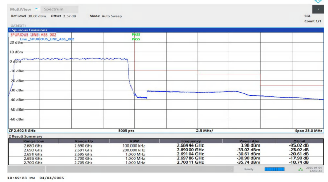
Band41-10MHz-QPSK-41540-50RB#0-PASS
