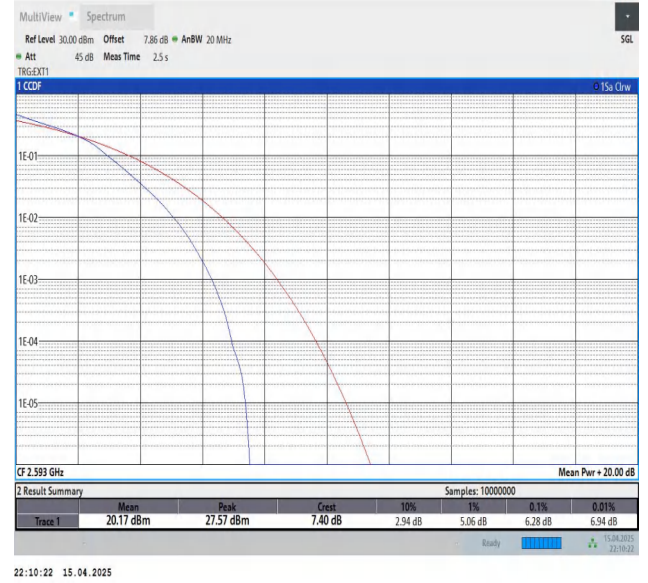
Band41-20MHz-16QAM-40620-100RB#0-PASS
