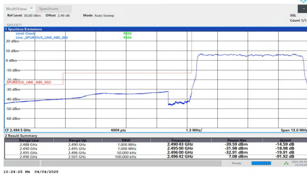
Band41-5MHz-QPSK-39675-25RB#0-PASS
