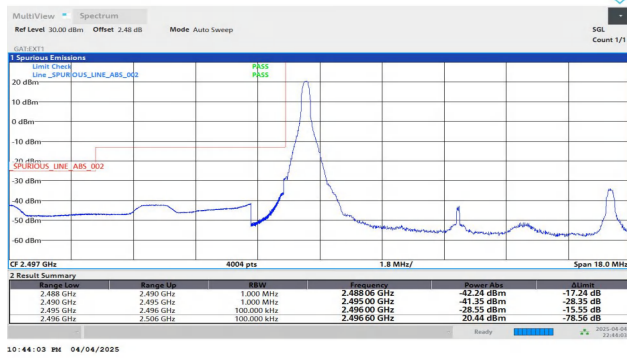
Band41-10MHz-QPSK-39700-1RB#0-PASS
