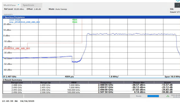
Band41-10MHz-QPSK-39700-50RB#0-PASS
