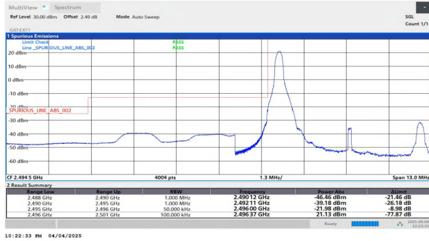
Band41-5MHz-QPSK-39675-1RB#0-PASS
