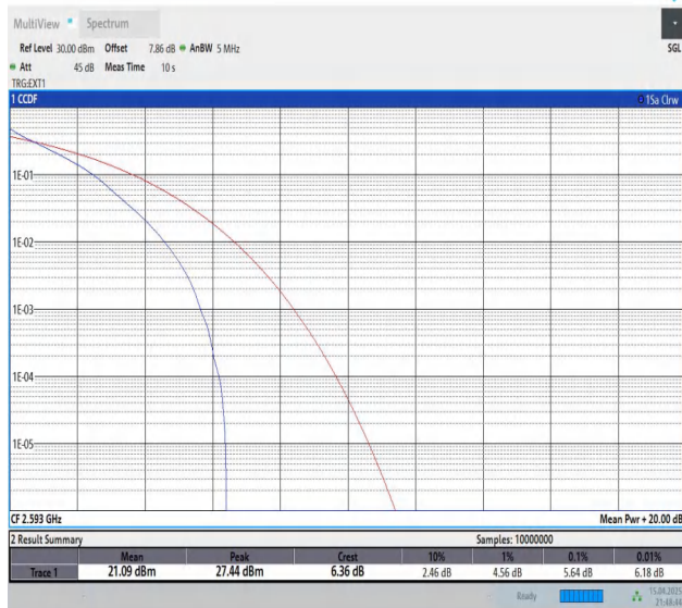
Band41-5MHz-QPSK-40620-25RB#0-PASS
