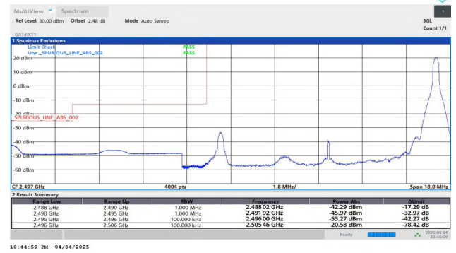
Band41-10MHz-QPSK-39700-1RB#49-PASS
