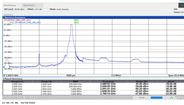
Band41-10MHz-QPSK-41540-1RB#49-PASS
