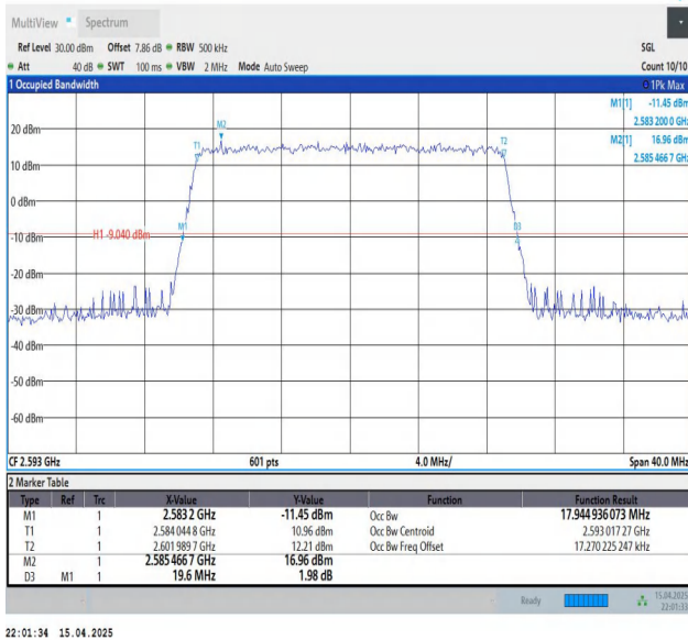
Band41-20MHz-QPSK-40620-100RB#0-PASS
