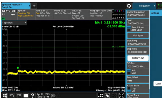
Band5-1.4MHz-QPSK-20407-1RB#0-3000~10000-PASS
