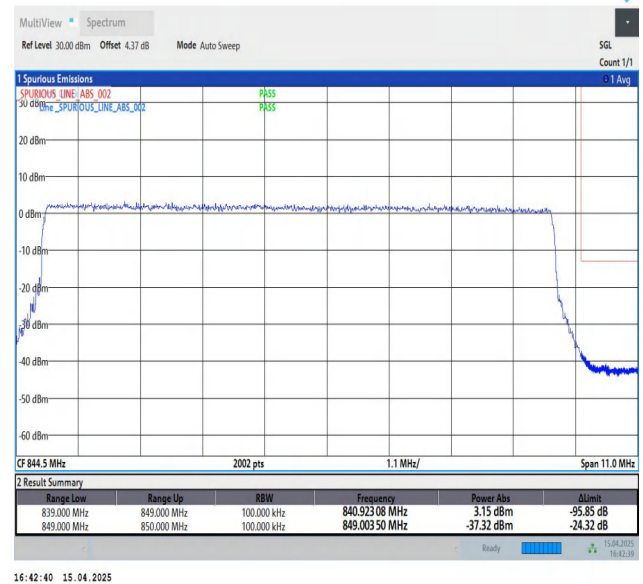
Band5-10MHz-QPSK-20600-50RB#0-PASS
