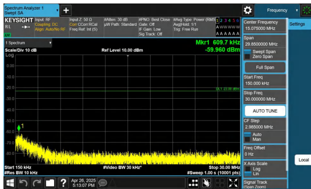
Band5-3MHz-QPSK-20525-1RB#14-0.15~30-PASS
