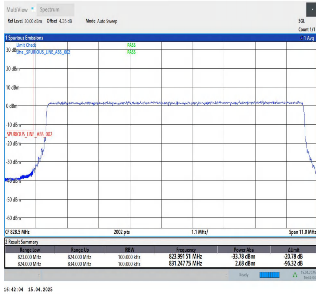
Band5-10MHz-QPSK-20450-50RB#0-PASS
