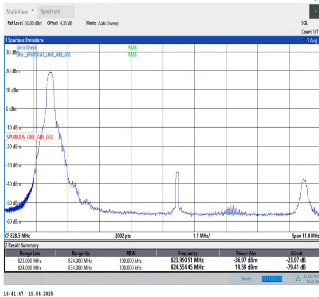
Band5-10MHz-QPSK-20450-1RB#0-PASS
