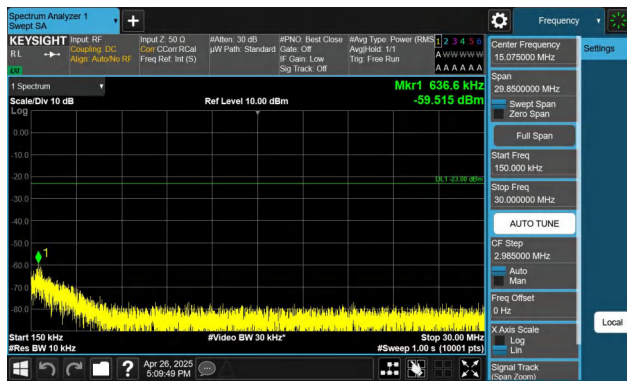
Band5-1.4MHz-QPSK-20643-1RB#5-0.15~30-PASS
