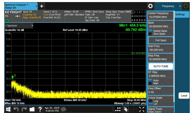
Band5-1.4MHz-QPSK-20643-1RB#0-0.15~30-PASS
