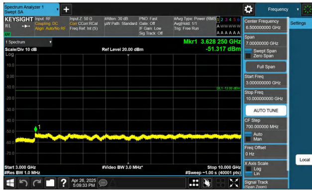
Band5-1.4MHz-QPSK-20643-1RB#0-3000~10000-PASS
