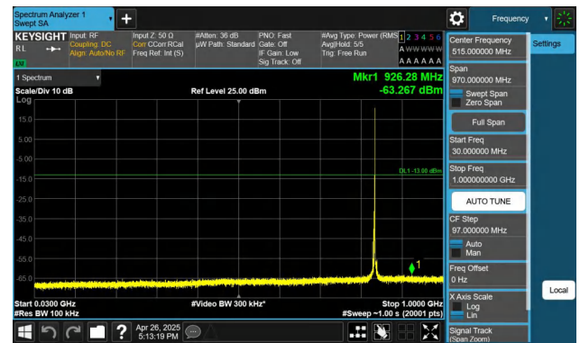
Band5-3MHz-QPSK-20525-1RB#14-30~1000-PASS
