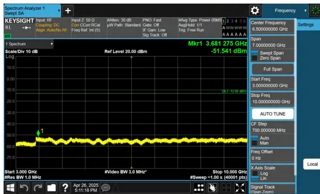
Band5-3MHz-QPSK-20415-1RB#0-3000~10000-PASS
