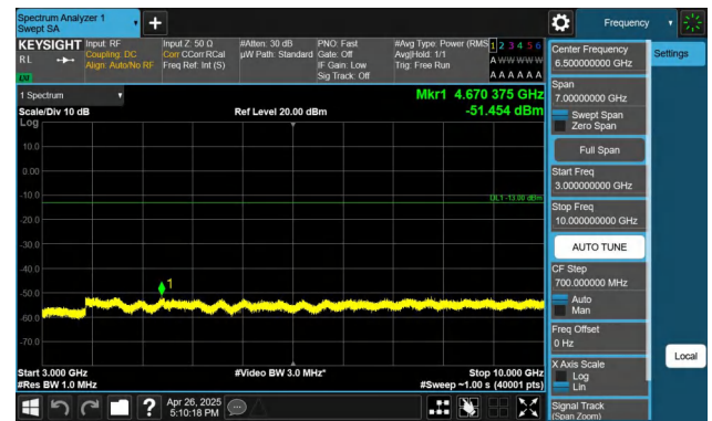
Band5-1.4MHz-QPSK-20643-1RB#5-3000~10000-PASS
