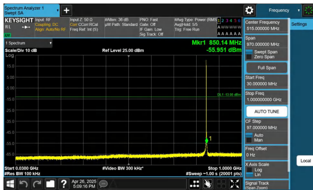
Band5-1.4MHz-QPSK-20643-1RB#0-30~1000-PASS
