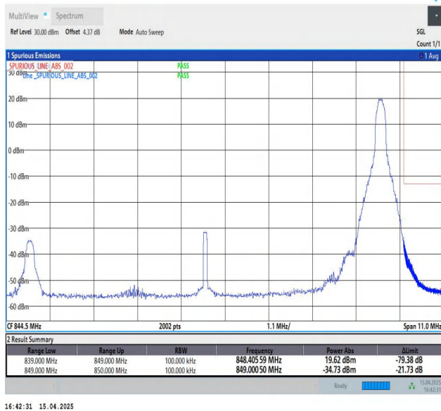
Band5-10MHz-QPSK-20600-1RB#49-PASS
