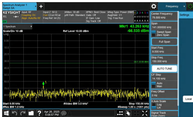
Band5-1.4MHz-QPSK-20643-1RB#0-0.009~0.15-PASS
