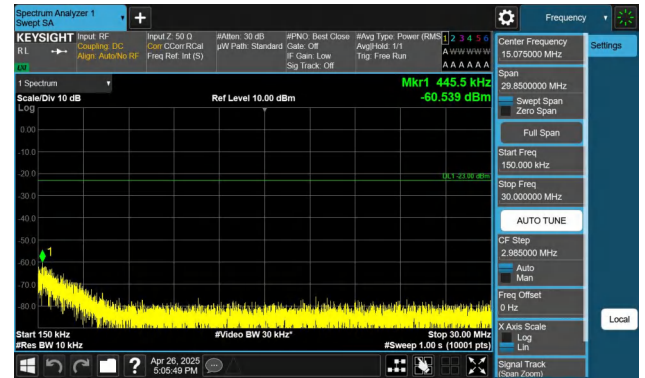
Band5-1.4MHz-QPSK-20407-1RB#0-0.15~30-PASS
