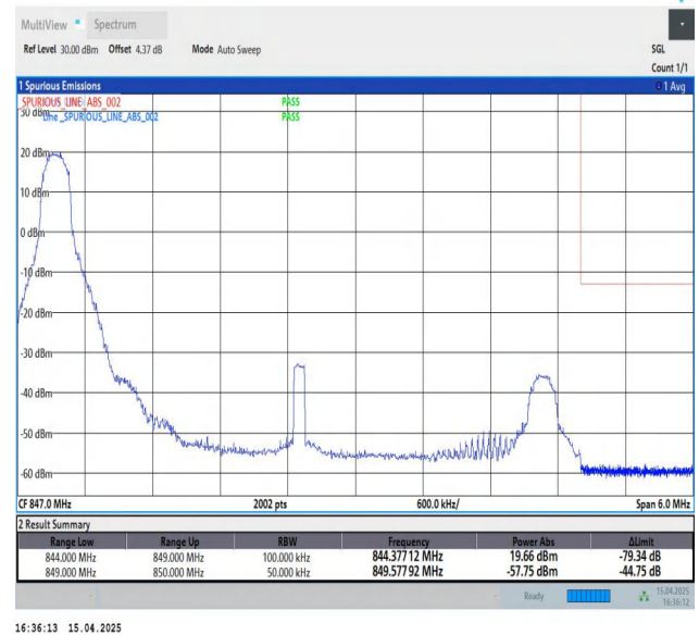
Band5-5MHz-QPSK-20625-1RB#0-PASS
