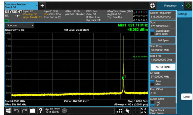
Band5-3MHz-QPSK-20415-1RB#14-30~1000-PASS
