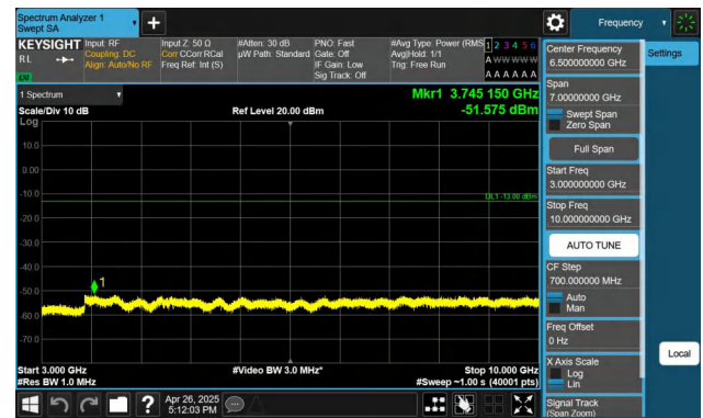
Band5-3MHz-QPSK-20415-1RB#14-3000~10000-PASS
