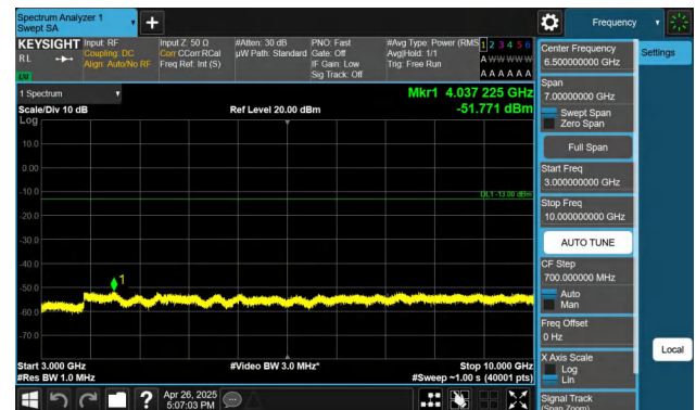
Band5-1.4MHz-QPSK-20407-1RB#5-3000~10000-PASS
