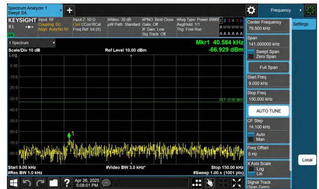
Band5-1.4MHz-QPSK-20525-1RB#5-0.009~0.15-PASS
