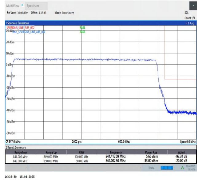
Band5-5MHz-QPSK-20625-25RB#0-PASS
