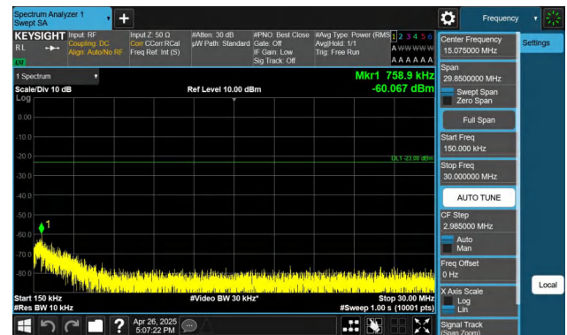
Band5-1.4MHz-QPSK-20525-1RB#0-0.15~30-PASS
