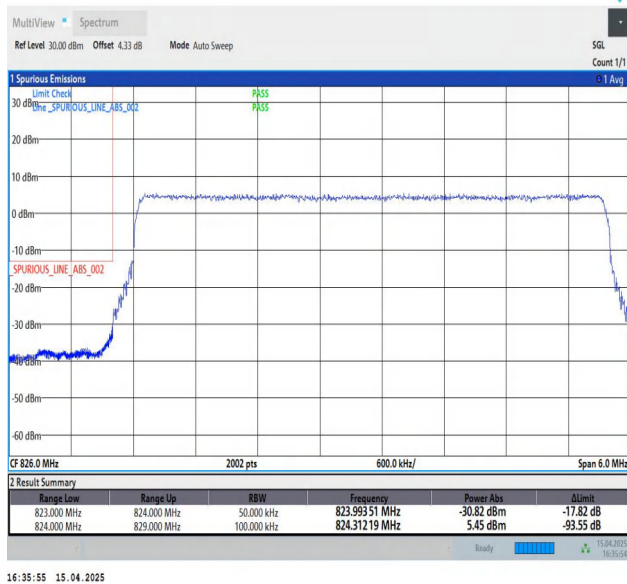
Band5-5MHz-QPSK-20425-25RB#0-PASS
