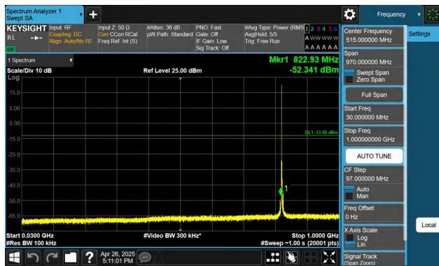
Band5-3MHz-QPSK-20415-1RB#0-30~1000-PASS
