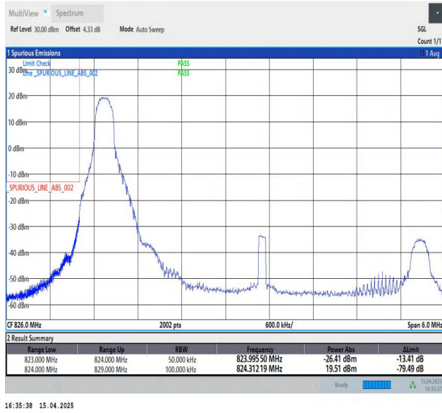
Band5-5MHz-QPSK-20425-1RB#0-PASS
