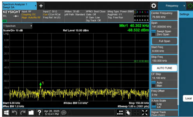
Band5-3MHz-QPSK-20415-1RB#0-0.009~0.15-PASS
