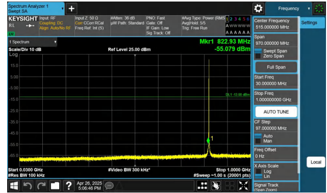
Band5-1.4MHz-QPSK-20407-1RB#5-30~1000-PASS
