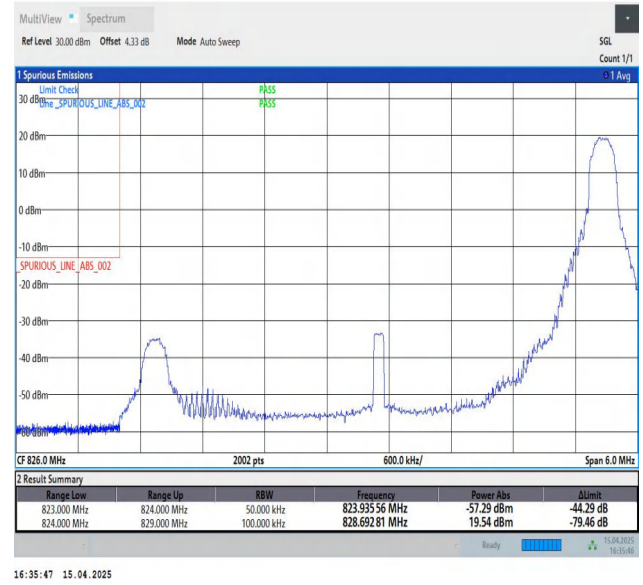
Band5-5MHz-QPSK-20425-1RB#24-PASS
