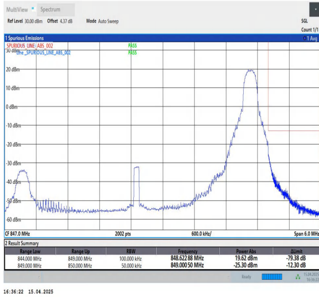
Band5-5MHz-QPSK-20625-1RB#24-PASS
