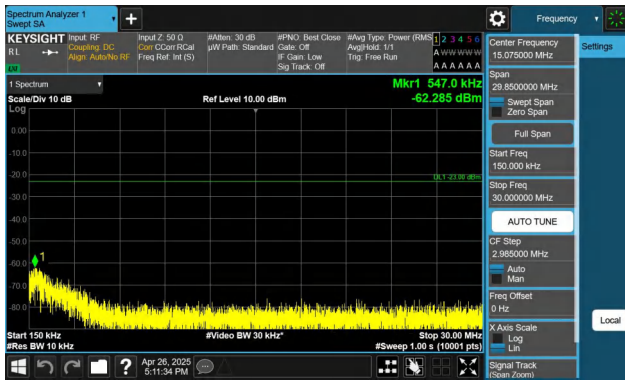
Band5-3MHz-QPSK-20415-1RB#14-0.15~30-PASS
