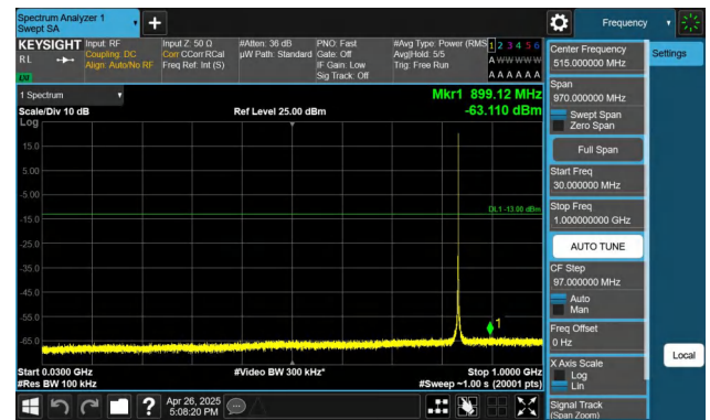
Band5-1.4MHz-QPSK-20525-1RB#5-30~1000-PASS
