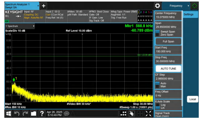
Band5-3MHz-QPSK-20415-1RB#0-0.15~30-PASS
