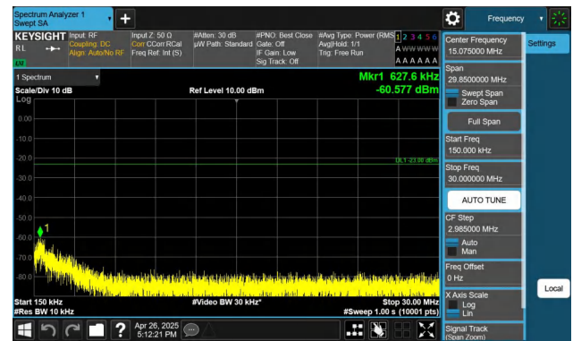
Band5-3MHz-QPSK-20525-1RB#0-0.15~30-PASS
