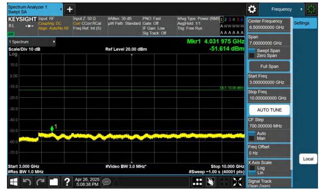
Band5-1.4MHz-QPSK-20525-1RB#5-3000~10000-PASS
