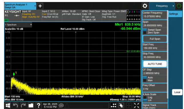
Band5-3MHz-QPSK-20635-1RB#0-0.15~30-PASS
