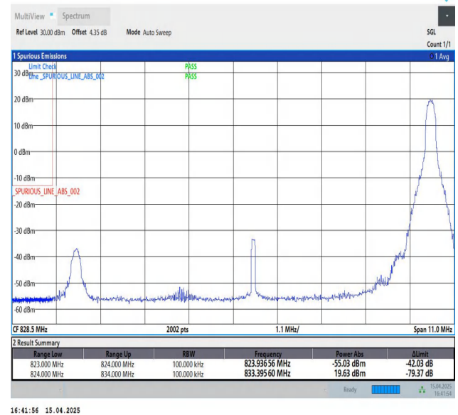
Band5-10MHz-QPSK-20450-1RB#49-PASS
