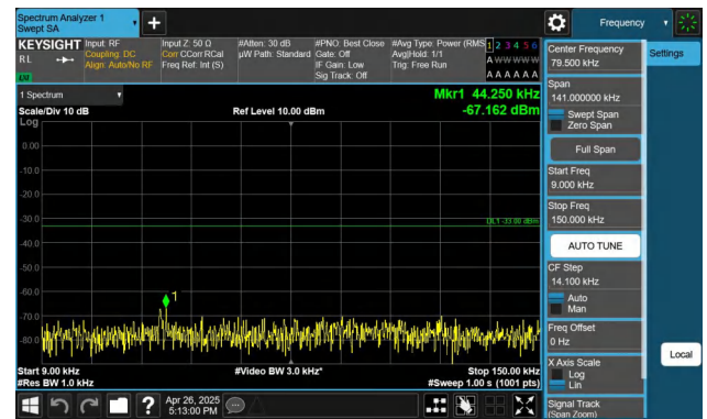
Band5-3MHz-QPSK-20525-1RB#14-0.009~0.15-PASS
