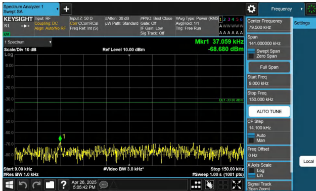
Band5-1.4MHz-QPSK-20407-1RB#0-0.009~0.15-PASS
