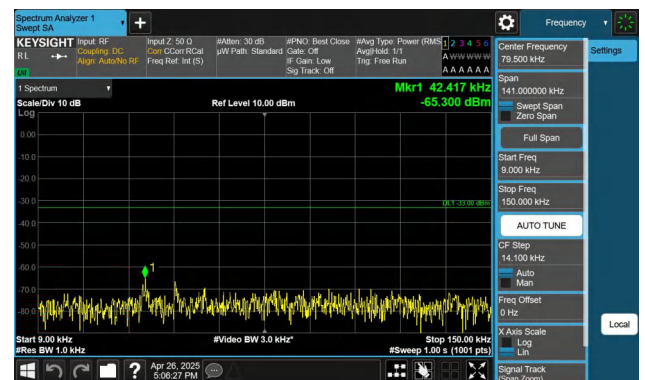
Band5-1.4MHz-QPSK-20407-1RB#5-0.009~0.15-PASS
