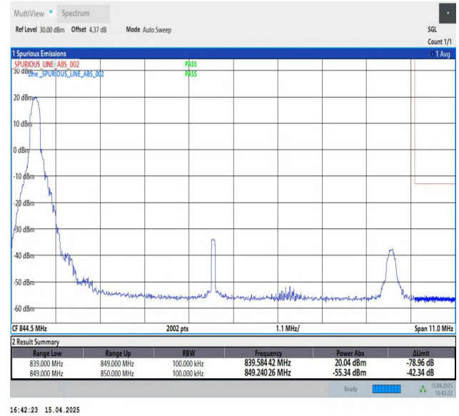
Band5-10MHz-QPSK-20600-1RB#0-PASS
