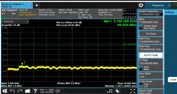
Band26(824-849)-10MHz-QPSK-26915-1RB#0-3000~10000-PAS
