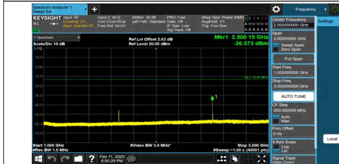
Band26(824-849)-10MHz-QPSK-26840-1RB#49-1000~3000-PAS
