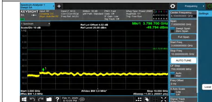
Band26(824-849)-15MHz-QPSK-26865-1RB#0-3000~10000-PAS
