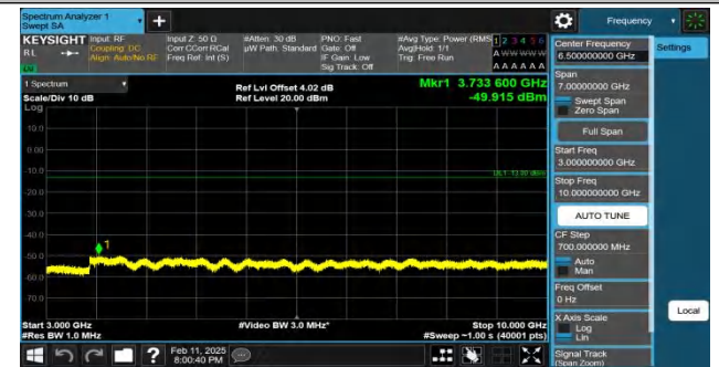
Band26(824-849)-10MHz-QPSK-26840-1RB#49-3000~10000-PAS
