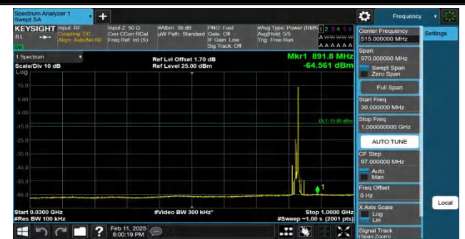
Band26(824-849)-10MHz-QPSK-26840-1RB#49-30~1000-PASS
