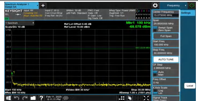
Band26(824-849)-15MHz-QPSK-26915-1RB#0-0.15~30-PASS
