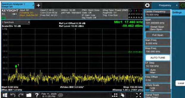
Band26(824-849)-15MHz-QPSK-26915-1RB#0-0.009~0.15-PASS
