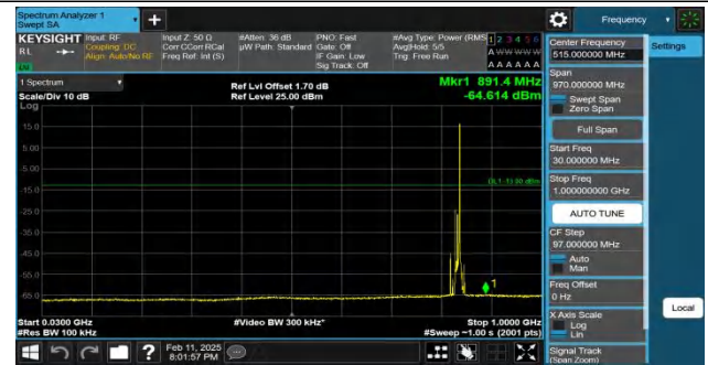
Band26(824-849)-10MHz-QPSK-26915-1RB#49-30~1000-PASS
