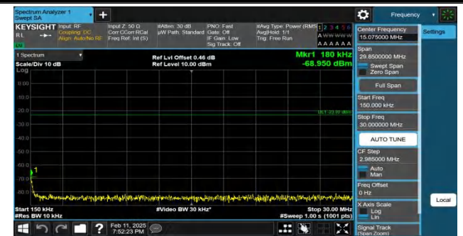
Band26(824-849)-5MHz-QPSK-27015-1RB#0-0.15~30-PASS
