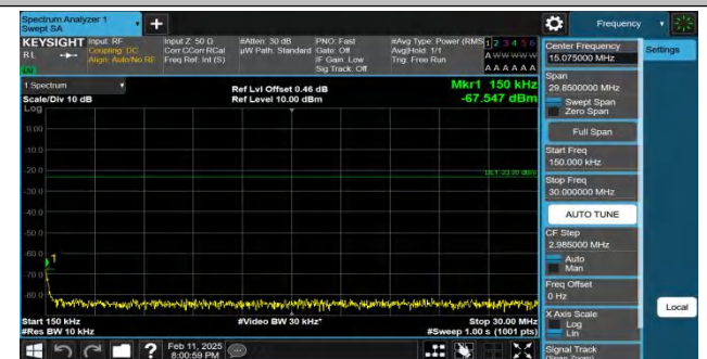
Band26(824-849)-10MHz-QPSK-26915-1RB#0-0.15~30-PASS
