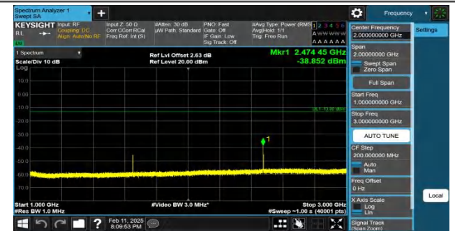
Band26(824-849)-15MHz-QPSK-26865-1RB#0-1000~3000-PASS
