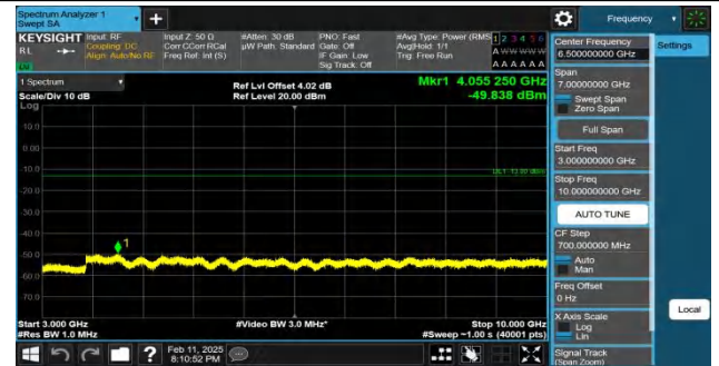
Band26(824-849)-15MHz-QPSK-26865-1RB#74-3000~10000-PAS
