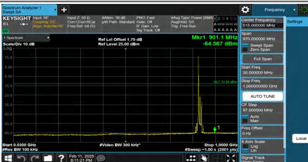
Band26(824-849)-15MHz-QPSK-26915-1RB#0-30~1000-PASS
