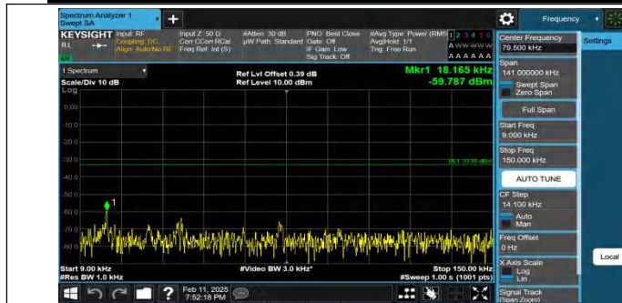
Band26(824-849)-5MHz-QPSK-27015-1RB#0-0.009~0.15-PASS
