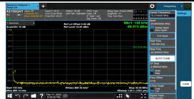
Band26(824-849)-15MHz-QPSK-26865-1RB#0-0.15~30-PASS
