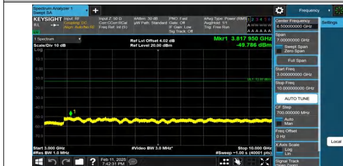
Band26(824-849)-3MHz-QPSK-27025-1RB#0-3000~10000-PASS
