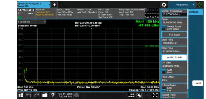
Band26(824-849)-3MHz-QPSK-27025-1RB#0-0.15~30-PASS
