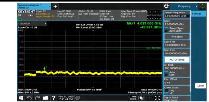
Band26(824-849)-3MHz-QPSK-26915-1RB#14-3000~10000-PASS
