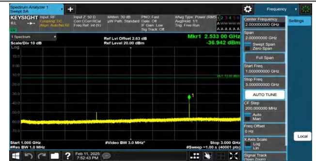
Band26(824-849)-5MHz-QPSK-27015-1RB#0-1000~3000-PASS
