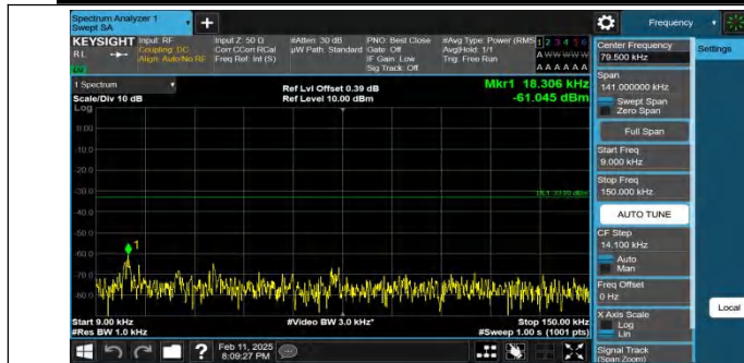
Band26(824-849)-15MHz-QPSK-26865-1RB#0-0.009~0.15-PASS
