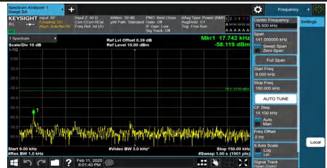
Band26(824-849)-10MHz-QPSK-26915-1RB#49-0.009~0.15-PASS
