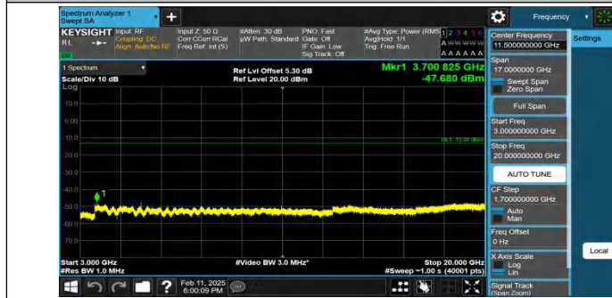
Band25-3MHz-QPSK-26055-1RB#0-3000~20000-PASS
