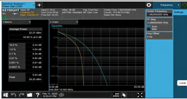
Band25-15MHz-QPSK-26365-75RB#0-PASS
