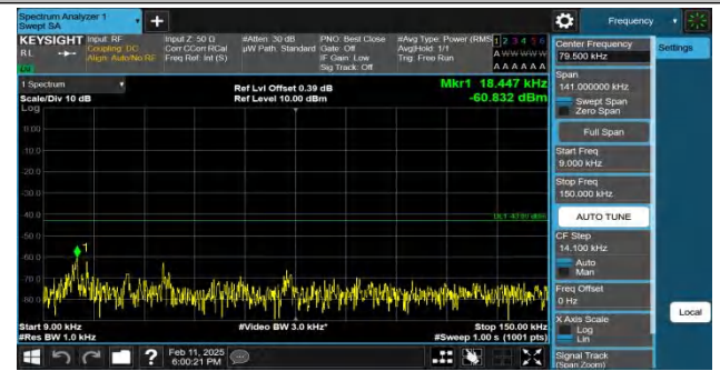
Band25-3MHz-QPSK-26055-1RB#14-0.009~0.15-PASS
