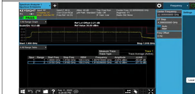
Band25-15MHz-QPSK-26615-1RB#74-PASS
