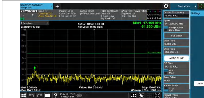
Band12-3MHz-QPSK-23025-1RB#0-0.009~0.15-PASS
