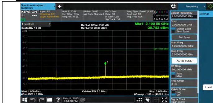
Band12-1.4MHz-QPSK-23017-1RB#5-1000~3000-PASS
