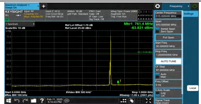
Band12-5MHz-QPSK-23095-1RB#24-30~1000-PASS
