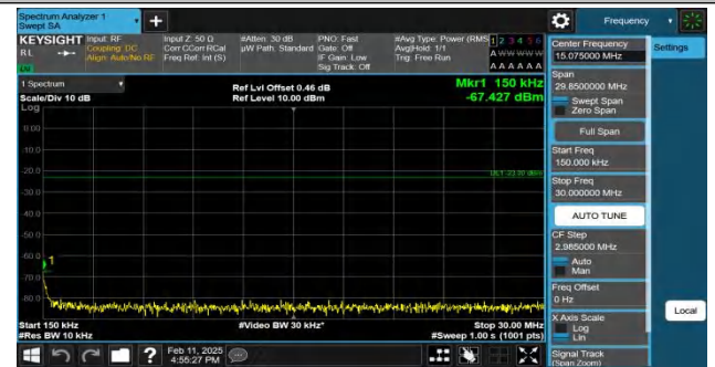
Band12-1.4MHz-QPSK-23095-1RB#0-0.15~30-PASS
