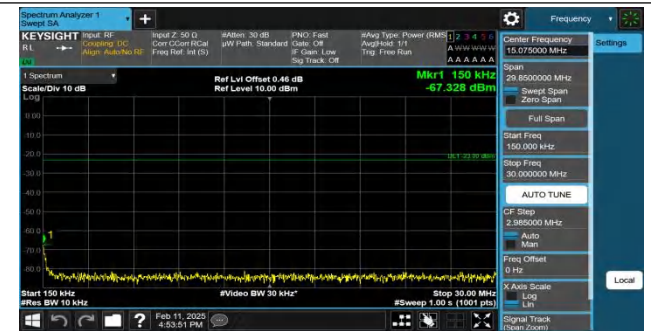
Band12-1.4MHz-QPSK-23017-1RB#0-0.15~30-PASS
