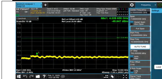
Band12-1.4MHz-QPSK-23173-1RB#0-3000~10000-PASS
