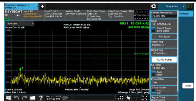
Band12-1.4MHz-QPSK-23173-1RB#5-0.009~0.15-PASS
