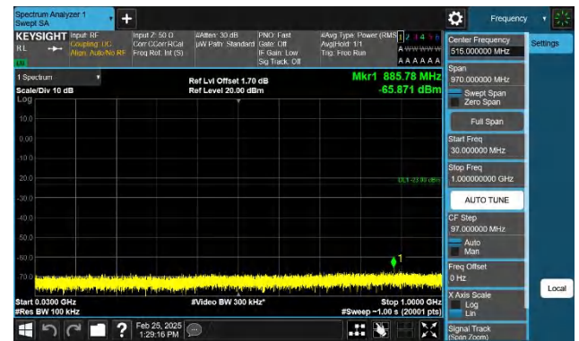
Band66-10MHz-QPSK-132322-1RB#49-30~1000-PASS
