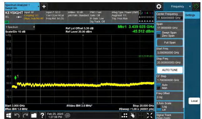
Band66-10MHz-QPSK-132022-1RB#49-3000~20000-PASS
