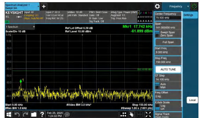
Band66-5MHz-QPSK-132322-1RB#24-0.009~0.15-PASS
