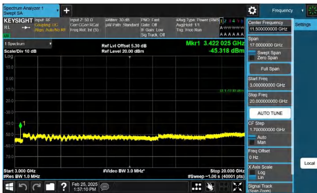
Band66-20MHz-QPSK-132072-1RB#0-3000~20000-PASS
