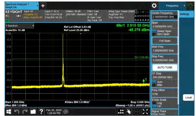
Band66-10MHz-QPSK-132322-1RB#0-1000~3000-PASS
