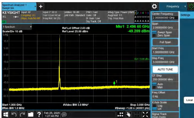
Band66-10MHz-QPSK-132022-1RB#49-1000~3000-PASS
