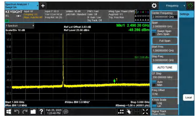
Band66-5MHz-QPSK-132322-1RB#0-1000~3000-PASS
