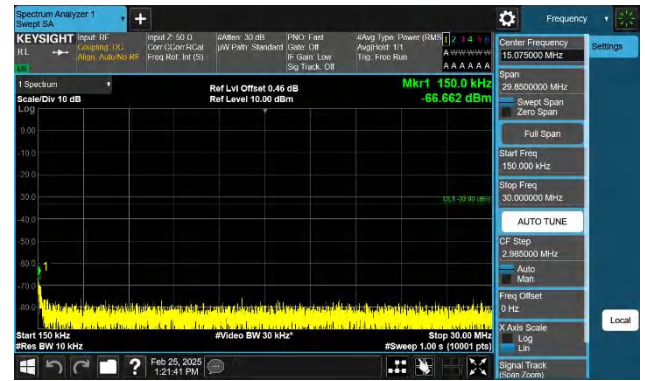
Band66-5MHz-QPSK-131997-1RB#0-0.15~30-PASS
