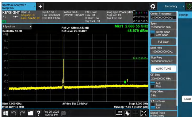
Band66-5MHz-QPSK-132647-1RB#24-1000~3000-PASS
