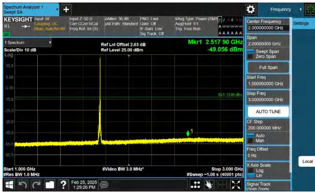
Band66-10MHz-QPSK-132322-1RB#49-1000~3000-PASS
