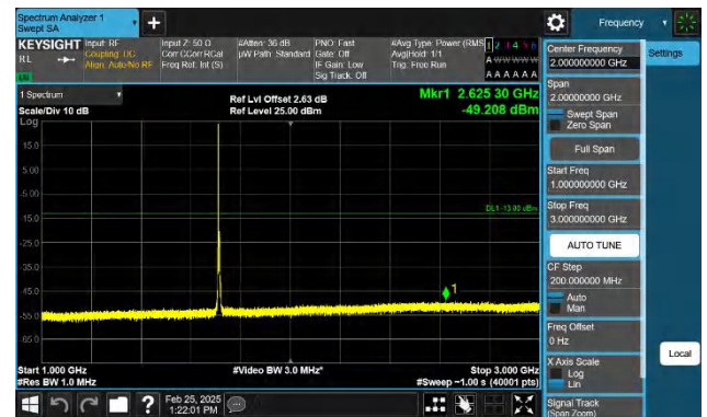
Band66-5MHz-QPSK-131997-1RB#0-1000~3000-PASS
