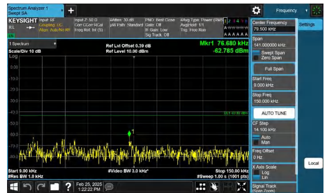
Band66-5MHz-QPSK-131997-1RB#24-0.009~0.15-PASS
