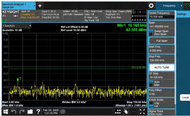
Band66-5MHz-QPSK-131997-1RB#0-0.009~0.15-PASS
