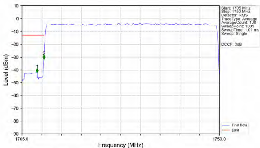
n66 15kHz MIMO NTNV 40MHz DFT-s-OFDM QPSK 1730MHz Outer Full Ant2
