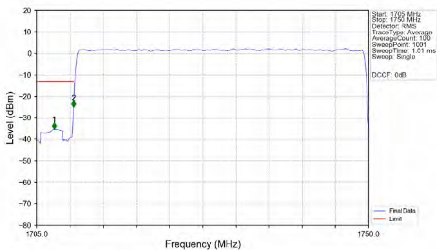
n66 15kHz MIMO NTNV 40MHz DFT-s-OFDM QPSK 1730MHz Outer Full MIMO
