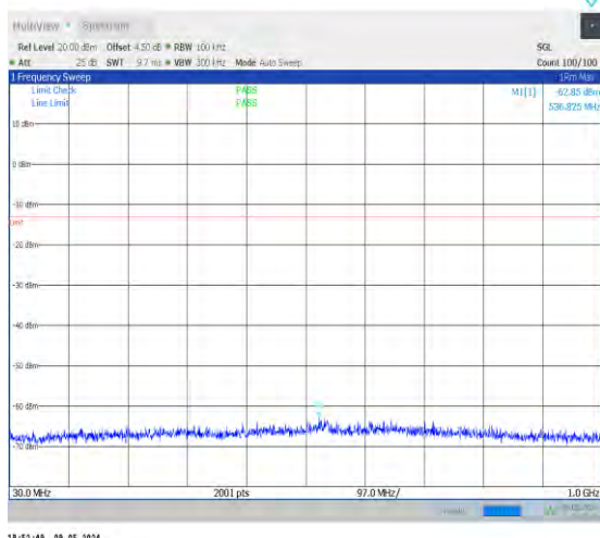
1-N78-3700-3800-PC2-30-100-M-1-DFT-PI2BPSK-Inner_1RB_Left-1@1-30-1000-Ant0-536.83--62.85--1 3-PASS
