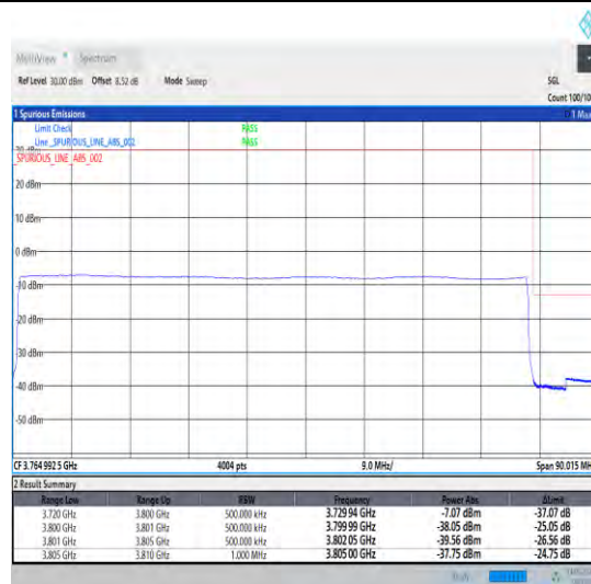
1-N78-3700-3800-30-80-H-6-CP-QPSK-Outer_Full -217@0-Ant0-1--PASS-see graph
