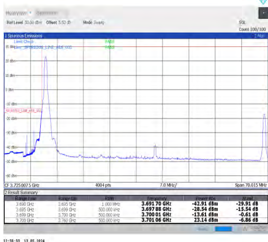
1-N78-3700-3800-PC2-30-60-L-4-CP-QPSK-Edge_1RB_Left-1@0-Ant0-1--PASS-see graph
