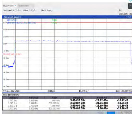
1-N78-3700-3800-PC2-30-100-L-3-DFT-PI2BPSK-Outer_Full-270@0-Ant0-1--PASS-see graph
