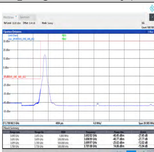
1-N78-3700-3800-30-30-L-4-CP-QPSK-Edge_1RB_Lef t-1@0-Ant0-1--PASS-see graph
