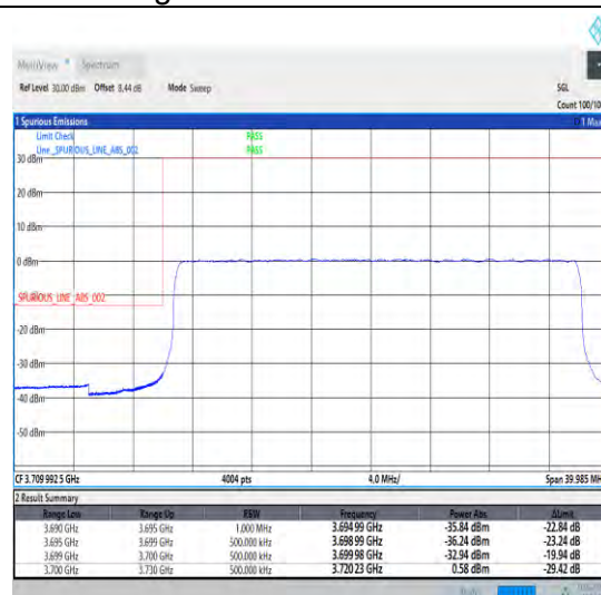
1-N78-3700-3800-30-30-L-3-DFT-PI2BPSK-Outer _Full-75@0-Ant0-1--PASS-see graph
