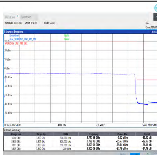
1-N78-3700-3800-30-60-H-6-CP-QPSK-Outer_Full -162@0-Ant0-1--PASS-see graph
