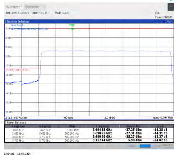
1-N78-3700-3800-PC2-30-40-L-6-CP-QPSK-Outer_Full-106@0-Ant0-1--PASS-see graph
