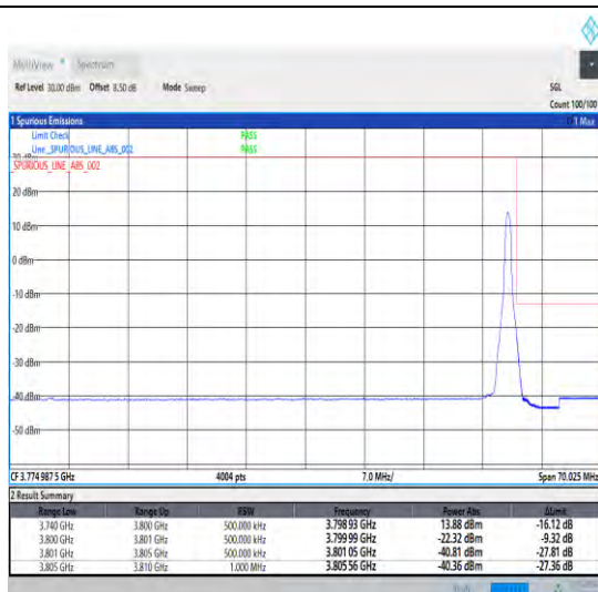
1-N78-3700-3800-30-60-H-2-DFT-PI2BPSK-Edge_1R B_Right-1@161-Ant0-1--PASS-see graph
