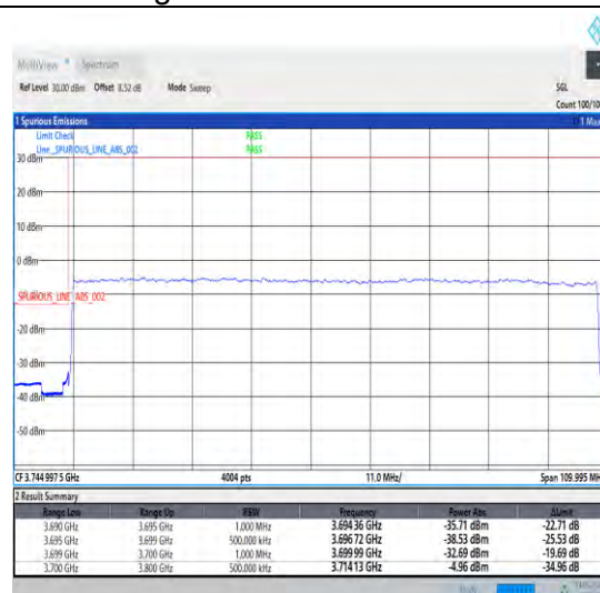
1-N78-3700-3800-30-100-L-3-DFT-PI2BPSK-Outer_Full-270@0-Ant0-1--PASS-see graph
