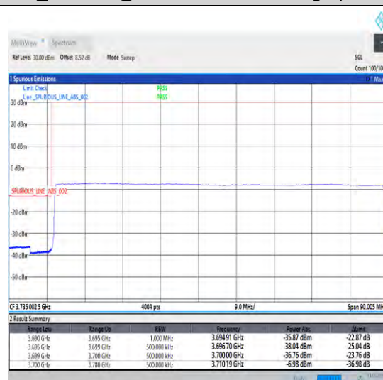
1-N78-3700-3800-30-80-L-6-CP-QPSK-Outer_Full -217@0-Ant0-1--PASS-see graph
