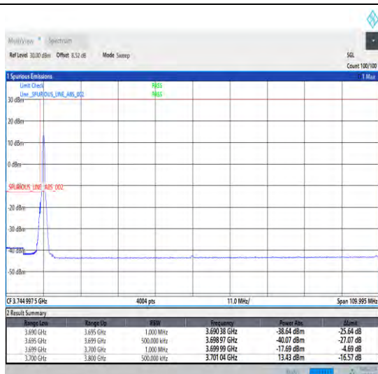
1-N78-3700-3800-30-100-L-1-DFT-PI2BPSK-Edge_1R_B_Left-1@0-Ant0-1--PASS-see graph
