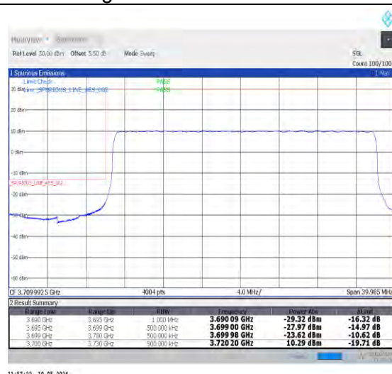
1-N78-3700-3800-PC2-30-30-L-3-DFT-PI2BPSK-Outer_Full-75@0-Ant0-1--PASS-see graph
