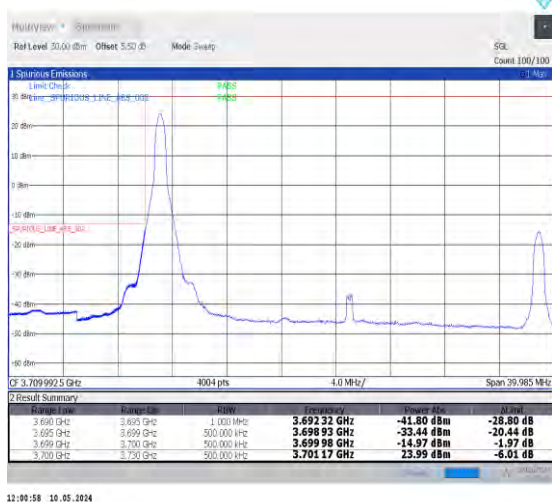
1-N78-3700-3800-PC2-30-30-L-4-CP-QPSK-Edge_1RB_Left-1@0-Ant0-1--PASS-see graph
