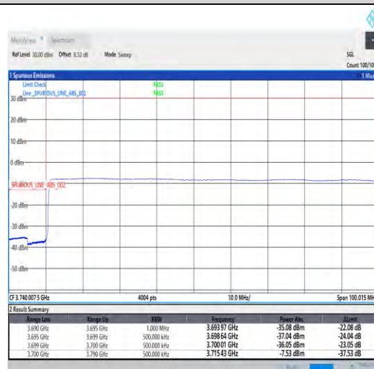
1-N78-3700-3800-30-90-L-6-CP-QPSK-Outer_Full -245@0-Ant0-1--PASS-see graph
