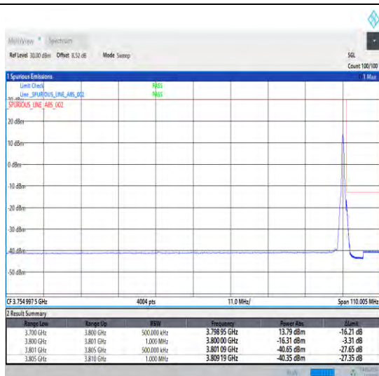
1-N78-3700-3800-30-100-H-2-DFT-PI2BPSK-Edge_1R_B_Right-1@272-Ant0-1--PASS-see graph
