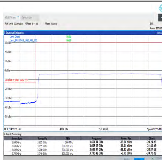
1-N78-3700-3800-30-40-L-6-CP-QPSK-Outer_Full -106@0-Ant0-1--PASS-see graph
