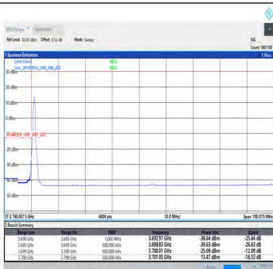
1-N78-3700-3800-30-90-L-1-DFT-PI2BPSK-Edge_1RB _Left-1@0-Ant0-1--PASS-see graph
