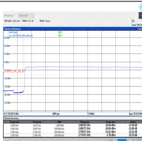
1-N78-3700-3800-30-60-L-6-CP-QPSK-Outer_Full -162@0-Ant0-1--PASS-see graph
