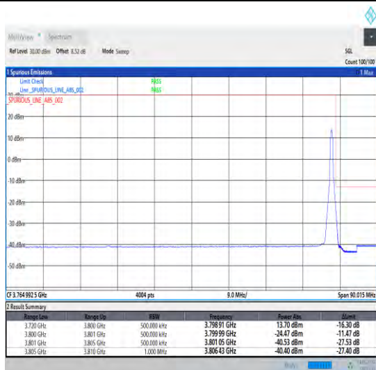
1-N78-3700-3800-30-80-H-5-CP-QPSK-Edge_1RB_Ri ght-1@216-Ant0-1--PASS-see graph
