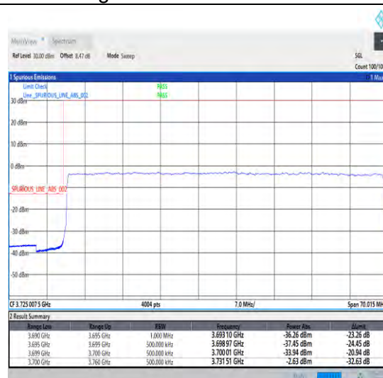
1-N78-3700-3800-30-60-L-3-DFT-PI2BPSK-Outer _Full-162@0-Ant0-1--PASS-see graph
