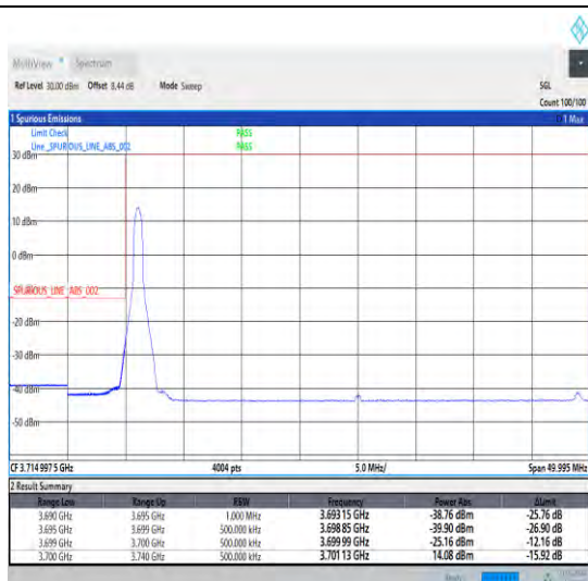
1-N78-3700-3800-30-40-L-1-DFT-PI2BPSK-Edge_1RB _Left-1@0-Ant0-1--PASS-see graph
