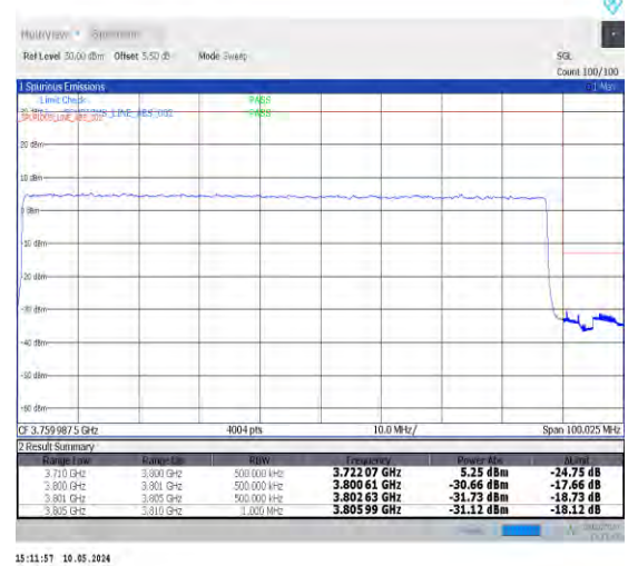
1-N78-3700-3800-PC2-30-90-H-3-DFT-PI2BPSK-Outer_Full-240@0-Ant0-1--PASS-see graph
