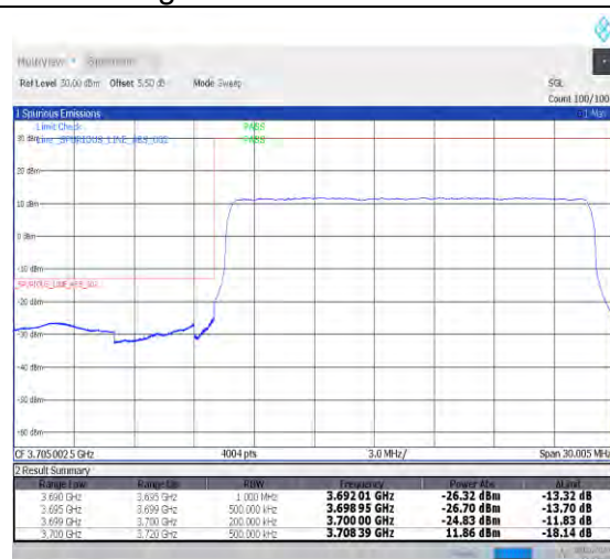
1-N78-3700-3800-PC2-30-20-L-3-DFT-PI2BPSK-Outer_Full-50@0-Ant0-1--PASS-see graph
