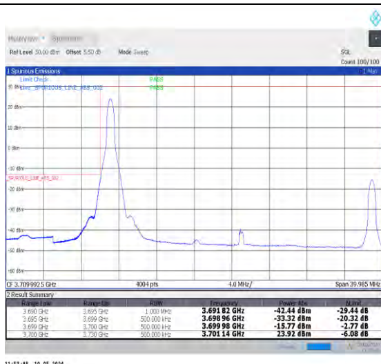
1-N78-3700-3800-PC2-30-30-L-1-DFT-PI2BPSK-Edge_1RB_Left-1@0-Ant0-1--PASS-see graph
