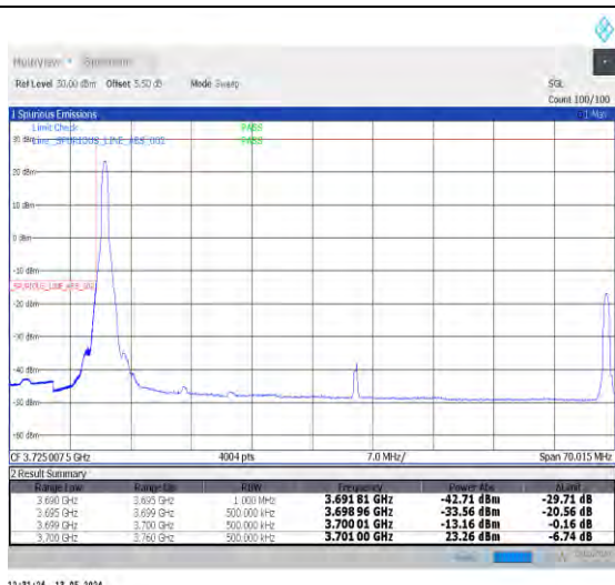
1-N78-3700-3800-PC2-30-60-L-1-DFT-PI2BPSK-Edge_1RB_Left-1@0-Ant0-1--PASS-see graph
