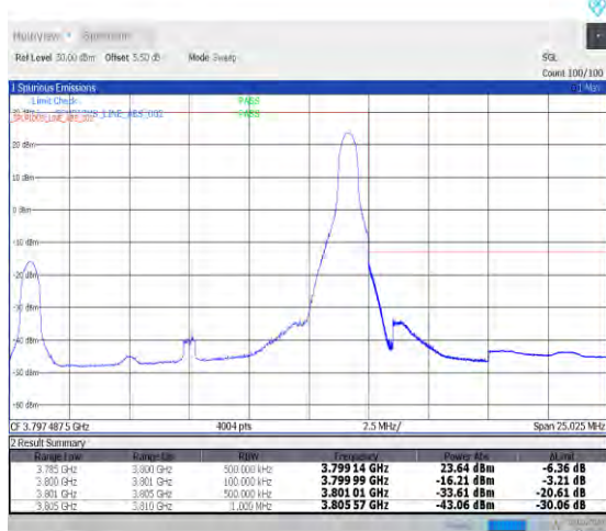
1-N78-3700-3800-PC2-30-15-H-2-DFT-PI2BPSK-Edge_1RB_Right-1@37-Ant0-1--PASS-see graph
