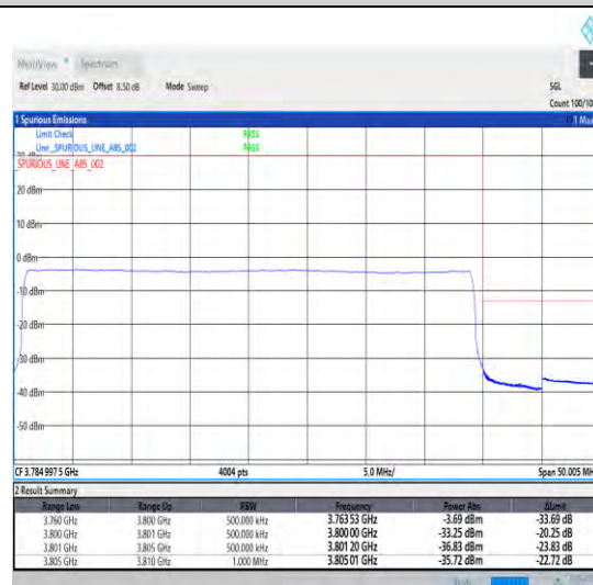
1-N78-3700-3800-30-40-H-6-CP-QPSK-Outer_Full -106@0-Ant0-1--PASS-see graph
