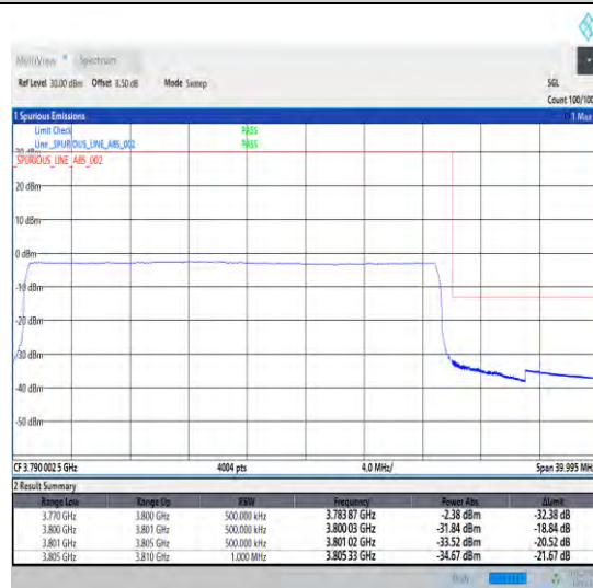
1-N78-3700-3800-30-30-H-6-CP-QPSK-Outer_Full-78@0-Ant0-1--PASS-see graph
