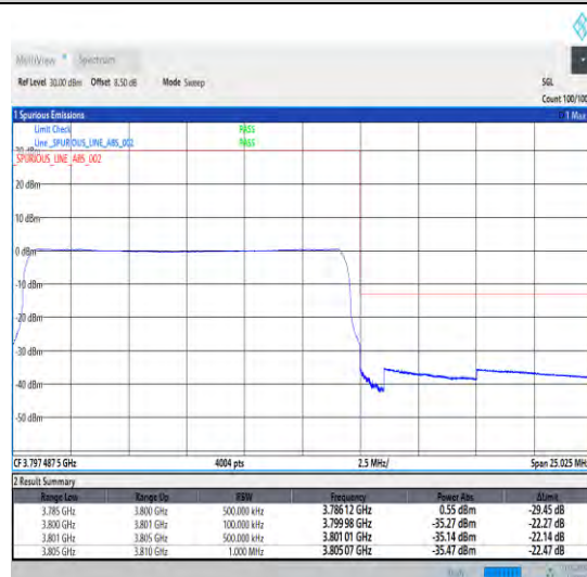
1-N78-3700-3800-30-15-H-6-CP-QPSK-Outer_Full-38@0-Ant0-1--PASS-see graph
