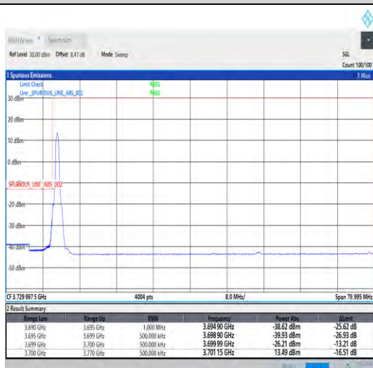
1-N78-3700-3800-30-70-L-4-CP-QPSK-Edge_1RB_Lef t-1@0-Ant0-1--PASS-see graph
