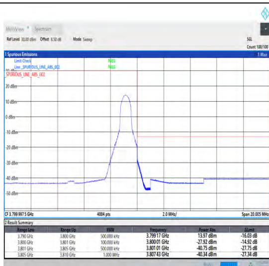
1-N78-3700-3800-30-10-H-2-DFT-PI2BPSK-Edge_1R_B_Right-1@23-Ant0-1--PASS-see graph
