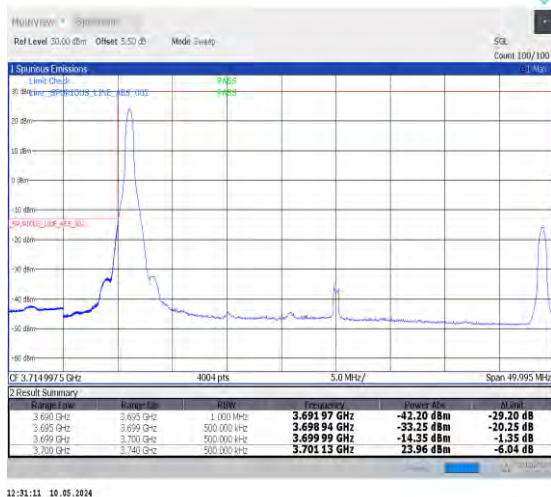
1-N78-3700-3800-PC2-30-40-L-4-CP-QPSK-Edge_1RB_Left-1@0-Ant0-1--PASS-see graph
