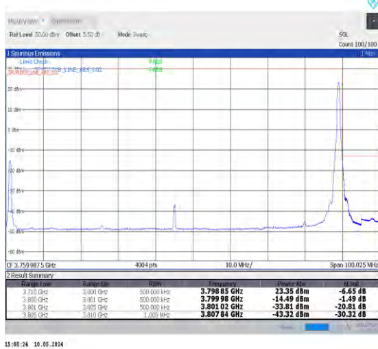
1-N78-3700-3800-PC2-30-90-H-2-DFT-PI2BPSK-Edge_1RB_Right-1@244-Ant0-1--PASS-see graph
