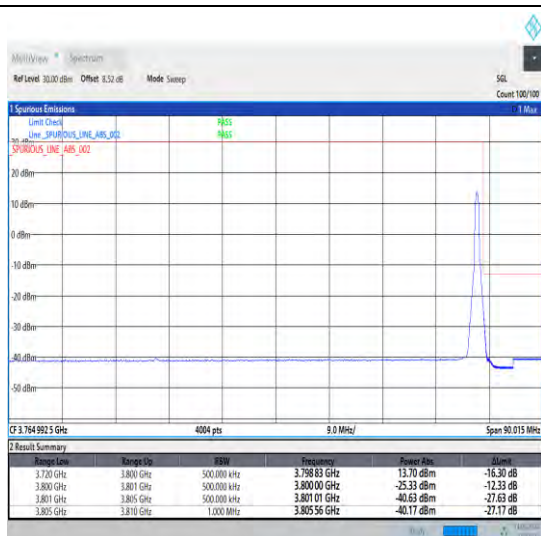
1-N78-3700-3800-30-80-H-2-DFT-PI2BPSK-Edge_1R B_Right-1@216-Ant0-1--PASS-see graph
