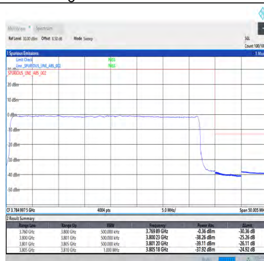
1-N78-3700-3800-30-40-H-3-DFT-PI2BPSK-Outer _Full-100@0-Ant0-1--PASS-see graph
