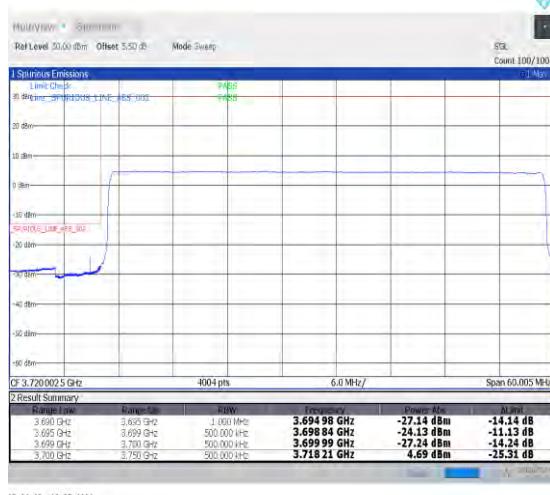
1-N78-3700-3800-PC2-30-50-L-6-CP-QPSK-Outer_Full-133@0-Ant0-1--PASS-see graph
