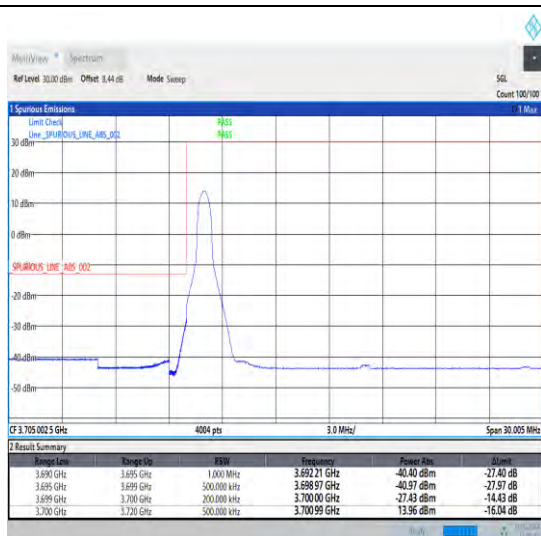
1-N78-3700-3800-30-20-L-1-DFT-PI2BPSK-Edge_1RB _Left-1@0-Ant0-1--PASS-see graph
