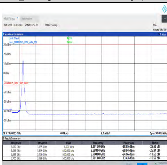
1-N78-3700-3800-30-80-L-4-CP-QPSK-Edge_1RB_Lef t-1@0-Ant0-1--PASS-see graph
