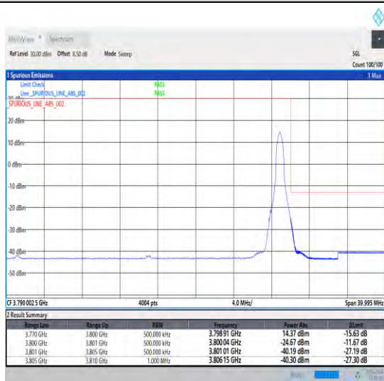
1-N78-3700-3800-30-30-H-5-CP-QPSK-Edge_1RB_Right-1@77-Ant0-1--PASS-see graph
