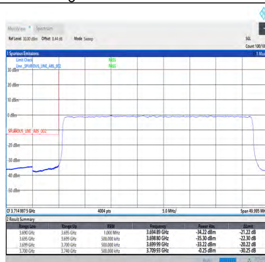
1-N78-3700-3800-30-40-L-3-DFT-PI2BPSK-Outer _Full-100@0-Ant0-1--PASS-see graph
