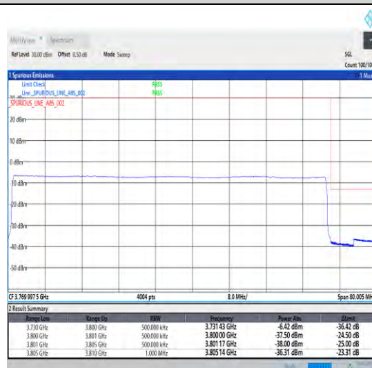
1-N78-3700-3800-30-70-H-6-CP-QPSK-Outer_Full -189@0-Ant0-1--PASS-see graph
