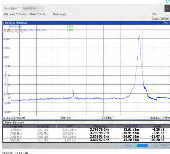
1-N78-3700-3800-PC2-30-50-H-5-CP-QPSK-Edge_1R B_Right-1@132-Ant0-1--PASS-see graph
