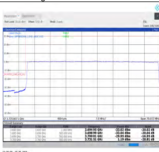
1-N78-3700-3800-PC2-30-60-L-3-DFT-PI2BPSK-Outer_Full-162@0-Ant0-1--PASS-see graph
