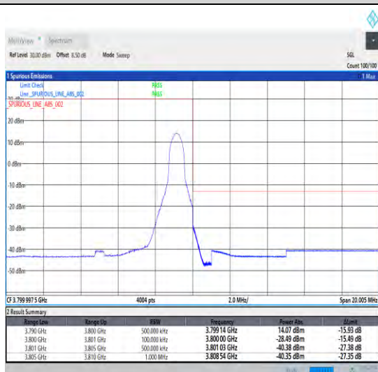
1-N78-3700-3800-30-10-H-5-CP-QPSK-Edge_1RB_Right-1@23-Ant0-1--PASS-see graph
