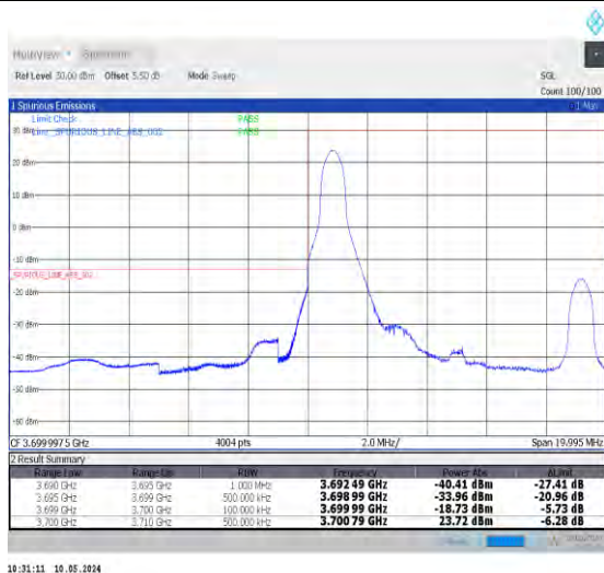
1-N78-3700-3800-PC2-30-10-L-4-CP-QPSK-Edge_1RB_Left-1@0-Ant0-1--PASS-see graph
