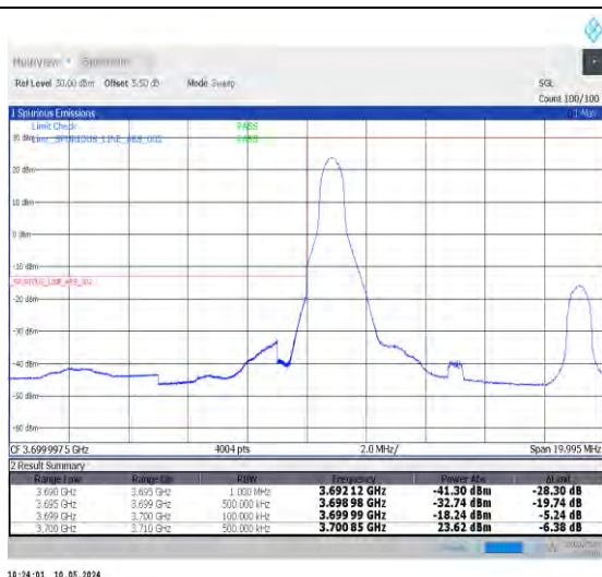
1-N78-3700-3800-PC2-30-10-L-1-DFT-PI2BPSK-Edge_1RB_Left-1@0-Ant0-1--PASS-see graph
