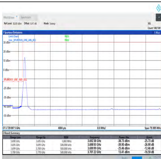
1-N78-3700-3800-30-70-L-1-DFT-PI2BPSK-Edge_1RB _Left-1@0-Ant0-1--PASS-see graph
