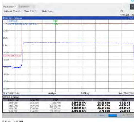
1-N78-3700-3800-PC2-30-60-L-6-CP-QPSK-Outer_Full-162@0-Ant0-1--PASS-see graph
