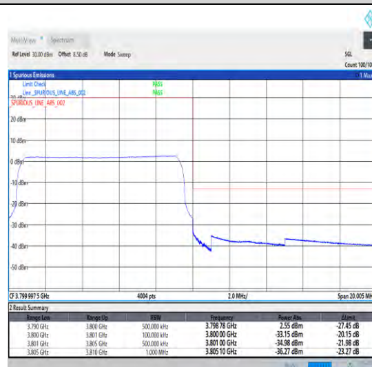
1-N78-3700-3800-30-10-H-6-CP-QPSK-Outer_Full-24@0-Ant0-1--PASS-see graph
