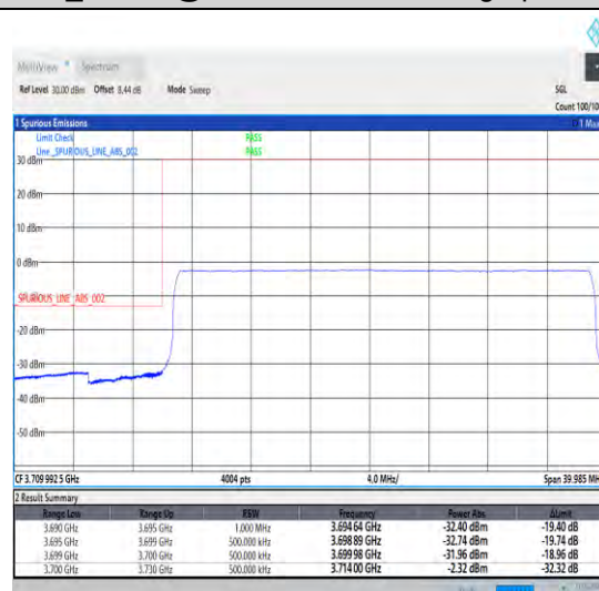
1-N78-3700-3800-30-30-L-6-CP-QPSK-Outer_Full -78@0-Ant0-1--PASS-see graph
