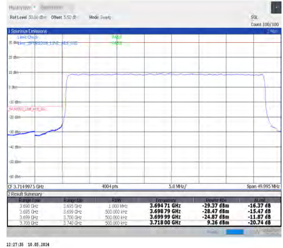
1-N78-3700-3800-PC2-30-40-L-3-DFT-PI2BPSK-Outer_Full-100@0-Ant0-1--PASS-see graph
