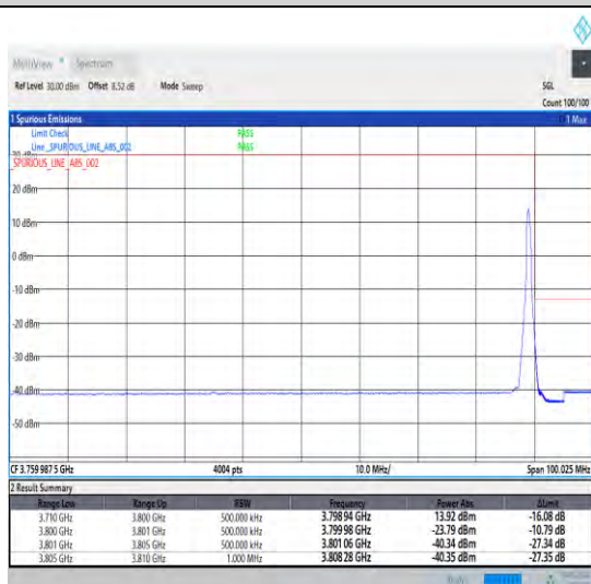
1-N78-3700-3800-30-90-H-5-CP-QPSK-Edge_1RB_Ri ght-1@244-Ant0-1--PASS-see graph
