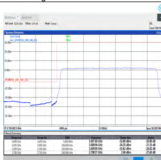
1-N78-3700-3800-30-20-L-3-DFT-PI2BPSK-Outer _Full-50@0-Ant0-1--PASS-see graph
