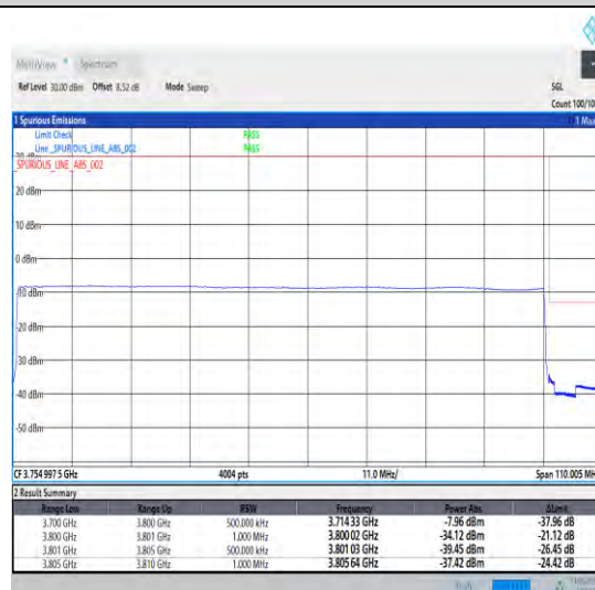
1-N78-3700-3800-30-100-H-6-CP-QPSK-Outer_Full-273@0-Ant0-1--PASS-see graph
