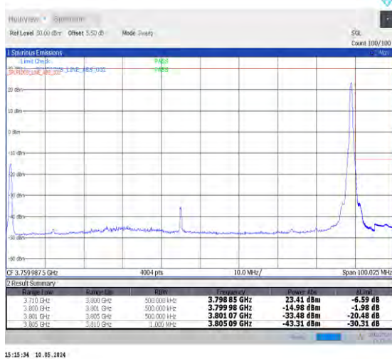
1-N78-3700-3800-PC2-30-90-H-5-CP-QPSK-Edge_1RB_Right-1@244-Ant0-1--PASS-see graph
