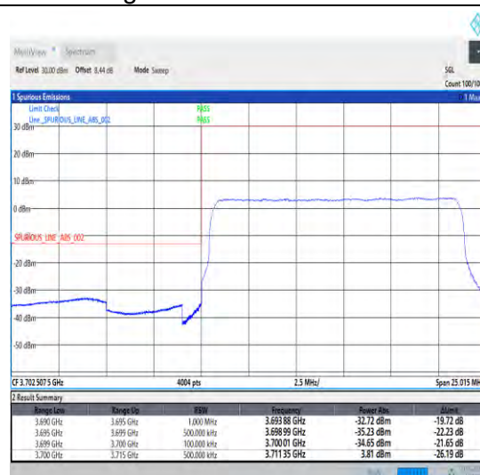
1-N78-3700-3800-30-15-L-3-DFT-PI2BPSK-Outer _Full-36@0-Ant0-1--PASS-see graph
