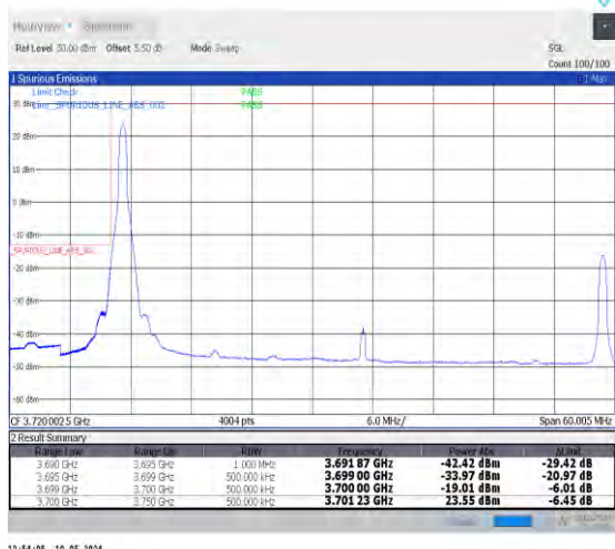
1-N78-3700-3800-PC2-30-50-L-1-DFT-PI2BPSK-Edge_1RB_Left-1@0-Ant0-1--PASS-see graph
