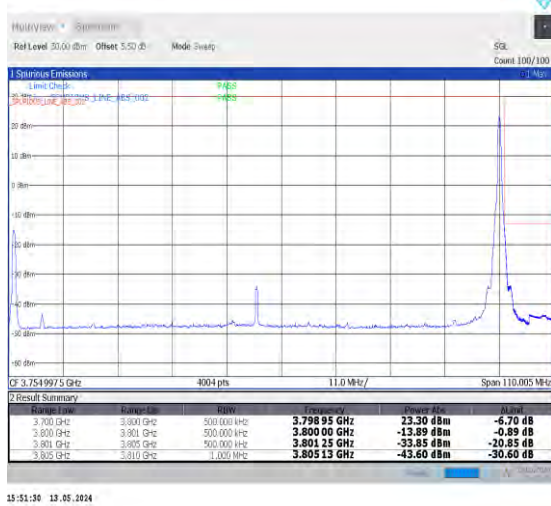
1-N78-3700-3800-PC2-30-100-H-5-CP-QPSK-Edge_1RB_Right-1@272-Ant0-1--PASS-see graph
