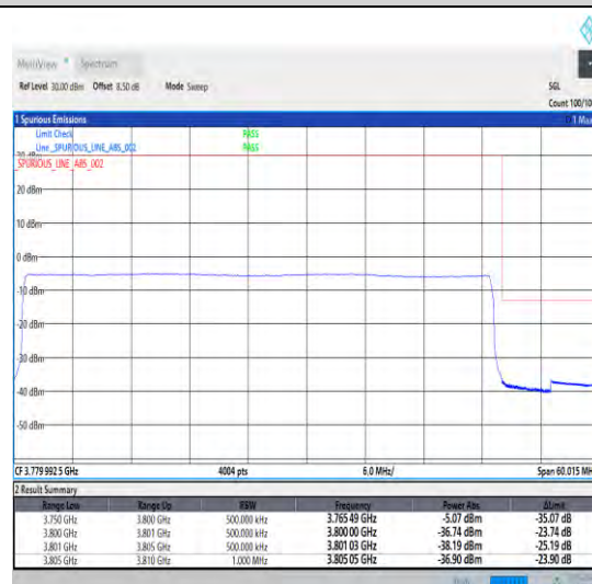
1-N78-3700-3800-30-50-H-6-CP-QPSK-Outer_Full -133@0-Ant0-1--PASS-see graph
