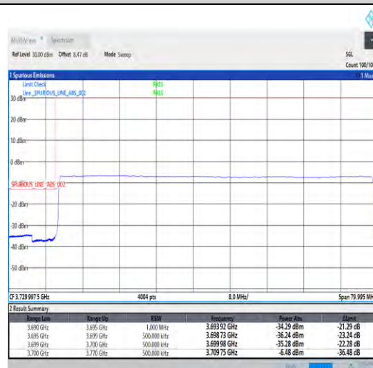
1-N78-3700-3800-30-70-L-6-CP-QPSK-Outer_Full -189@0-Ant0-1--PASS-see graph
