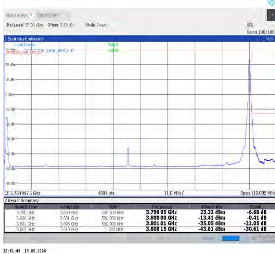
1-N78-3700-3800-PC2-30-100-H-2-DFT-PI2BPSK-Edge_1RB_Right-1@272-Ant0-1--PASS-see graph
