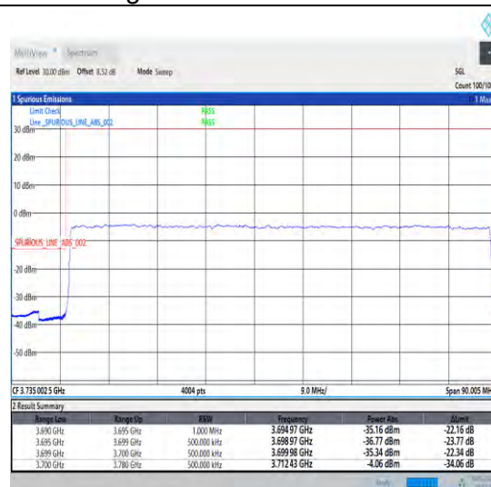
1-N78-3700-3800-30-80-L-3-DFT-PI2BPSK-Outer _Full-216@0-Ant0-1--PASS-see graph
