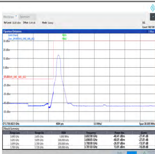
1-N78-3700-3800-30-20-L-4-CP-QPSK-Edge_1RB_Lef t-1@0-Ant0-1--PASS-see graph
