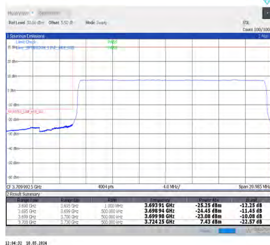
1-N78-3700-3800-PC2-30-30-L-6-CP-QPSK-Outer_Full-78@0-Ant0-1--PASS-see graph
