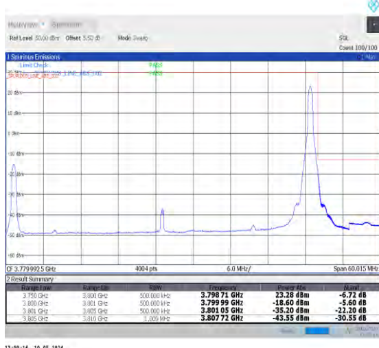
1-N78-3700-3800-PC2-30-50-H-2-DFT-PI2BPSK-Edge _1RB_Right-1@132-Ant0-1--PASS-see graph
