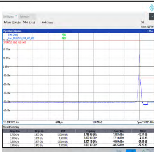
1-N78-3700-3800-30-100-H-5-CP-QPSK-Edge_1RB_Right-1@272-Ant0-1--PASS-see graph
