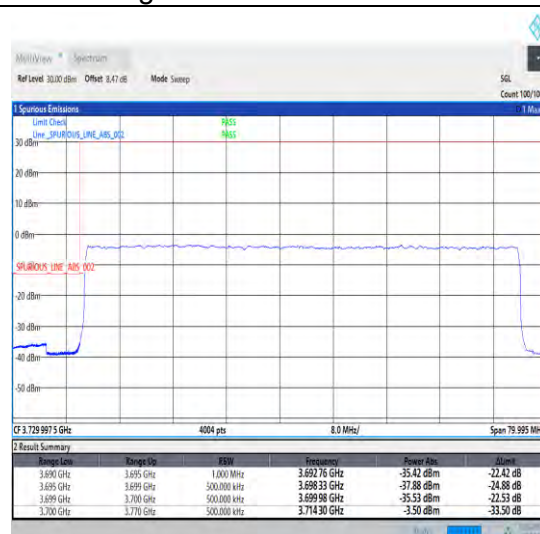
1-N78-3700-3800-30-70-L-3-DFT-PI2BPSK-Outer _Full-180@0-Ant0-1--PASS-see graph
