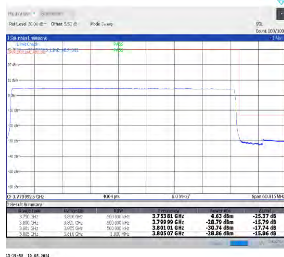
1-N78-3700-3800-PC2-30-50-H-6-CP-QPSK-Outer _Full-133@0-Ant0-1--PASS-see graph
