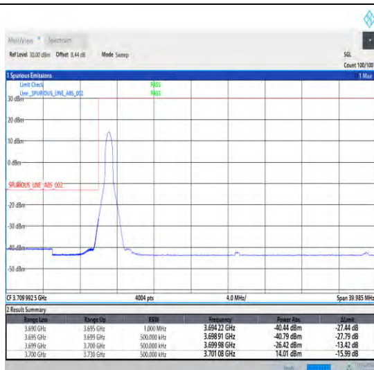
1-N78-3700-3800-30-30-L-1-DFT-PI2BPSK-Edge_1RB _Left-1@0-Ant0-1--PASS-see graph
