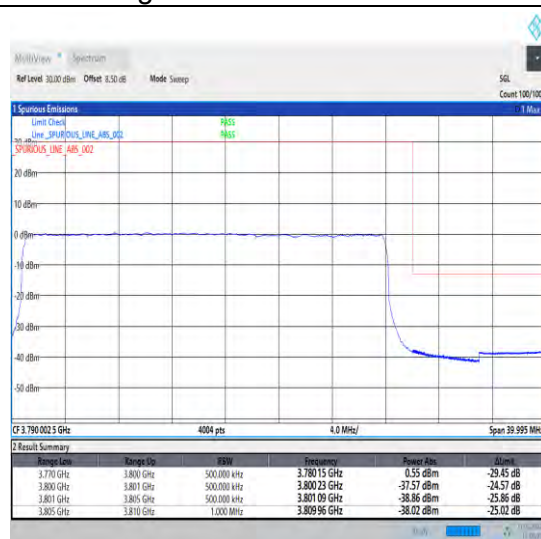
1-N78-3700-3800-30-30-H-3-DFT-PI2BPSK-Outer_Full-75@0-Ant0-1--PASS-see graph
