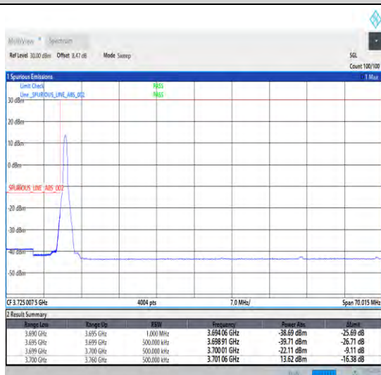
1-N78-3700-3800-30-60-L-4-CP-QPSK-Edge_1RB_Lef t-1@0-Ant0-1--PASS-see graph
