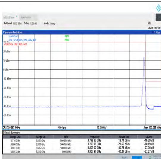
1-N78-3700-3800-30-90-H-2-DFT-PI2BPSK-Edge_1R B_Right-1@244-Ant0-1--PASS-see graph
