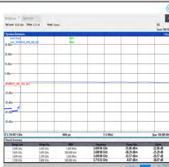
1-N78-3700-3800-30-100-L-6-CP-QPSK-Outer_Full-273@0-Ant0-1--PASS-see graph
