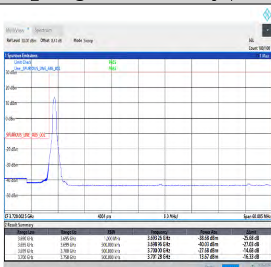
1-N78-3700-3800-30-50-L-4-CP-QPSK-Edge_1RB_Lef t-1@0-Ant0-1--PASS-see graph
