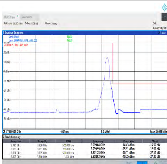
1-N78-3700-3800-30-20-H-5-CP-QPSK-Edge_1RB_Right-1@50-Ant0-1--PASS-see graph
