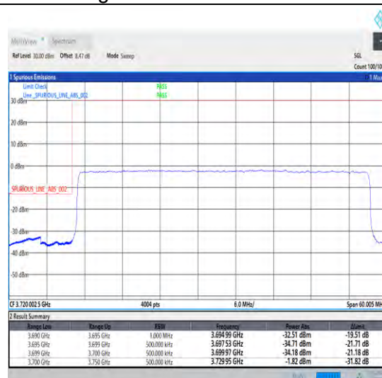
1-N78-3700-3800-30-50-L-3-DFT-PI2BPSK-Outer _Full-128@0-Ant0-1--PASS-see graph
