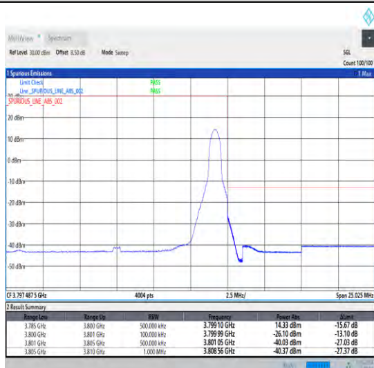
1-N78-3700-3800-30-15-H-5-CP-QPSK-Edge_1RB_Right-1@37-Ant0-1--PASS-see graph
