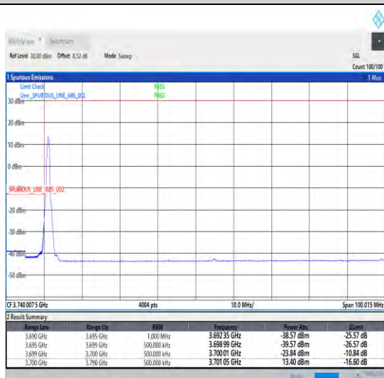
1-N78-3700-3800-30-90-L-4-CP-QPSK-Edge_1RB_Lef t-1@0-Ant0-1--PASS-see graph
