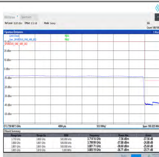
1-N78-3700-3800-30-90-H-6-CP-QPSK-Outer_Full -245@0-Ant0-1--PASS-see graph
