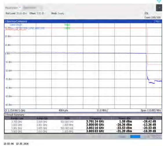
1-N78-3700-3800-PC2-30-100-H-6-CP-QPSK-Outer_Full-273@0-Ant0-1--PASS-see graph
