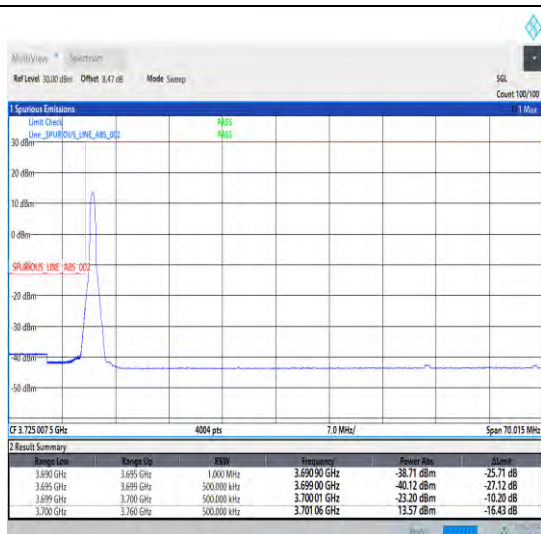
1-N78-3700-3800-30-60-L-1-DFT-PI2BPSK-Edge_1RB _Left-1@0-Ant0-1--PASS-see graph
