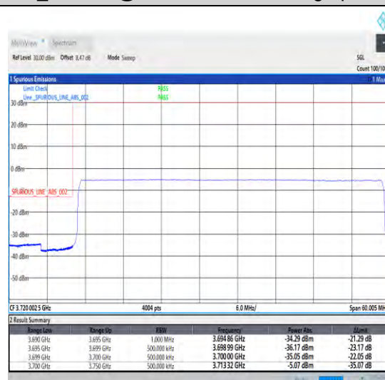
1-N78-3700-3800-30-50-L-6-CP-QPSK-Outer_Full -133@0-Ant0-1--PASS-see graph
