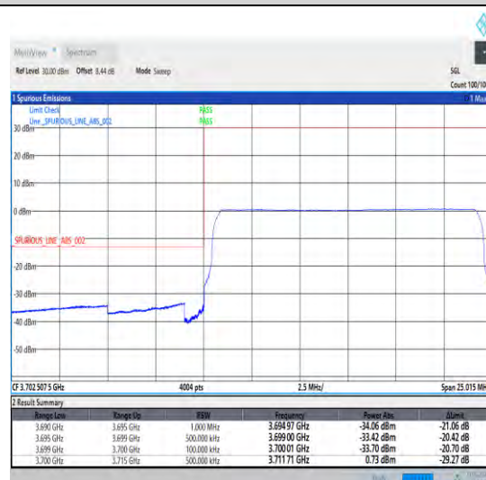
1-N78-3700-3800-30-15-L-6-CP-QPSK-Outer_Full -38@0-Ant0-1--PASS-see graph
