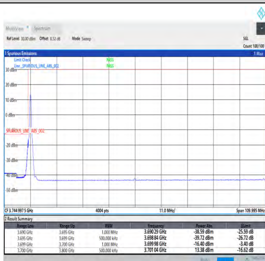
1-N78-3700-3800-30-100-L-4-CP-QPSK-Edge_1RB_Left-1@0-Ant0-1--PASS-see graph
