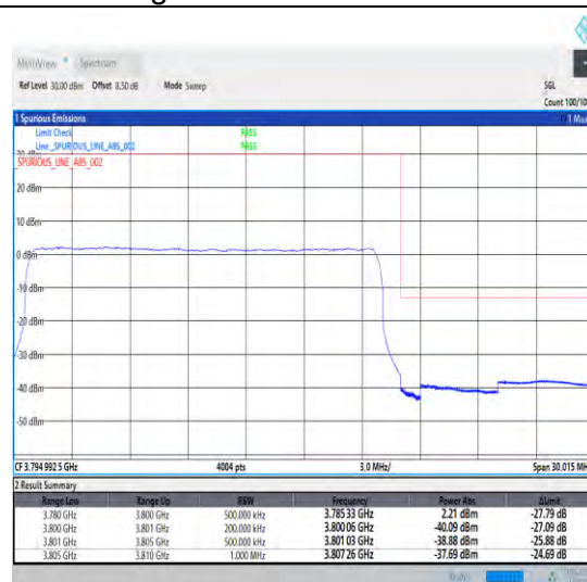
1-N78-3700-3800-30-20-H-3-DFT-PI2BPSK-Outer_Full-50@0-Ant0-1--PASS-see graph
