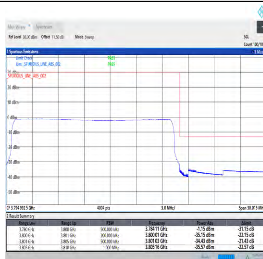
1-N78-3700-3800-30-20-H-6-CP-QPSK-Outer_Full-51@0-Ant0-1--PASS-see graph
