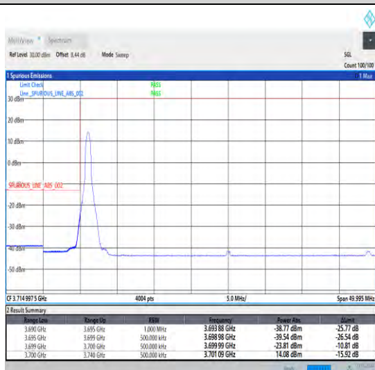
1-N78-3700-3800-30-40-L-4-CP-QPSK-Edge_1RB_Lef t-1@0-Ant0-1--PASS-see graph
