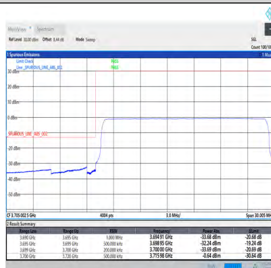
1-N78-3700-3800-30-20-L-6-CP-QPSK-Outer_Full -51@0-Ant0-1--PASS-see graph
