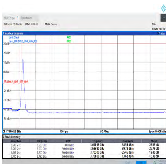
1-N78-3700-3800-30-80-L-1-DFT-PI2BPSK-Edge_1RB _Left-1@0-Ant0-1--PASS-see graph
