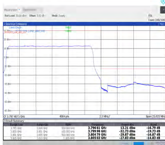
1-N78-3700-3800-PC2-30-15-H-3-DFT-PI2BPSK-Outer_Full-36@0-Ant0-1--PASS-see graph
