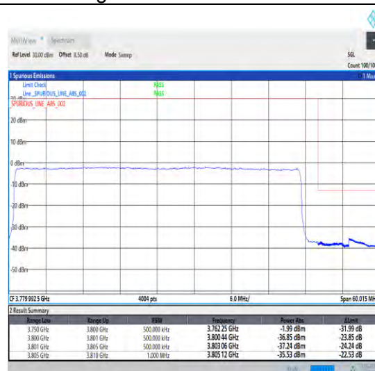
1-N78-3700-3800-30-50-H-3-DFT-PI2BPSK-Outer _Full-128@0-Ant0-1--PASS-see graph
