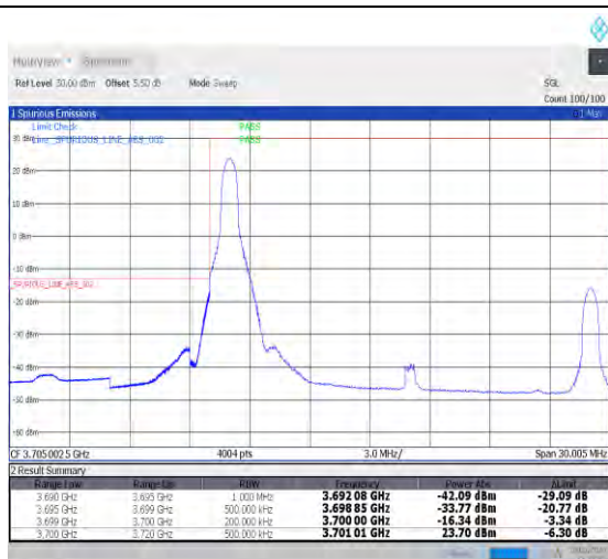
1-N78-3700-3800-PC2-30-20-L-1-DFT-PI2BPSK-Edge_1RB_Left-1@0-Ant0-1--PASS-see graph
