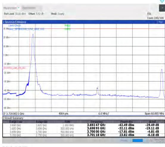
1-N78-3700-3800-PC2-30-50-L-4-CP-QPSK-Edge_1RB_Left-1@0-Ant0-1--PASS-see graph
