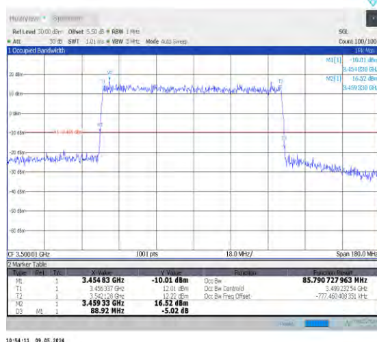
1-N78-3450-3550-PC2-30-90-M-3-DFT-16QAM-Outer_Full-240@0-Ant0-85.791-88.920-≤90-PASS
