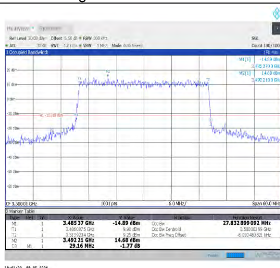
1-N78-3450-3550-PC2-30-30-M-7-CP-16QAM-Out-er_Full-78@0-Ant0-27.815-29.160-≤30-PASS
