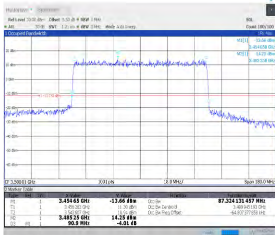
1-N78-3450-3550-PC2-30-90-M-8-CP-64QAM-Outer_Full-245@0-Ant0-87.324-90.900-≤90-PASS
