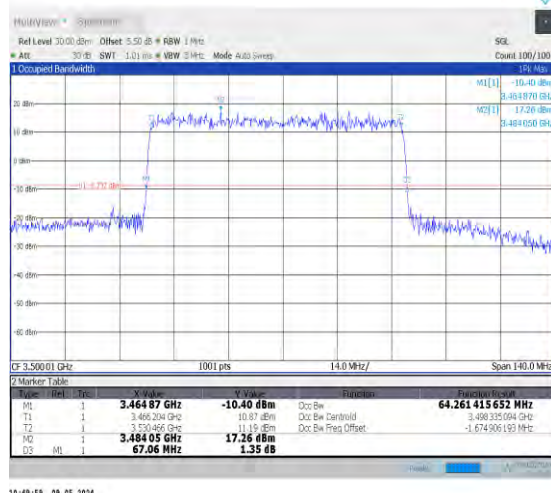
1-N78-3450-3550-PC2-30-70-M-3-DFT-16QAM-Outer_Full-180@0-Ant0-64.261-67.060-≤70-PASS
