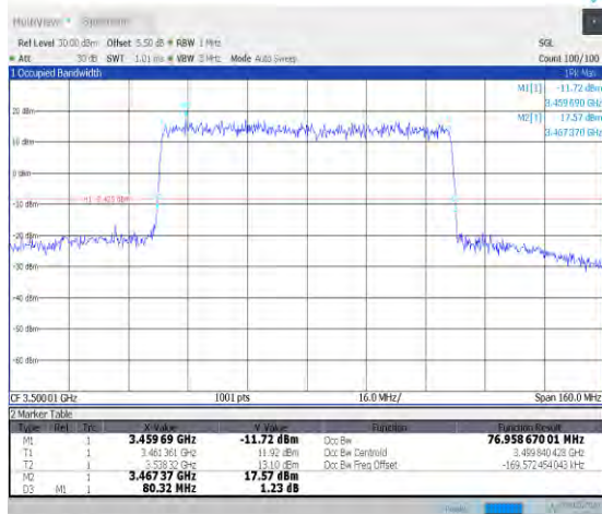
1-N78-3450-3550-PC2-30-80-M-1-DFT-QPSK-Outer_Full-216@0-Ant0-76.959-80.320-≤80-PASS
