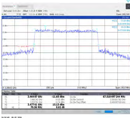
1-N78-3450-3550-PC2-30-70-M-8-CP-64QAM-Outer_Full-189@0-Ant0-67.518-70.560-≤70-PASS
