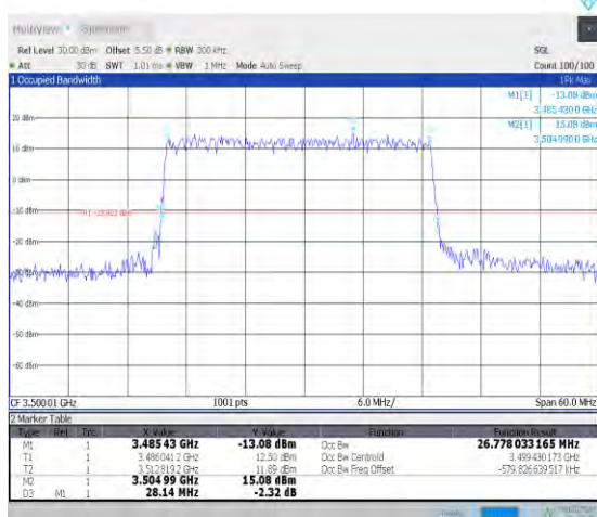
1-N78-3450-3550-PC2-30-30-M-4-DFT-64QAM-Outer_Full-75@0-Ant0-26.78-28.140-≤30-PASS
