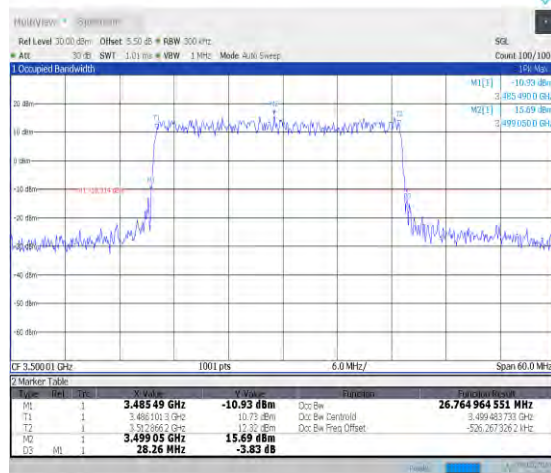
1-N78-3450-3550-PC2-30-30-M-3-DFT-16QAM-Outer_Full-75@0-Ant0-26.765-28.260-≤30-PASS
