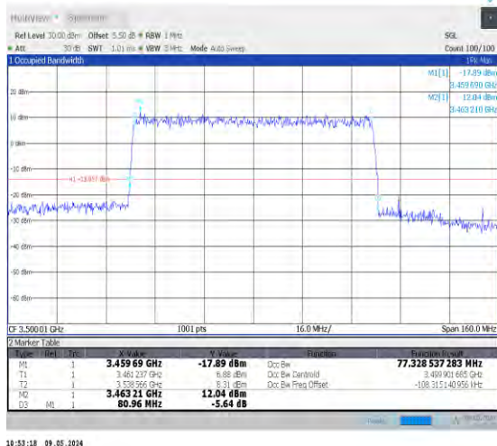
1-N78-3450-3550-PC2-30-80-M-9-CP-256QAM-Out_er_Full-217@0-Ant0-77.329-80.960-≤80-PASS
