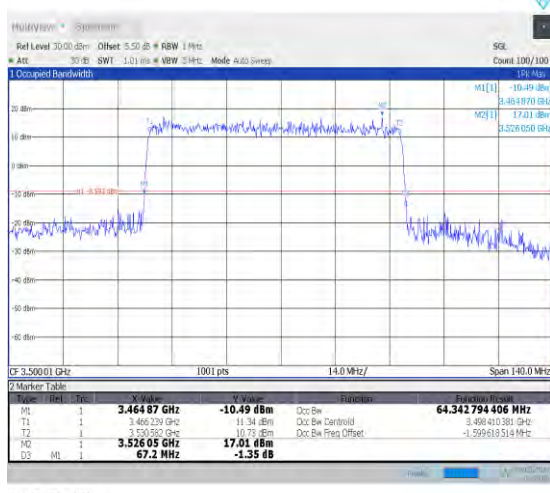
1-N78-3450-3550-PC2-30-70-M-4-DFT-64QAM-Outer_Full-180@0-Ant0-64.343-67.200-≤70-PASS
