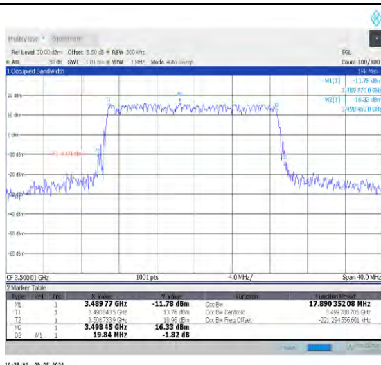
1-N78-3450-3550-PC2-30-20-M-3-DFT-16QAM-Out er_Full-50@0-Ant0-17.89-19.840-≤20-PASS
