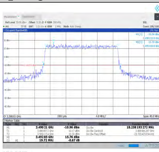
1-N78-3450-3550-PC2-30-20-M-6-CP-QPSK-Out er_Full-51@0-Ant0-18.258-19.720-≤20-PASS
