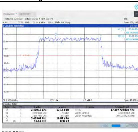
1-N78-3450-3550-PC2-30-20-M-4-DFT-64QAM-Out er_Full-50@0-Ant0-17.898-19.040-≤20-PASS
