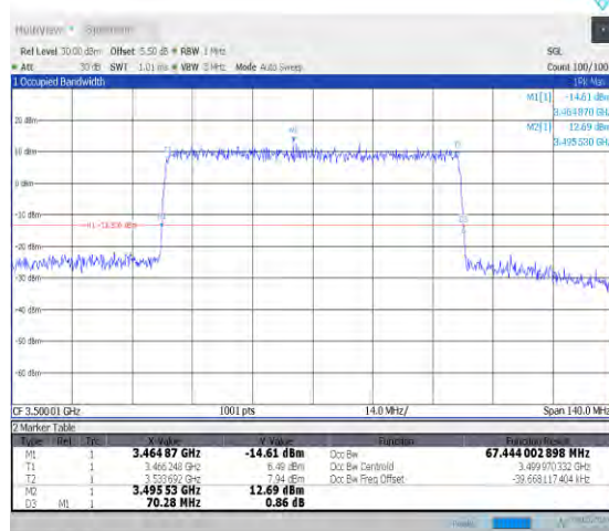
1-N78-3450-3550-PC2-30-70-M-9-CP-256QAM-Outer_Full-189@0-Ant0-67.444-70.280-≤70-PASS
