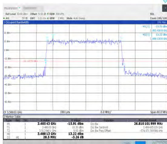
1-N78-3450-3550-PC2-30-30-M-5-DFT-256QAM-Outer_Full-75@0-Ant0-26.812-28.500-≤30-PASS
