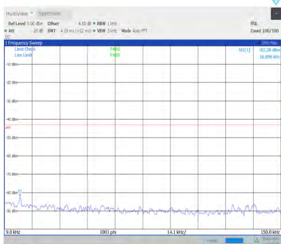
1-N2-15-20-M-1-DFT-PI2BPSK-Inner_1RB_Left-1@ 1-0.009-0.15-Ant0-0.02--82.38--43-PASS
