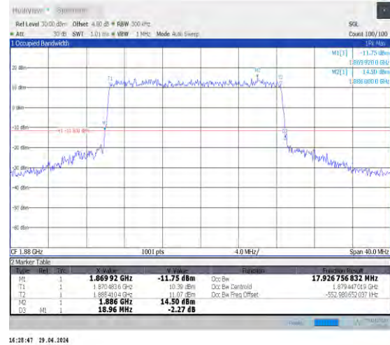
1-N2-15-20-M-3-DFT-16QAM-Outer_Full-100@0-Ant 0-17.927-18.960-≤20-PASS
