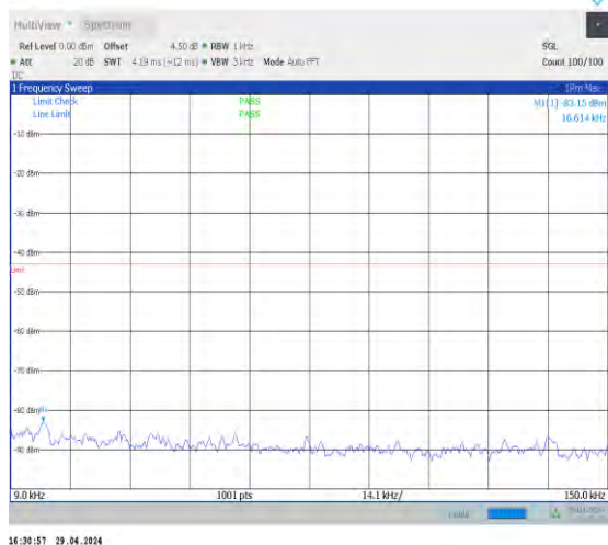
1-N2-15-20-L-1-DFT-PI2BPSK-Inner_1RB_Left-1@ 1-0.009-0.15-Ant0-0.02--83.15--43-PASS
