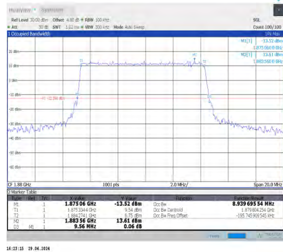
1-N2-15-10-M-1-DFT-QPSK-Outer_Full-50@0-Ant0- 8.94-9.560-≤10-PASS
