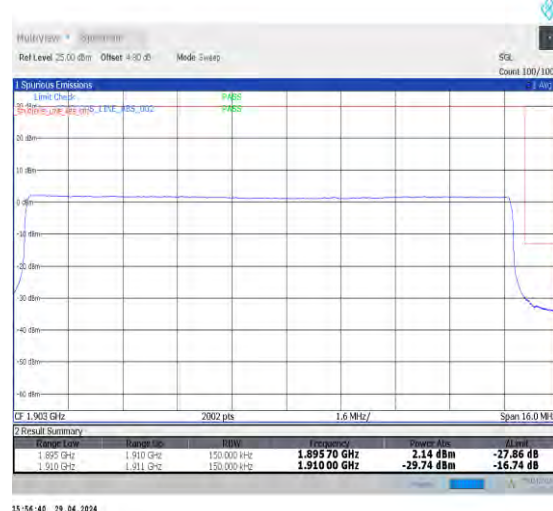
1-N2-15-15-H-6-CP-QPSK-Outer_Full-79@0-Ant0-1-seegraph-PASS-see graph
