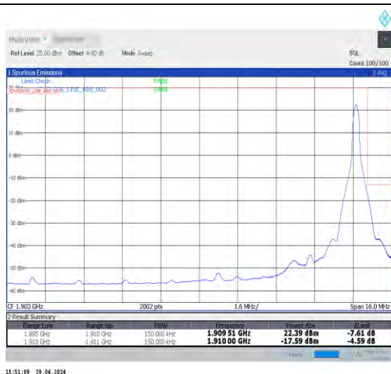
1-N2-15-15-H-2-DFT-PI2BPSK-Edge_1RB_Right-1@78-Ant0-1-seegraph-PASS-see graph
