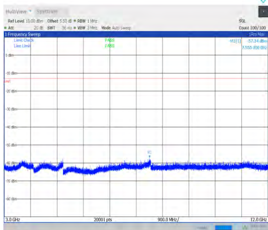
1-N2-15-20-L-1-DFT-PI2BPSK-Inner_1RB_Left-1@ 1-3000-12000-Ant0-3638.55--57.34--13-PASS
