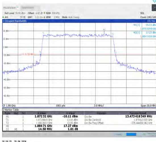
1-N2-15-15-M-1-DFT-QPSK-Outer_Full-75@0-Ant0-13.473-14.580-≤15-PASS
