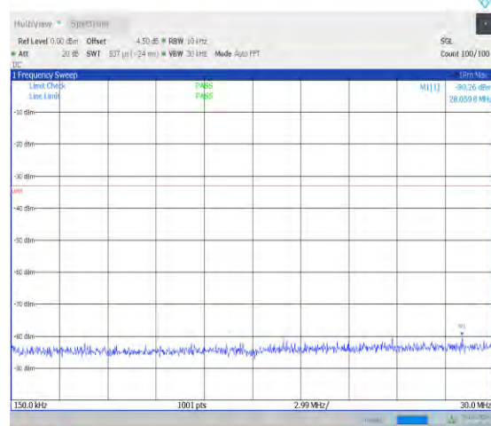
1-N2-15-20-M-1-DFT-PI2BPSK-Inner_1RB_Left-1@1 -0.15-30-Ant0-19.34--80.26--33-PASS
