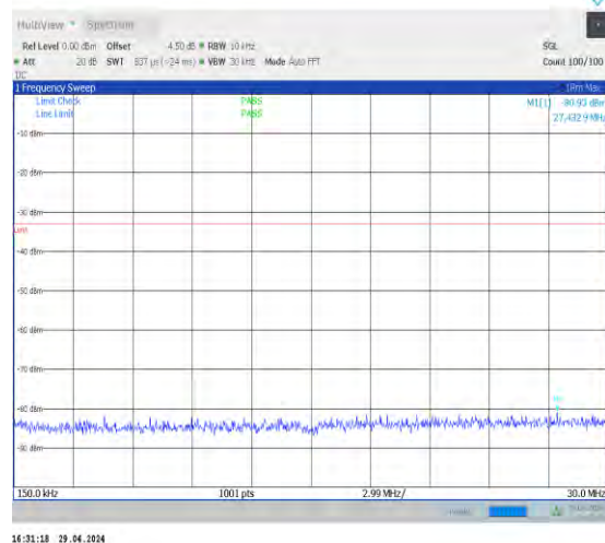
1-N2-15-20-L-1-DFT-PI2BPSK-Inner_1RB_Left-1@1- 0.15-30-Ant0-25.82--80.93--33-PASS
