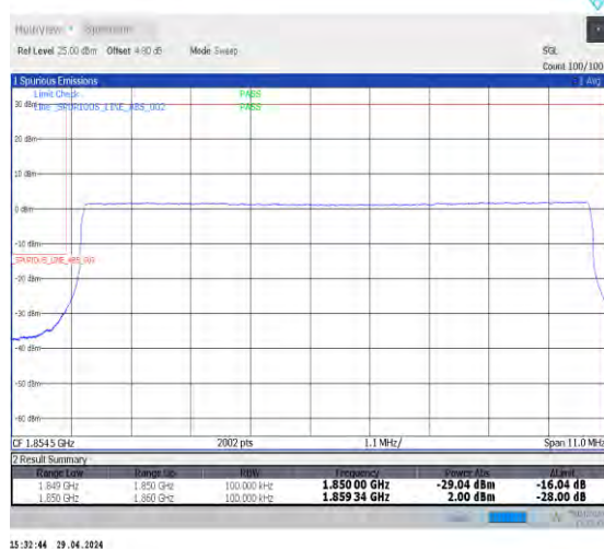
1-N2-15-10-L-6-CP-QPSK-Outer_Full-52@0-Ant0-1-seegraph-PASS-see graph
