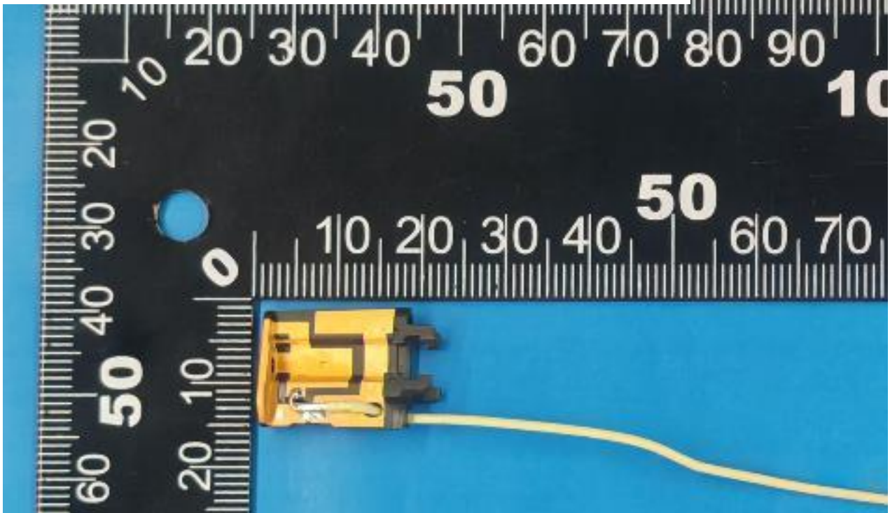
WLAN Aux. and Bluetooth Antenna for Speed Taiwan Corporation Antenna
