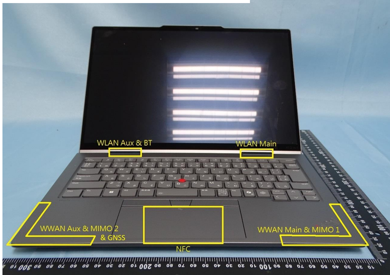
Amphenol Antenna and Speed Taiwan Corporation Antenna
