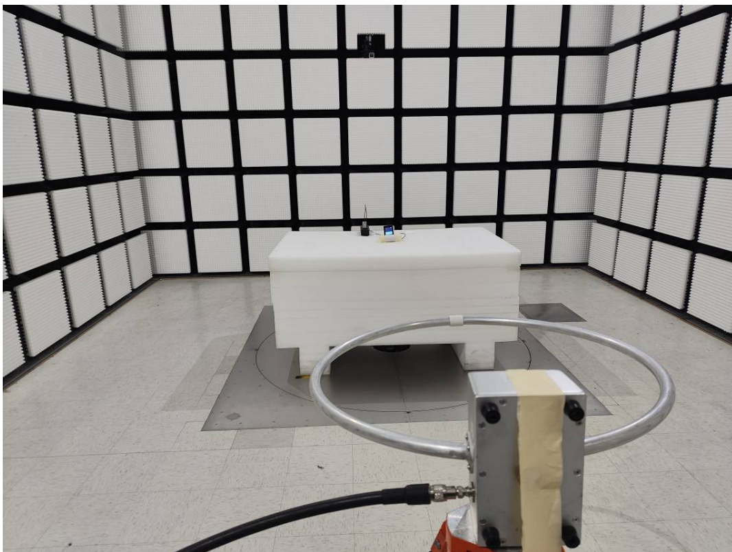
Radiated Emission 9kHz to 30MHz View Ground-parallel
