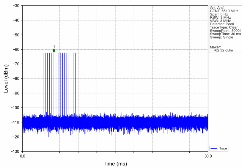
Signal Calibration_802.11n(HT40)_2C_5510MHz_RadarType3_Trial0
