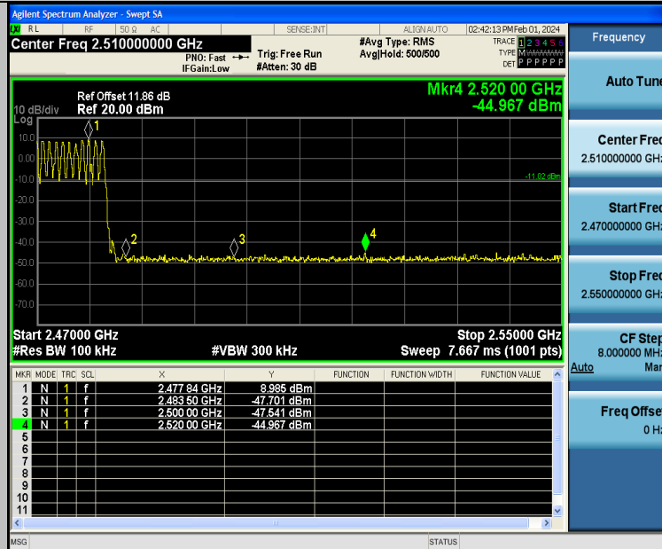
DH5-Ant2-Hop_2480-PASS
