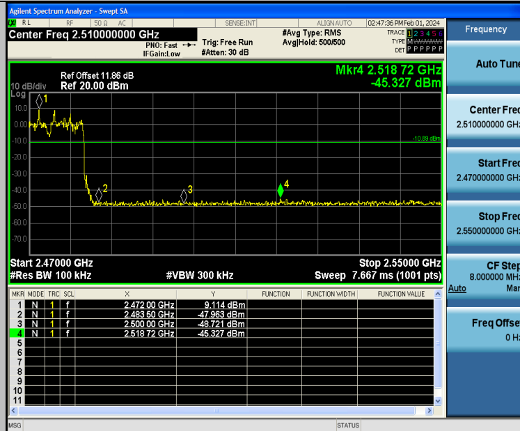
2DH5-Ant2-Hop_2480-PASS
