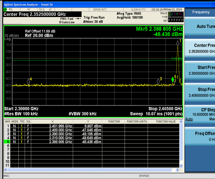
DH5-Ant2-2402-PASS
