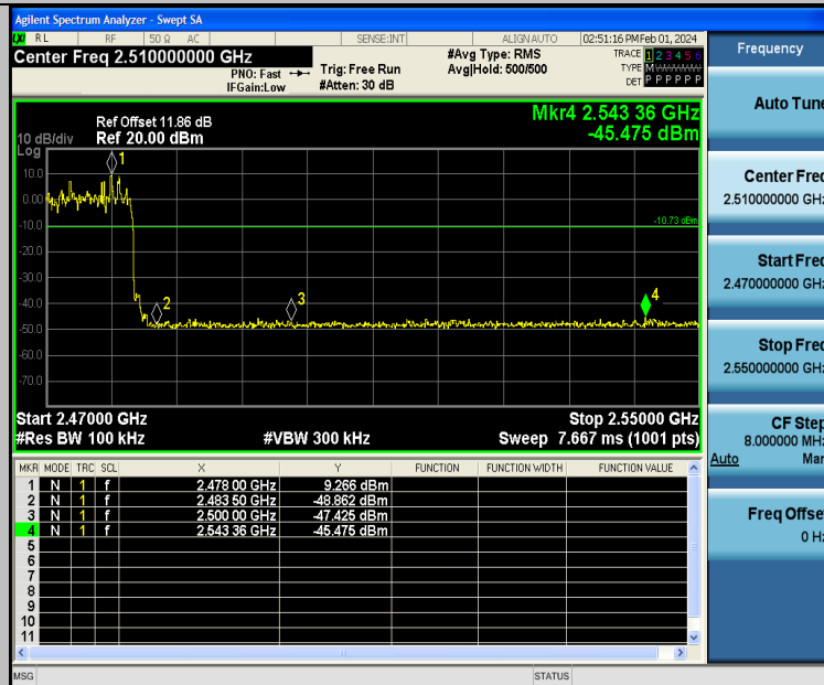
3DH5-Ant2-Hop_2480-PASS
