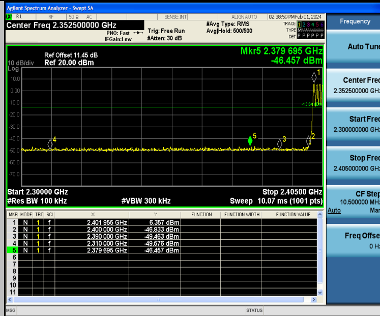
DH5-Ant2-Hop_2402-PASS
