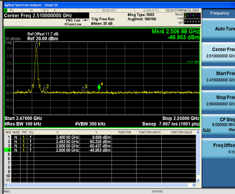
DH5-Ant2-2480-PASS
