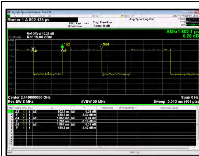
Bluetooth Low Energy 2Mbps 2440MHz
