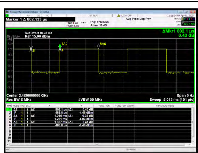
Bluetooth Low Energy 2Mbps 2480MHz
