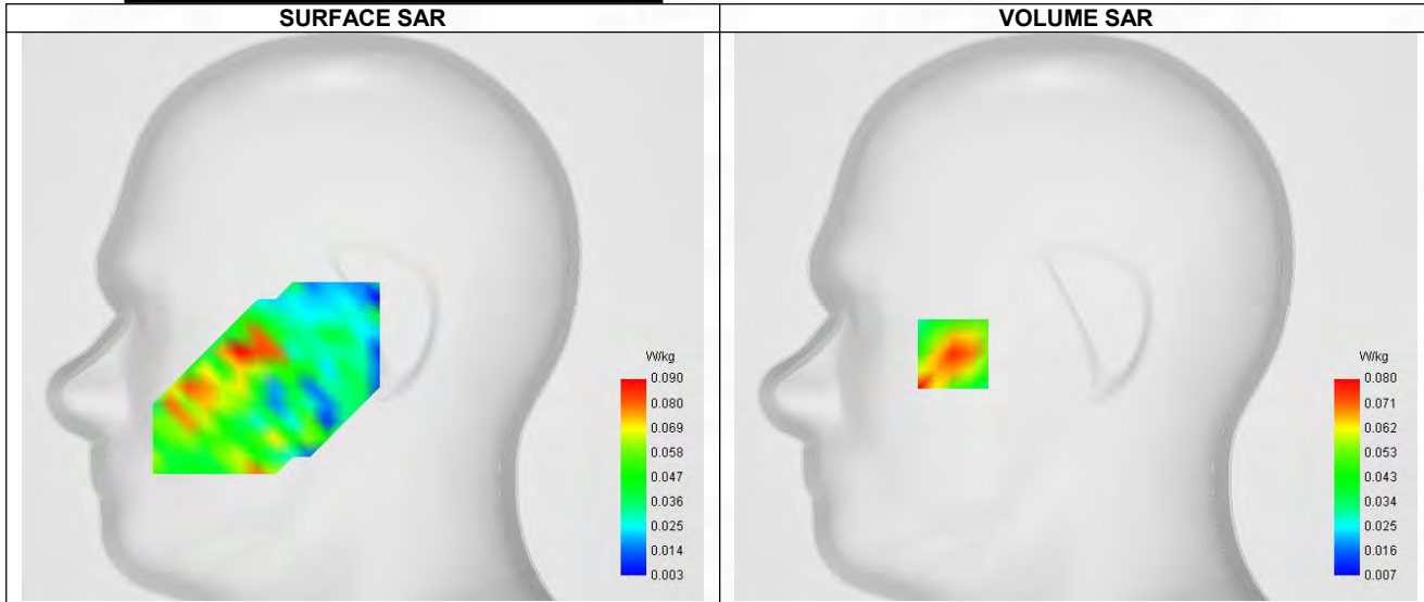
Maximum location: X=-56.00, Y=-17.00 ; SAR Peak: 0.11 W/kg
