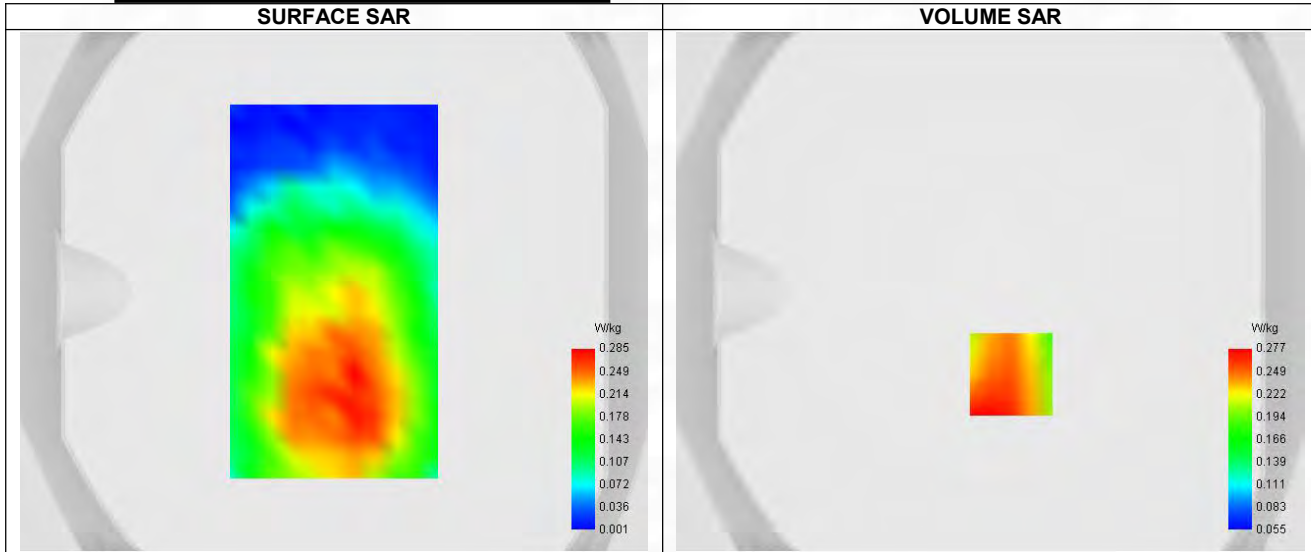
Maximum location: X=8.00, Y=-32.00 ; SAR Peak: 0.37 W/kg
