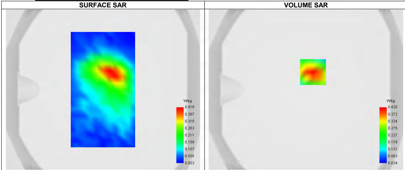
Maximum location: X=9.00, Y=22.00 ; SAR Peak: 0.64 W/kg
