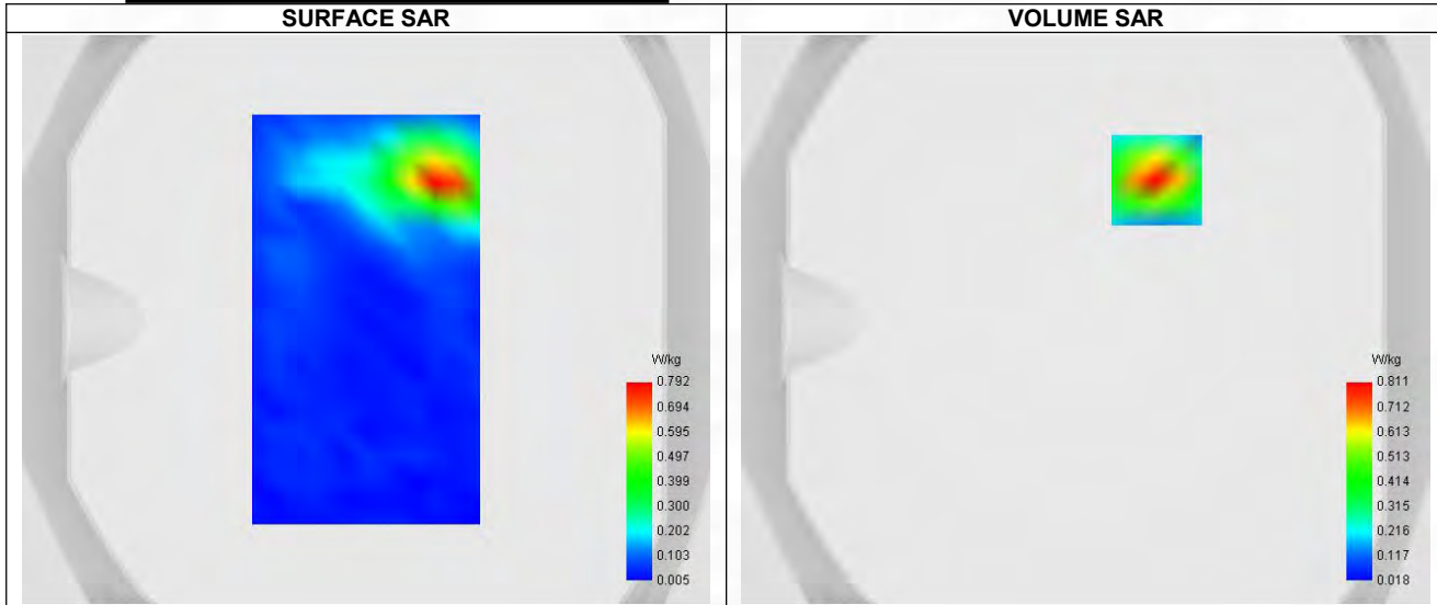
Maximum location: X=25.00, Y=49.00 ; SAR Peak: 1.44 W/kg
