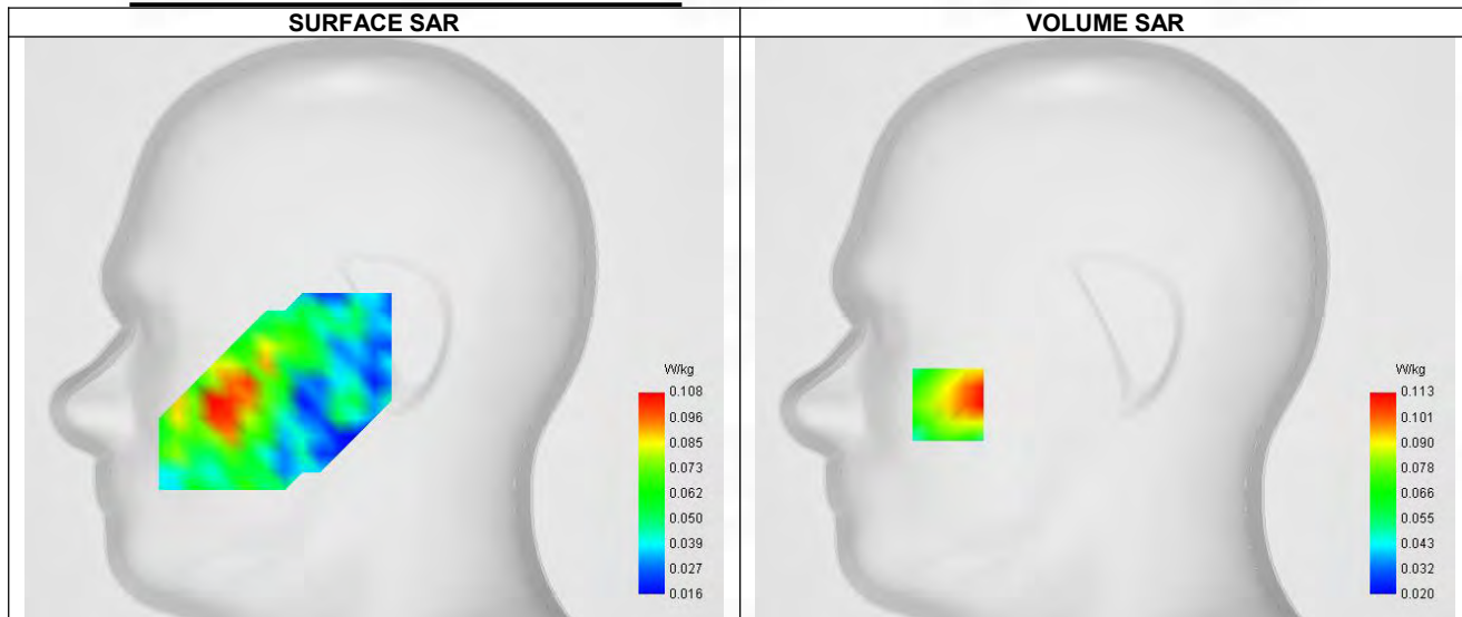
Maximum location: X=-70.00, Y=-34.00 ; SAR Peak: 0.18 W/kg
