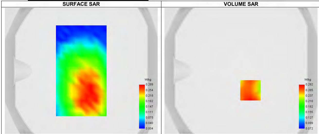
Maximum location: X=15.00, Y=-31.00 ; SAR Peak: 0.36 W/kg
