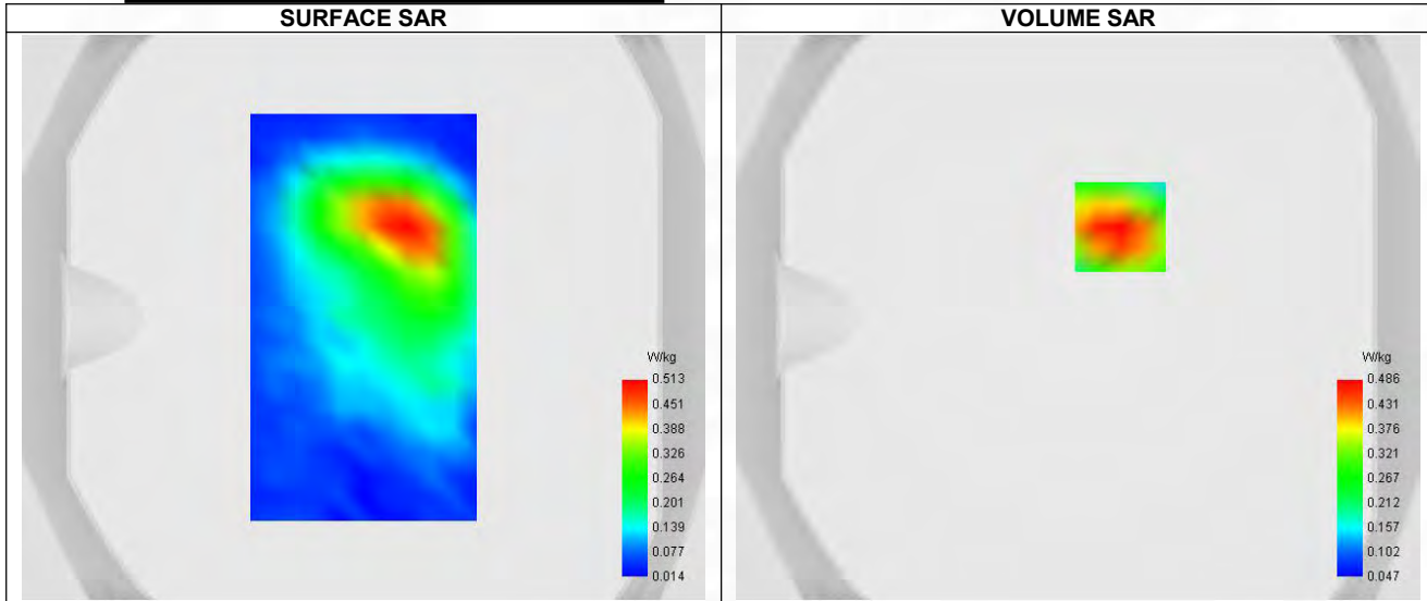
Maximum location: X=15.00, Y=32.00 ; SAR Peak: 0.68 W/kg
