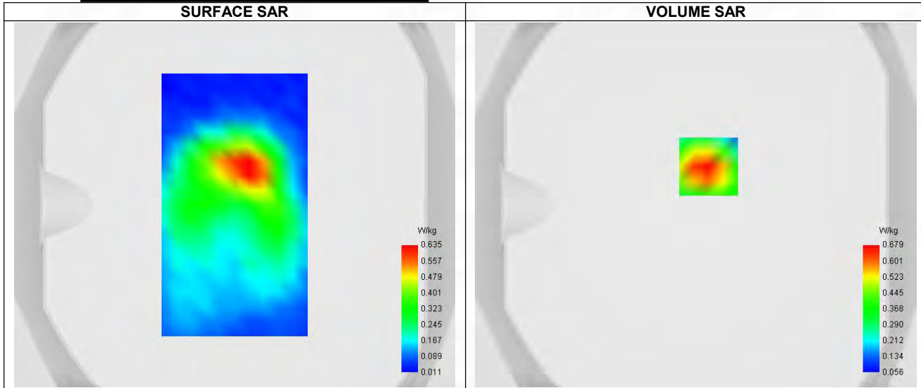
Maximum location: X=7.00, Y=21.00 ; SAR Peak: 1.03 W/kg
