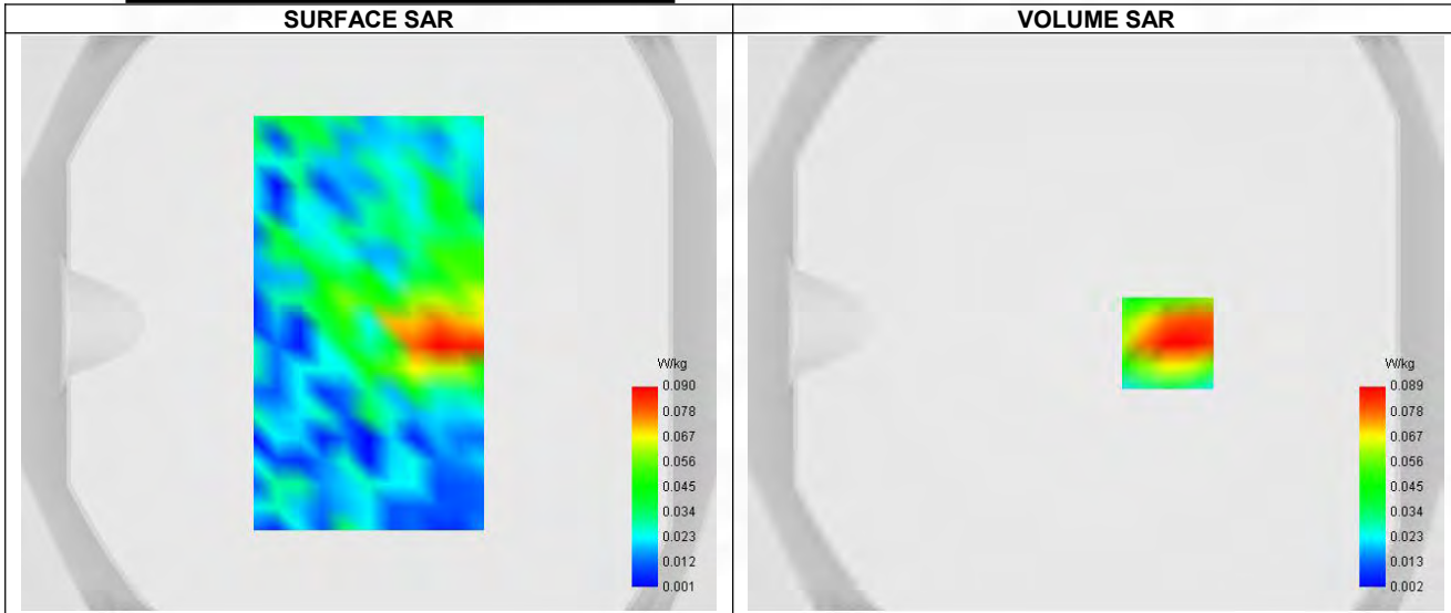
Maximum location: X=25.00, Y=-7.00 ; SAR Peak: 0.14 W/kg
