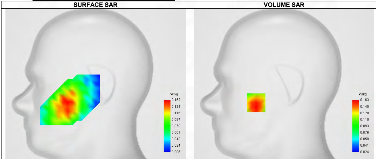
Maximum location: X=-48.00, Y=-33.00 ; SAR Peak: 0.22 W/kg
