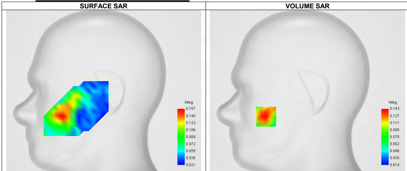
Maximum location: X=-66.00, Y=-41.00 ; SAR Peak: 0.19 W/kg
