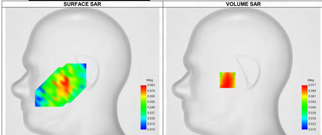
Maximum location: X=-32.00, Y=-18.00 ; SAR Peak: 0.10 W/kg
