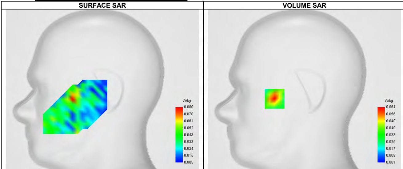
Maximum location: X=-48.00, Y=-15.00 ; SAR Peak: 0.11 W/kg
