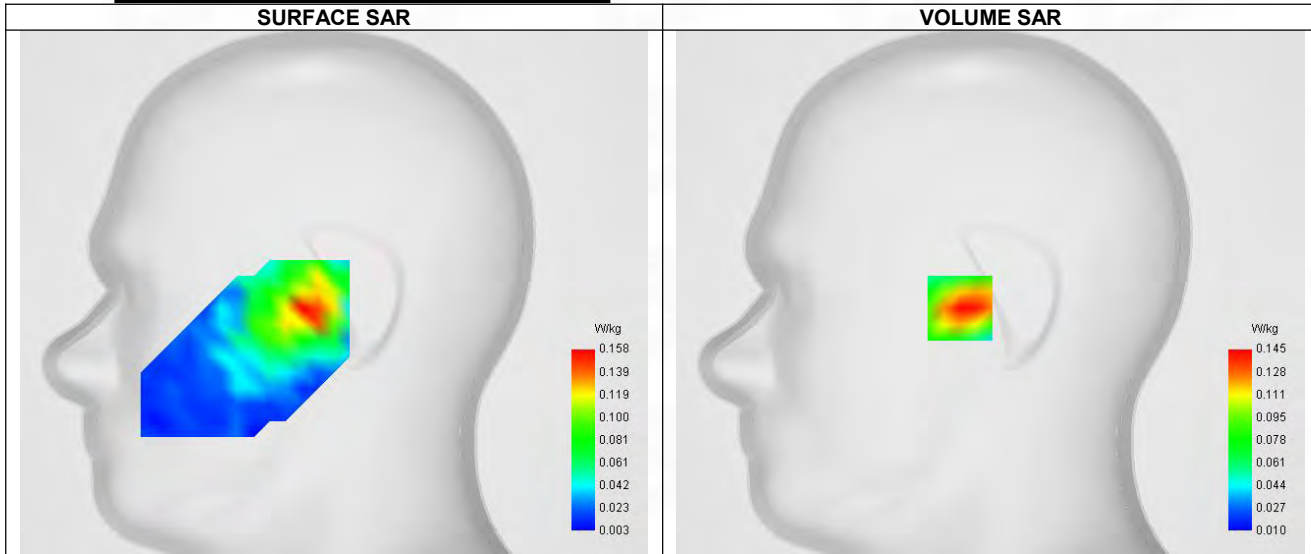
Maximum location: X=-15.00, Y=-8.00 ; SAR Peak: 0.27 W/kg
