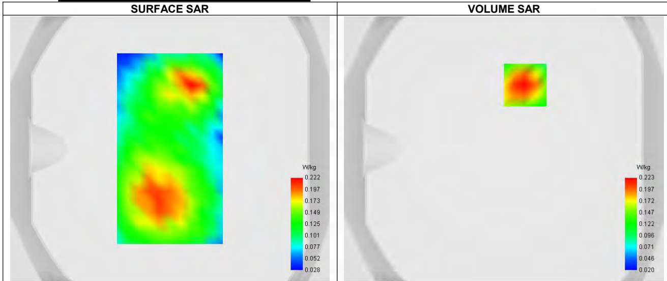
Maximum location: X=16.00, Y=48.00 ; SAR Peak: 0.30 W/kg
