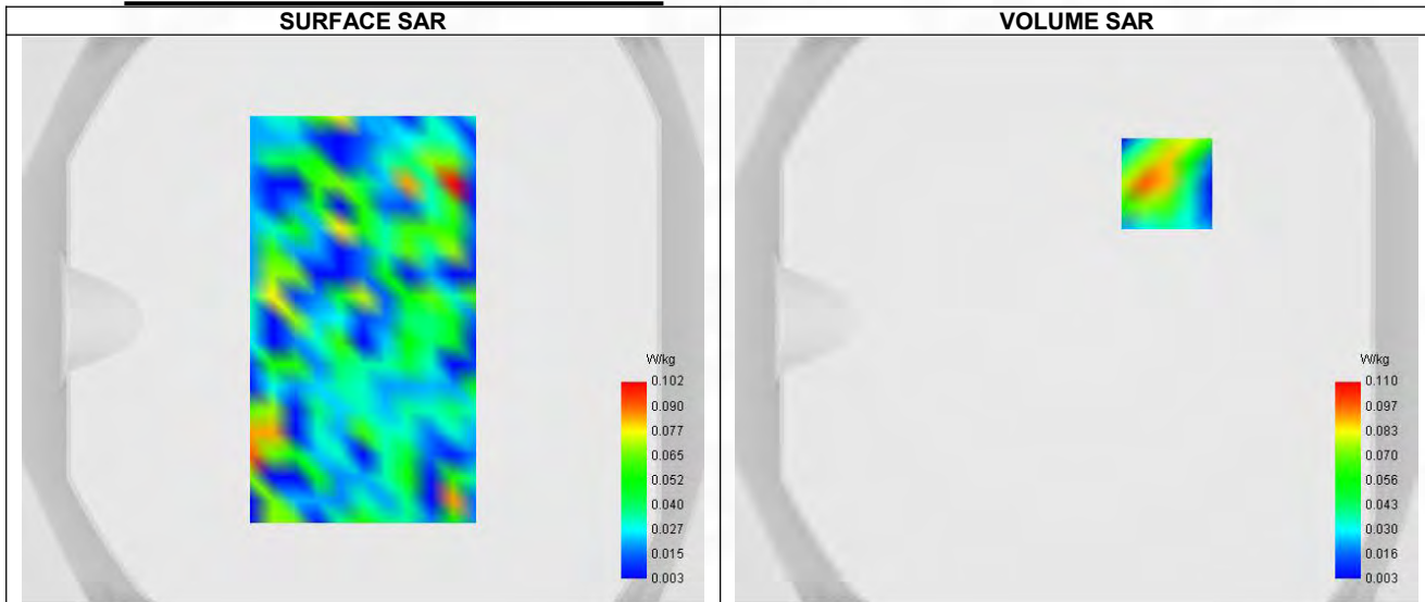
Maximum location: X=32.00, Y=48.00 ; SAR Peak: 0.09 W/kg
