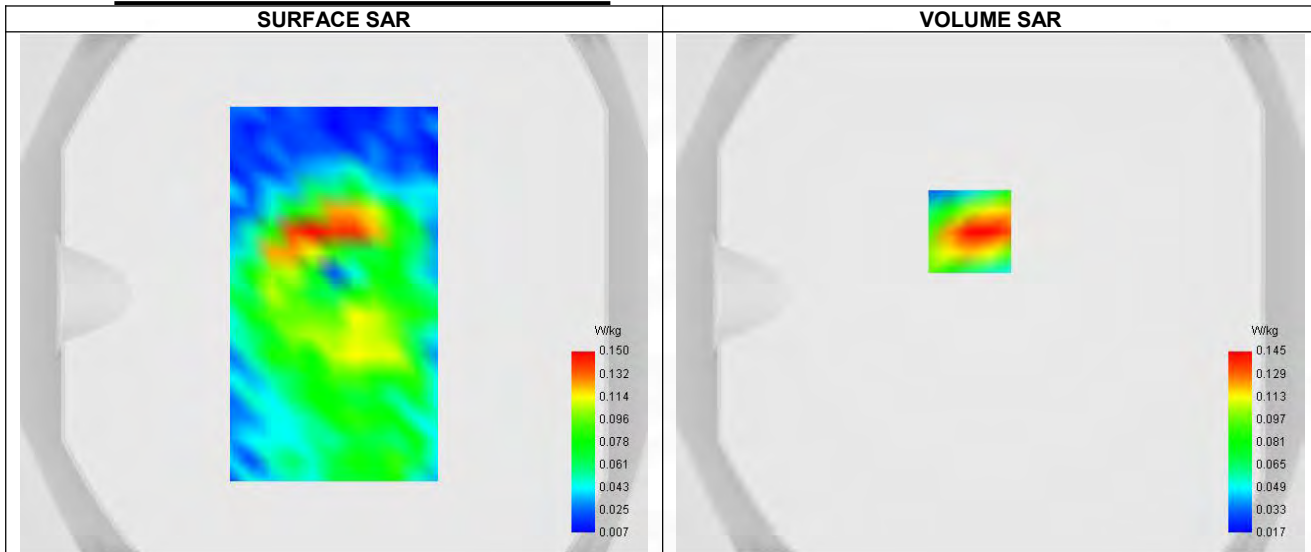
Maximum location: X=-8.00, Y=24.00 ; SAR Peak: 0.23 W/kg
