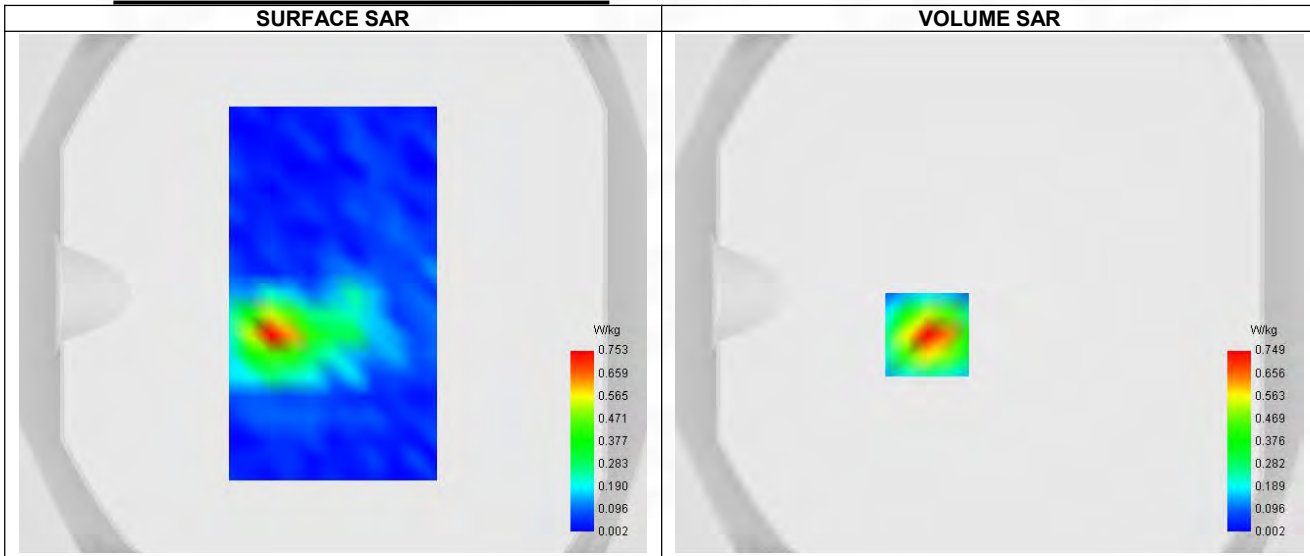
Maximum location: X=-24.00, Y=-16.00 ; SAR Peak: 1.21 W/kg
