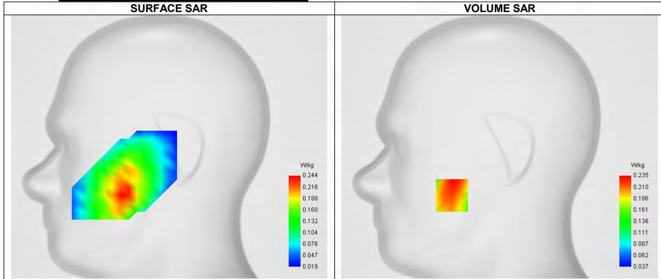
Maximum location: X=-47.00, Y=-48.00 ; SAR Peak: 0.33 W/kg
