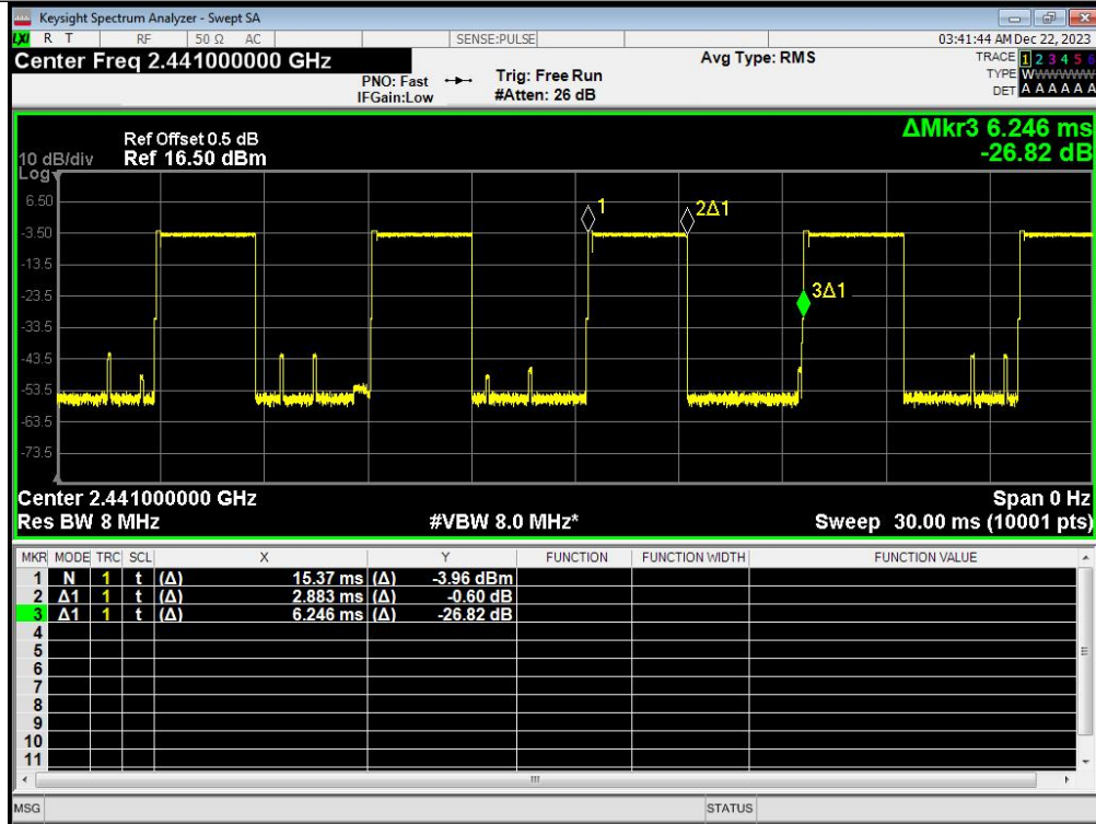
\pi/4 QPSK(2-DH5)_Channel 39
