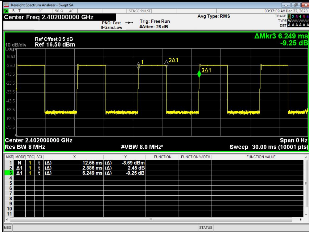
\pi/4 QPSK(2-DH5)_Channel 0
