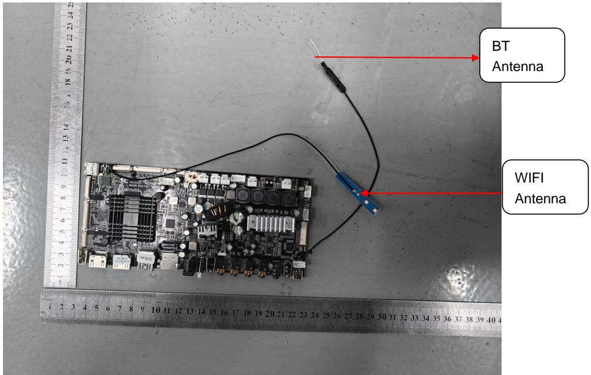
OPEN VIEW OF EUT (FIGURE 4)
