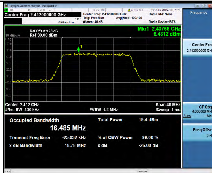
11G_Ant4_2412
