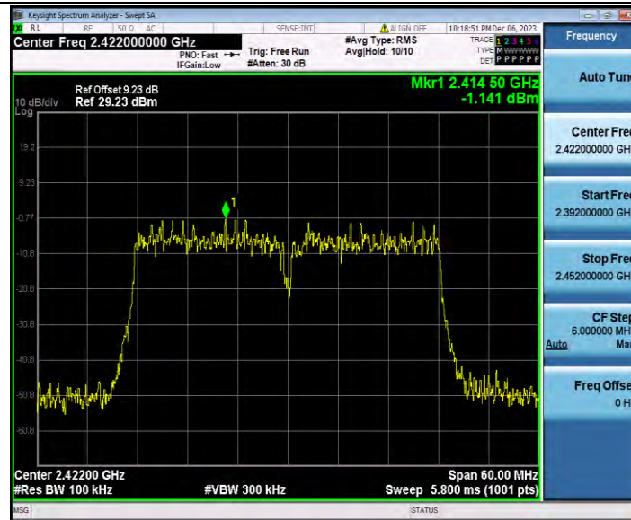
11N40SISO_Ant4_2422_0~Reference
