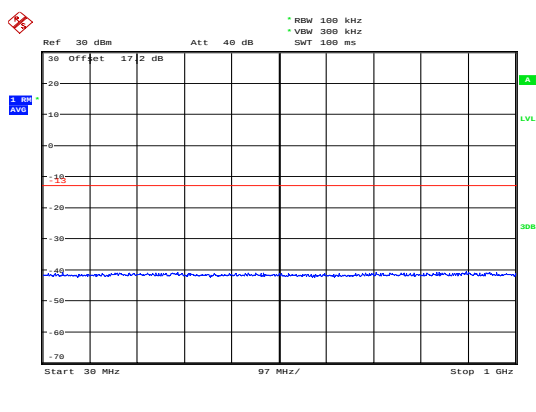
LTE Band 4 1.4MHz CH- High 30MHz~1GHz
