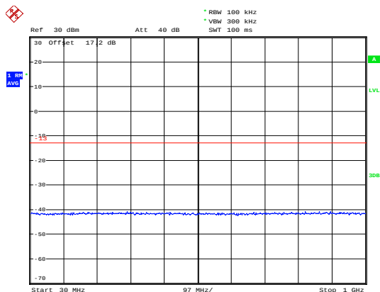
LTE Band 4 1.4MHz CH-Low 30MHz~1GHz
