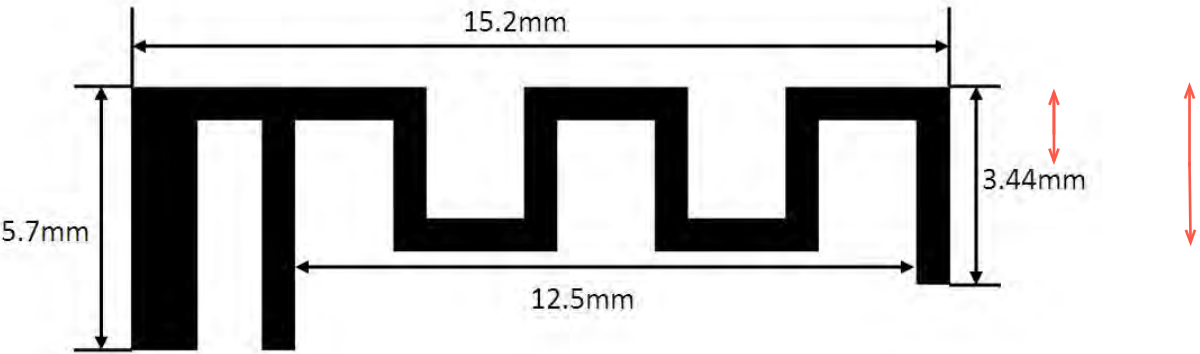
Antenna Photo & Length (mm)
