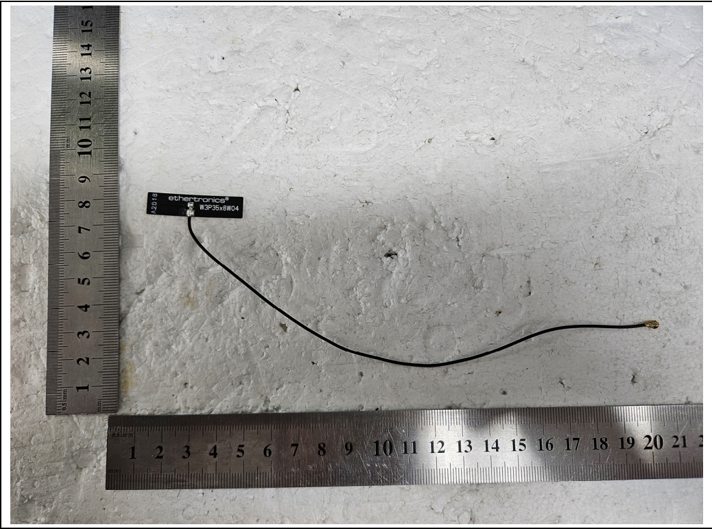
<Antenna 2 – WLAN 2.4GHz, 5GHz >
