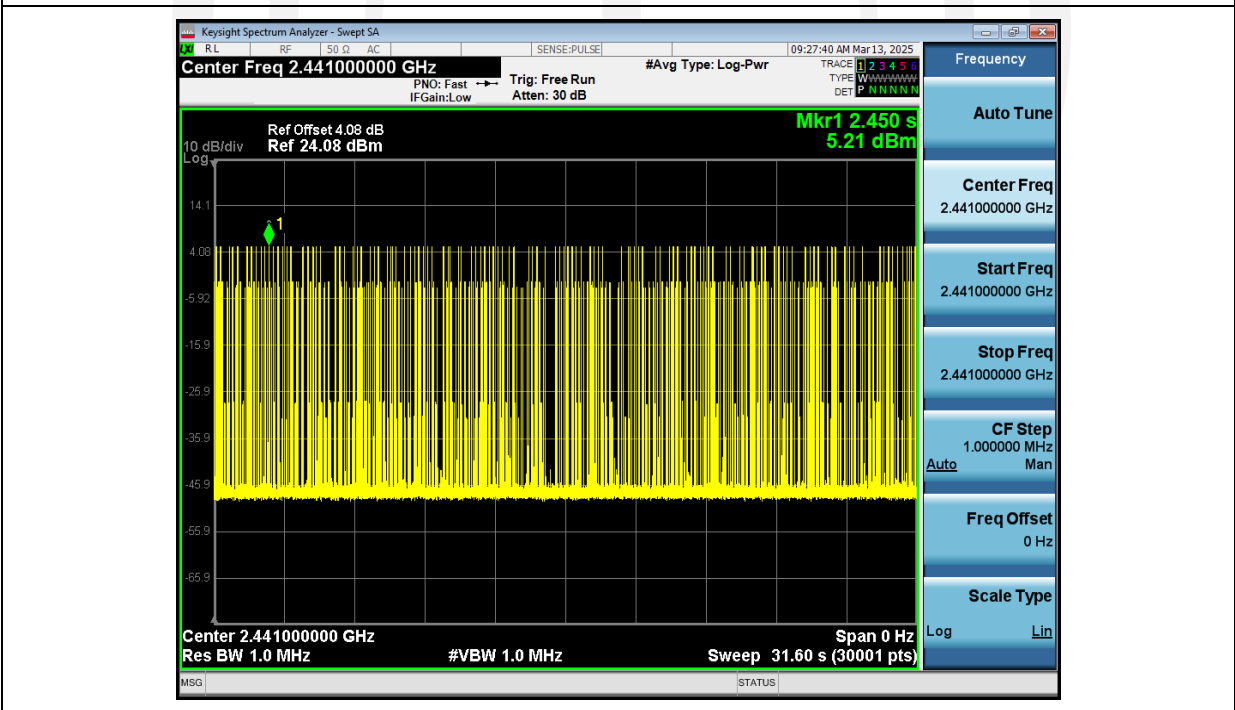
Dwell_Time_(Hopping)_NVNT_ANT1_2-DH3_2441_00_Accumulated
