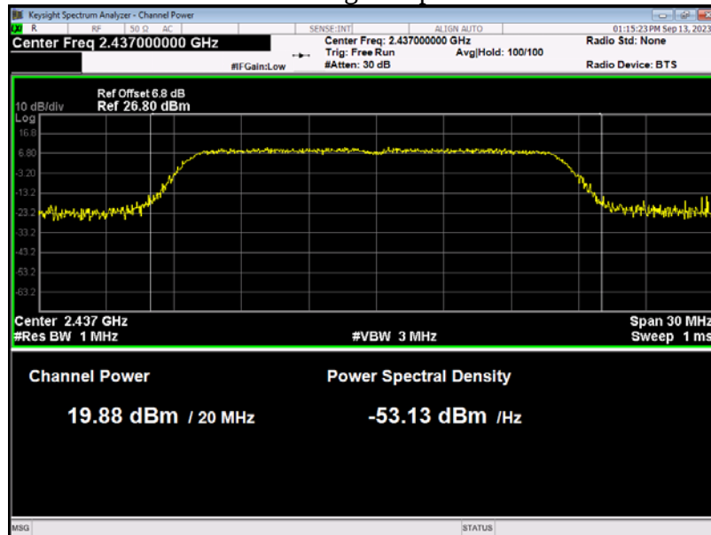
Power NVNT 802.11g 6Mbps 2437MHz Ant1
