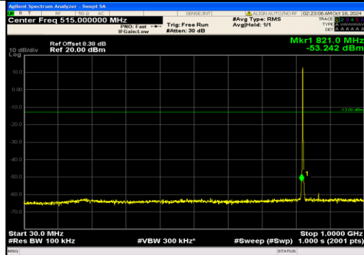
Band5_1.4MHz_16QAM_20407_6RB#0_30~1000_0.30~1000
