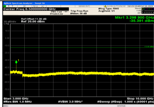
Band5_1.4MHz_16QAM_20407_6RB#0_3000~10000_0000_3000~10000
