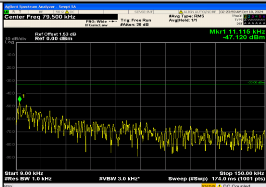
Band5_1.4MHz_16QAM_20525_6RB#0_0.009~0.15_0.009~0.15
