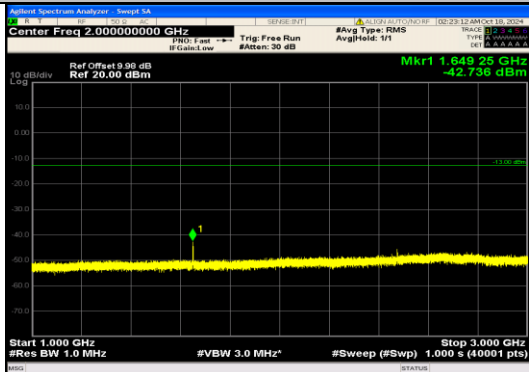
Band5_1.4MHz_16QAM_20407_6RB#0_1000~3000_000_1000~3000
