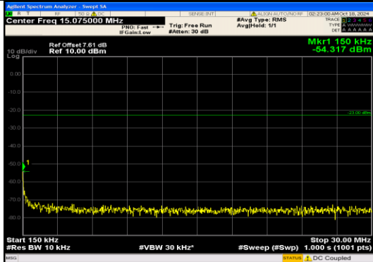
Band5_1.4MHz_16QAM_20407_6RB#0_0.15~30_0.15~30
