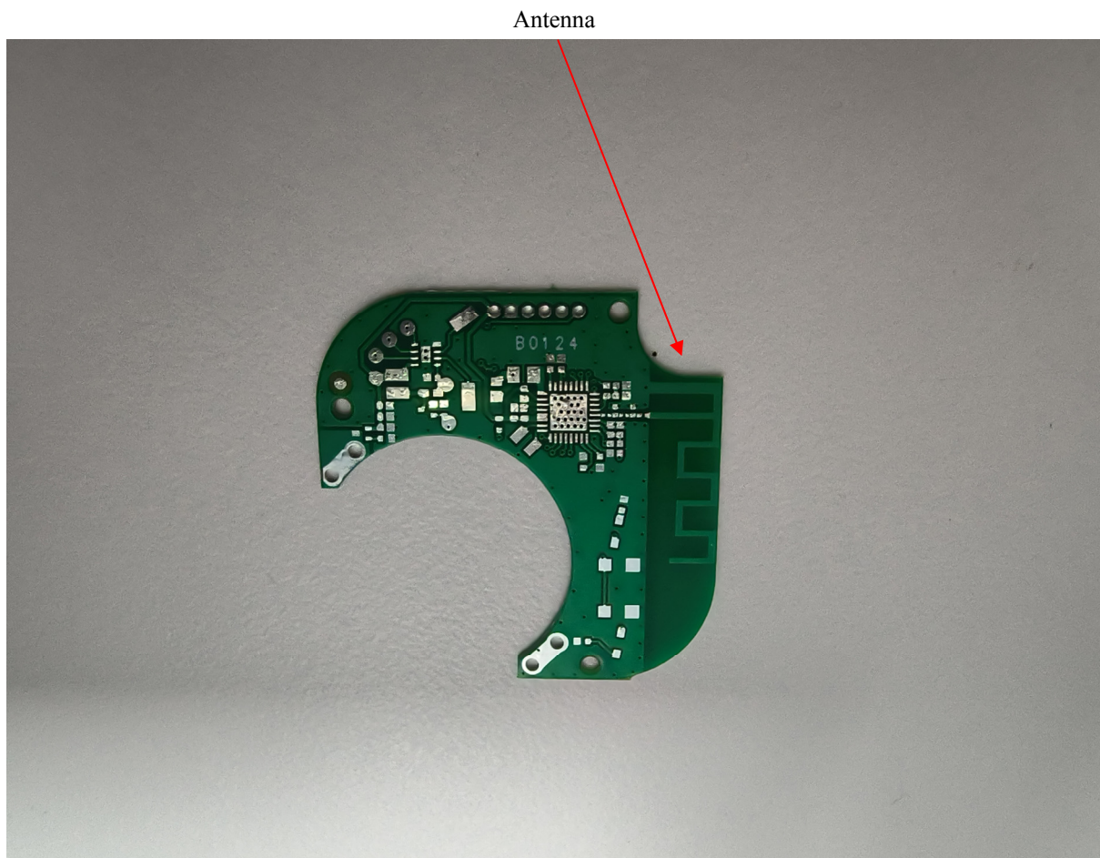
Antenna dimension
