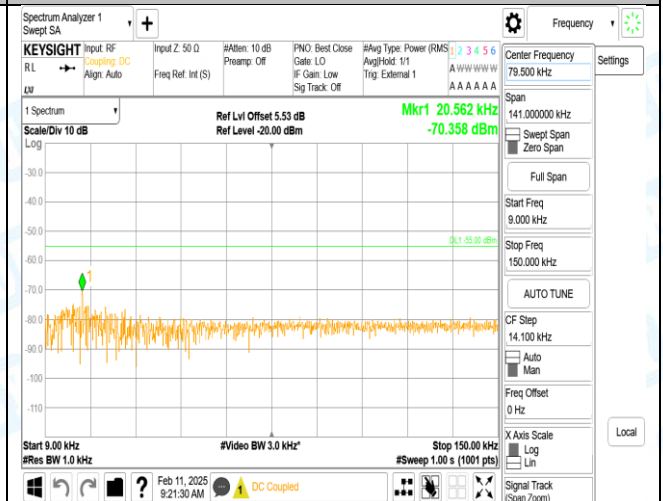
Band41_20MHz_QPSK_40690_1RB#0_0.009~0.15_0.009~0.15
