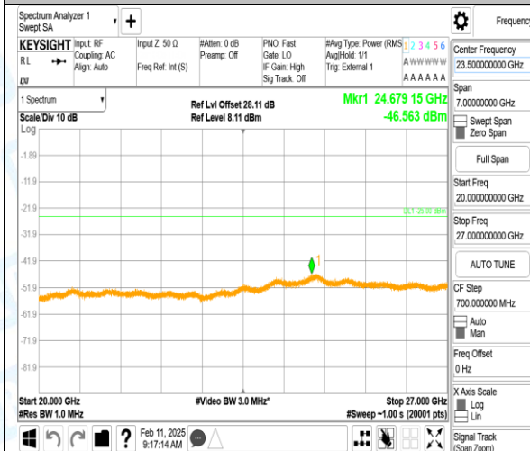
Band41_20MHz_QPSK_40340_1RB#0_20000~27000_20000~27000
