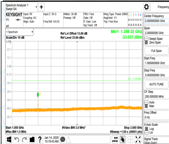
Band12_1.4MHz_16QAM_23017_1RB#_1000-3000_1000-3000
