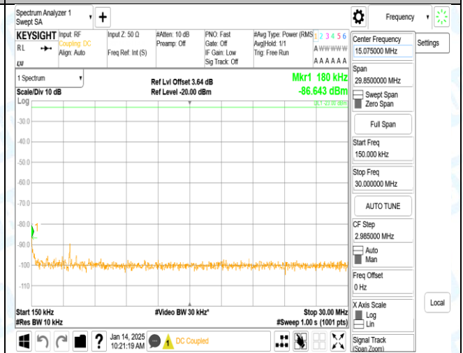
Band12_1.4MHz_16QAM_23095_1RB#_0.15-30_0.15-30
