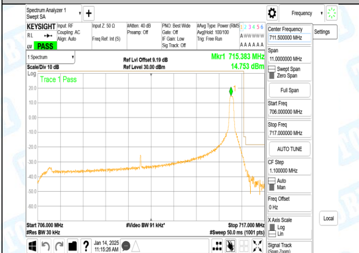
Band12_10MHz_QPSK_23130_1RB#49
