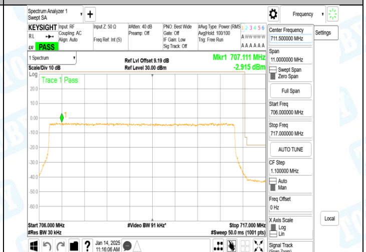
Band12_10MHz_16QAM_23130_50RB#0
