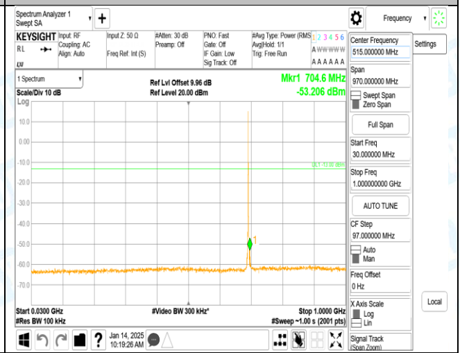
Band12_1.4MHz_16QAM_23017_1RB#0_30~1000_30~1000
