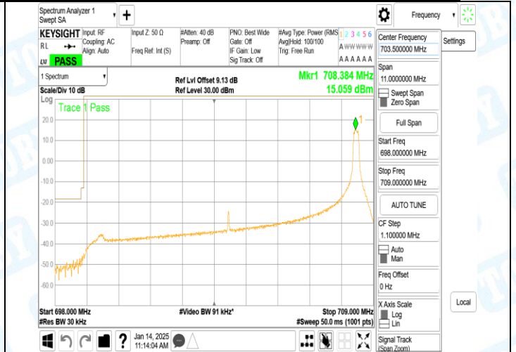
Band12_10MHz_QPSK_23060_1RB#49
