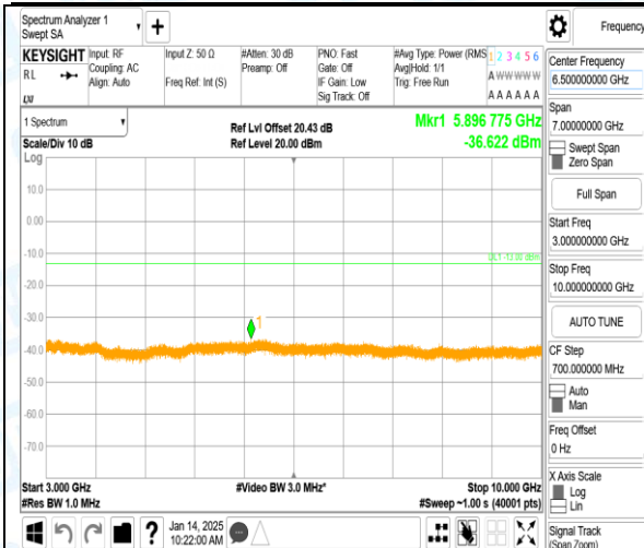
Band12_1.4MHz_16QAM_23095_1RB#0_3000~10000_3000~10000
