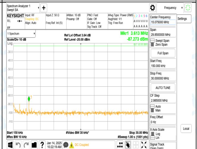
Band12_1.4MHz_QPSK_23173_1RB#0_0.15~30.015~30
