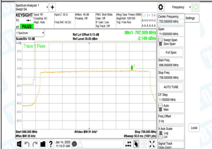
Band12_10MHz_QPSK_23060_50RB#0
