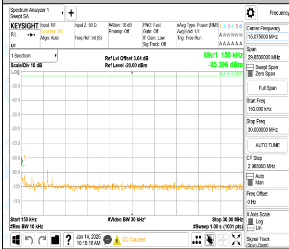
Band12_1.4MHz_16QAM_23017_1RB#0_0.15~30_0.15~30
