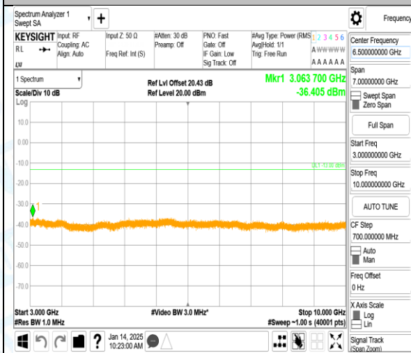
Band12_1.4MHz_QPSK_23173_1RB#0_3000~10000_3000~10000
