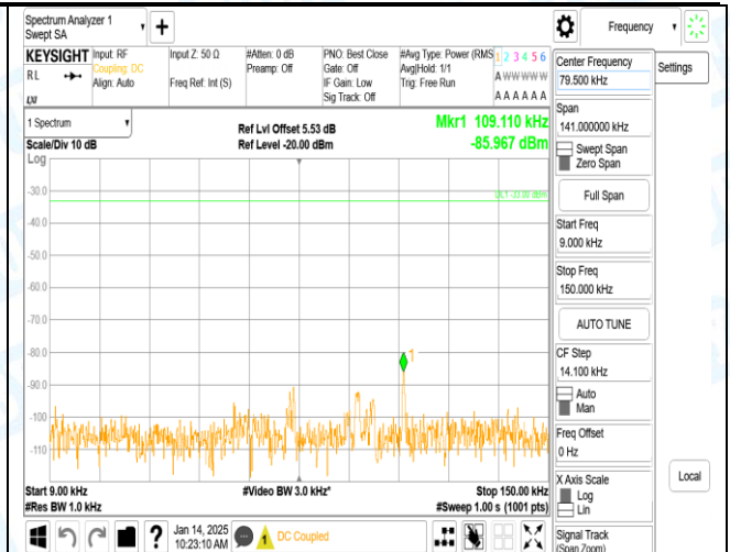
Band12_1.4MHz_16QAM_23173_1RB#0_0.009~0.15_0.009~0.15
