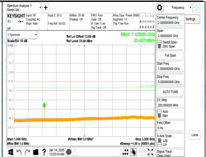
Band12_1.4MHz_QPSK_23173_1RB#0_1000~3000_1000~3000
