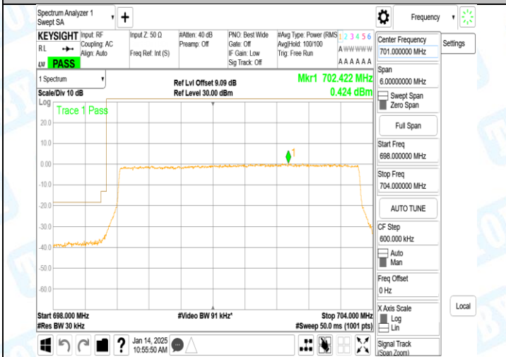
Band12_5MHz_16QAM_23035_25RB#0
