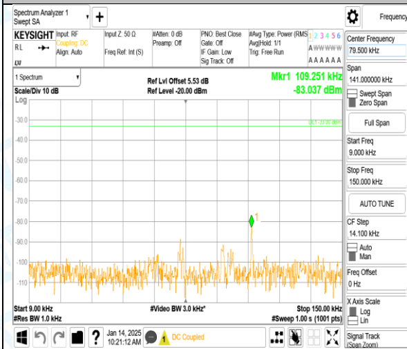
Band12_1.4MHz_16QAM_23095_1RB#_0.009-0.15_0.009-0.15
