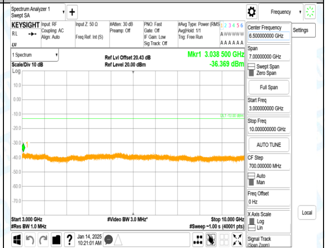
Band12_1.4MHz_QPSK_23095_1RB#0_3000~10000.3000~10000
