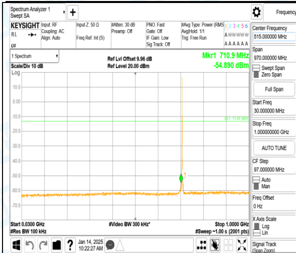
Band12_1.4MHz_QPSK_23173_1RB#0_30~1000_30~1000
