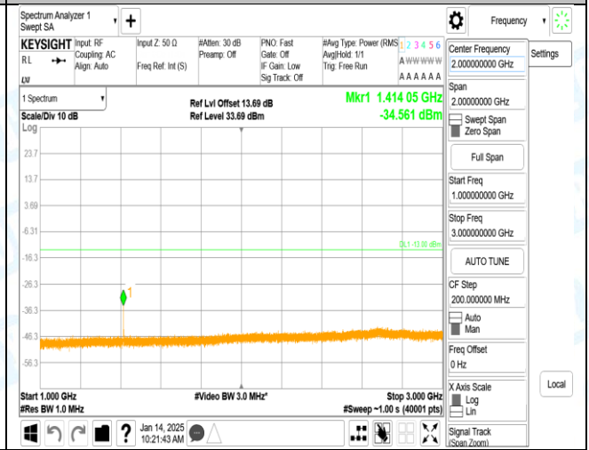
Band12_1.4MHz_16QAM_23095_1RB#_1000-3000_1000-3000
