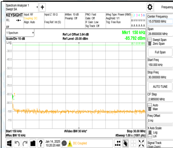
Band12_1.4MHz_QPSK_23095_1RB#0_0.15~30.015~30
