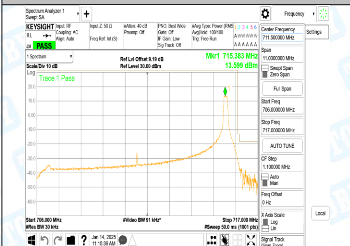
Band12_10MHz_16QAM_23130_1RB#49
