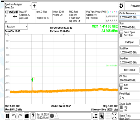
Band12_1.4MHz_QPSK_23095_1RB#0_1000~3000.1000~3000
