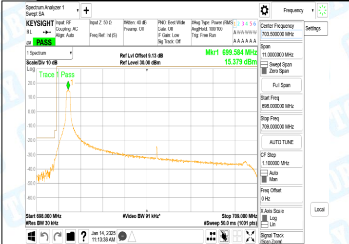
Band12_10MHz_QPSK_23060_1RB#0
