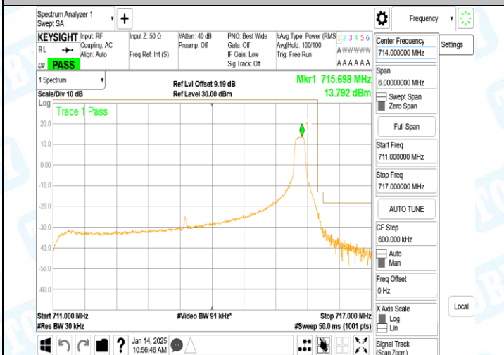
Band12_5MHz_16QAM_23155_1RB#24
