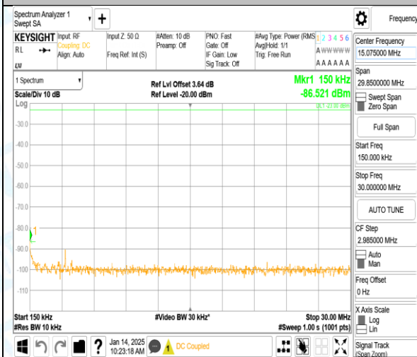
Band12_1.4MHz_16QAM_23173_1RB#0_0.15~30_0.15~30
