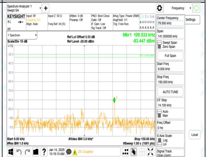
Band12_1.4MHz_16QAM_23017_1RB#0_0.009~0.15_0.009~0.15
