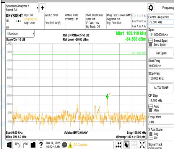
Band12_1.4MHz_QPSK_23173_1RB#0_0.009~0.15.009~0.15
