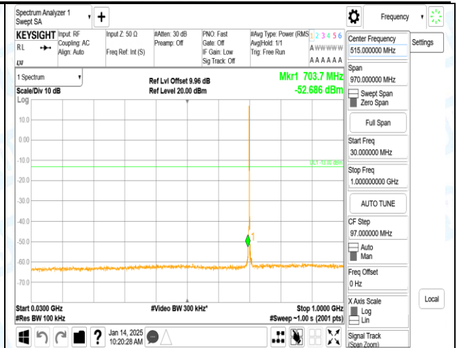
Band12_1.4MHz_QPSK_23095_1RB#0_30~1000.30~1000
