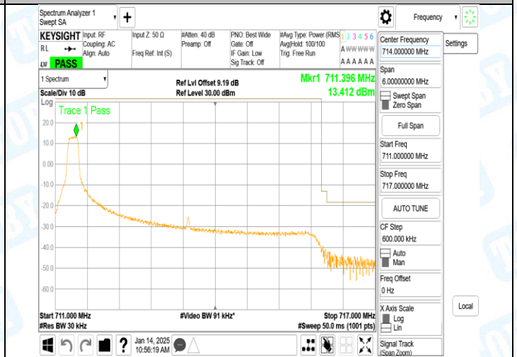
Band12_5MHz_16QAM_23155_1RB#0
