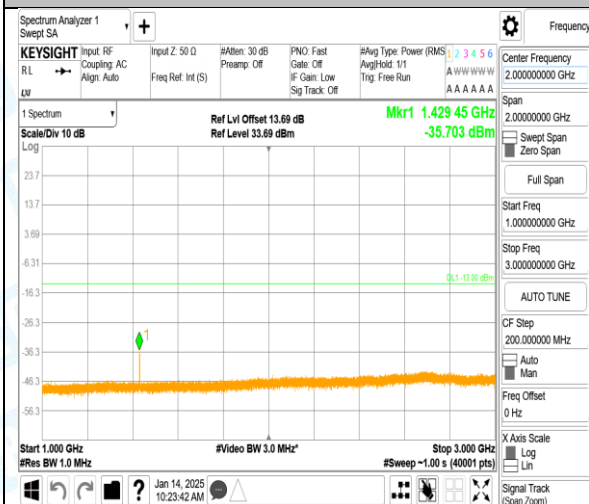
Band12_1.4MHz_16QAM_23173_1RB#0_1000~3000_1000~3000
