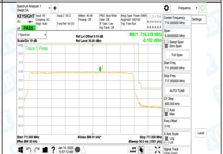
Band12_5MHz_16QAM_23155_25RB#0
