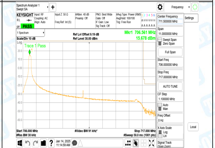
Band12_10MHz_QPSK_23130_1RB#0
