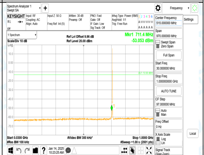
Band12_1.4MHz_16QAM_23173_1RB#0_30~1000_30~1000
