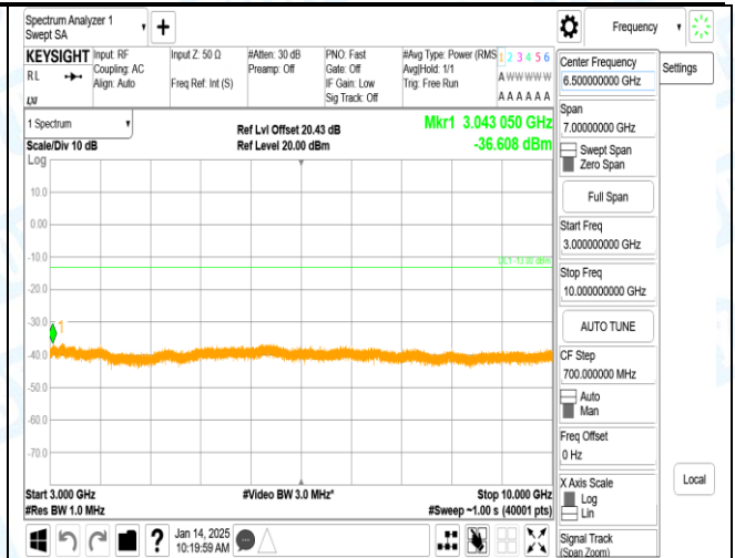
Band12_1.4MHz_16QAM_23017_1RB#_3000-10000_3000-10000
