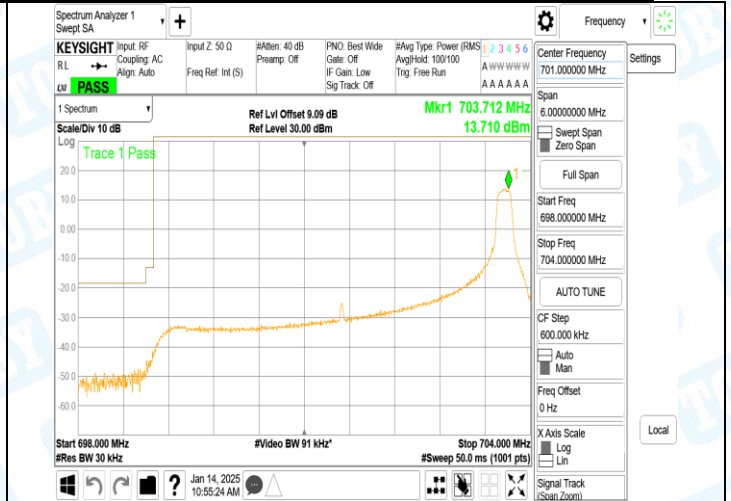
Band12_5MHz_16QAM_23035_1RB#24
