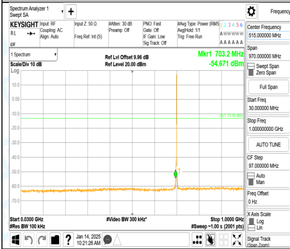
Band12_1.4MHz_16QAM_23095_1RB#_0_30-1000_30-1000
