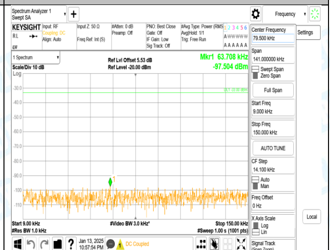
Band5_3MHz_QPSK_20525_1RB#0_0.009~0.15_0.009~0.15
