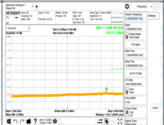
Band5_3MHz_QPSK_20415_1RB#0_1000~3000_1000~3000
