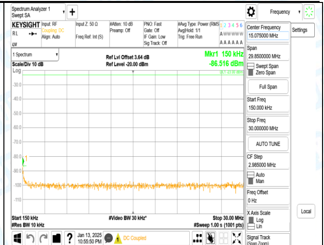
Band5_3MHz_QPSK_20415_1RB#0_0.15~30_0.15~30
