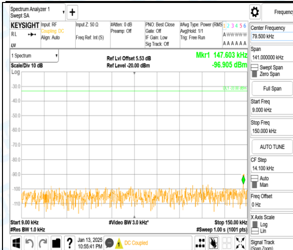
Band5_3MHz_QPSK_20415_1RB#0_0.009~0.15_0.009~0.15
