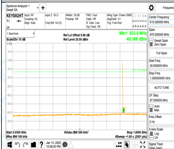
Band5_3MHz_QPSK_20415_1RB#0_30~1000_30~1000
