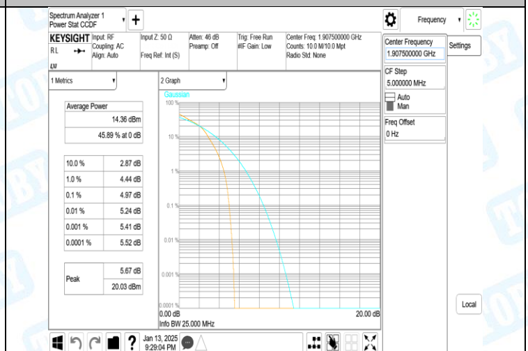
Band2-5MHz-16QAM-19175-25RB#0-PASS
