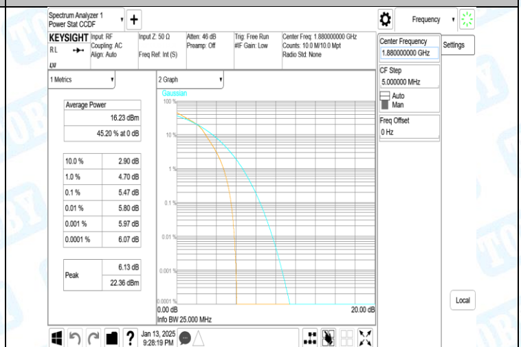
Band2-5MHz-16QAM-18900-25RB#0-PASS
