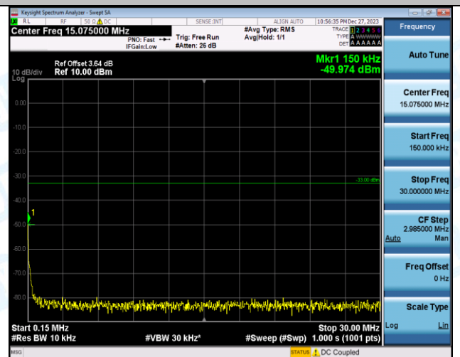
Band66_3MHz_QPSK_132322_1RB#0_15.075000 MHz
