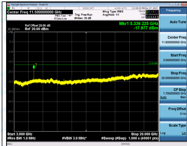
Band66_3MHz_QPSK_131987_1RB#0_30~1000_30~1000
