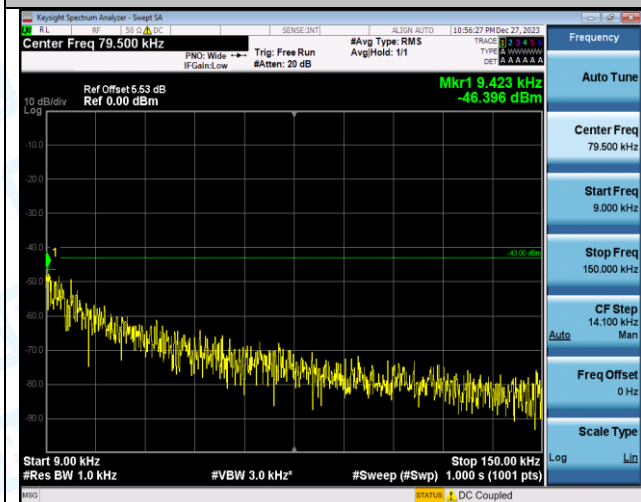
Band66_3MHz_QPSK_132322_1RB#0_0.009~0.15_0.009~0.15
