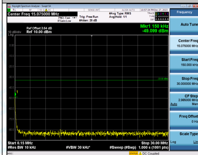
Band66_3MHz_16QAM_132322_1RB#0_1000~3000_1000~3000
