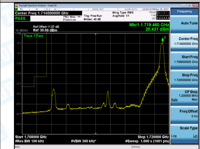
Band4_10MHz_16QAM_20000_50RB#0
