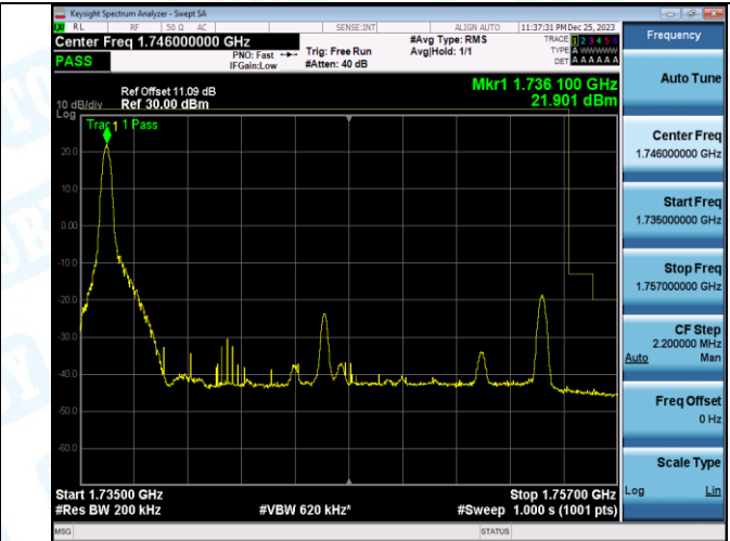
Band4_20MHz_16QAM_20300_1RB#99
