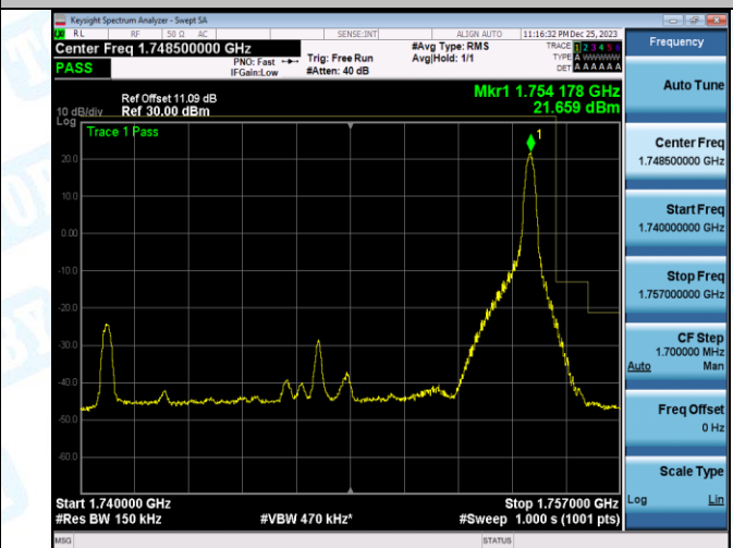
Band4_15MHz_16QAM_20325_75RB#0
