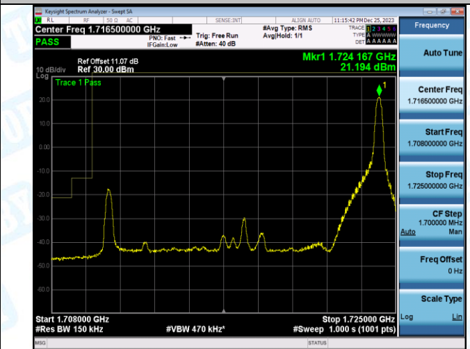
Band4_15MHz_16QAM_2025_75RB#0
