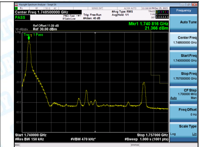
Band4_15MHz_16QAM_20325_1RB#74
