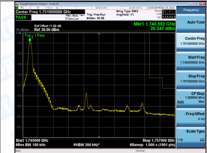
Band4_10MHz_16QAM_20350_1RB#49
