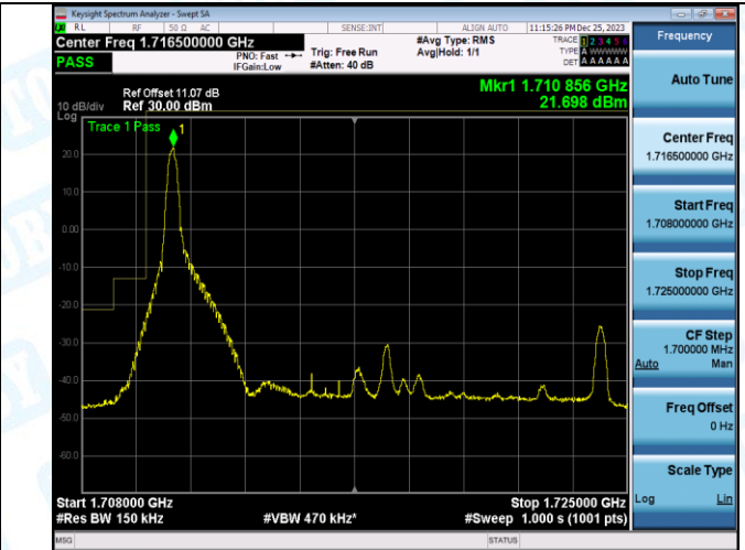
Band4_15MHz_16QAM_2025_1RB#74
