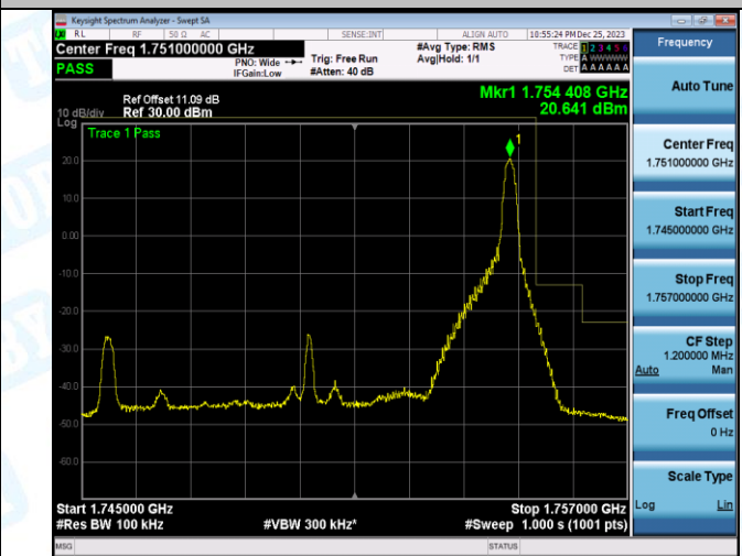
Band4_10MHz_16QAM_20350_50RB#0
