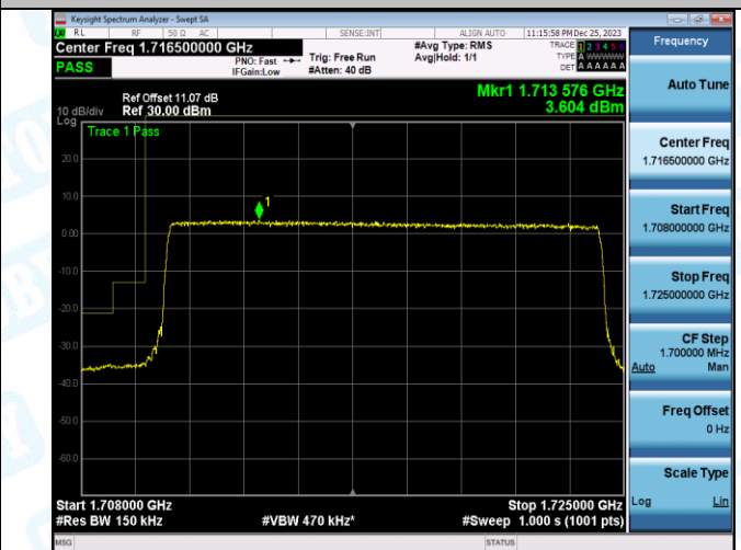
Band4_15MHz_16QAM_2025_1RB#0
