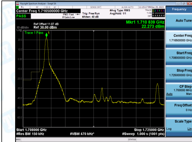
Band4_15MHz_QPSK_2025_1RB#74
