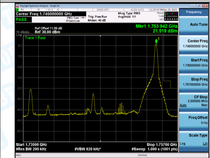
Band4_20MHz_16QAM_20300_100RB#0
