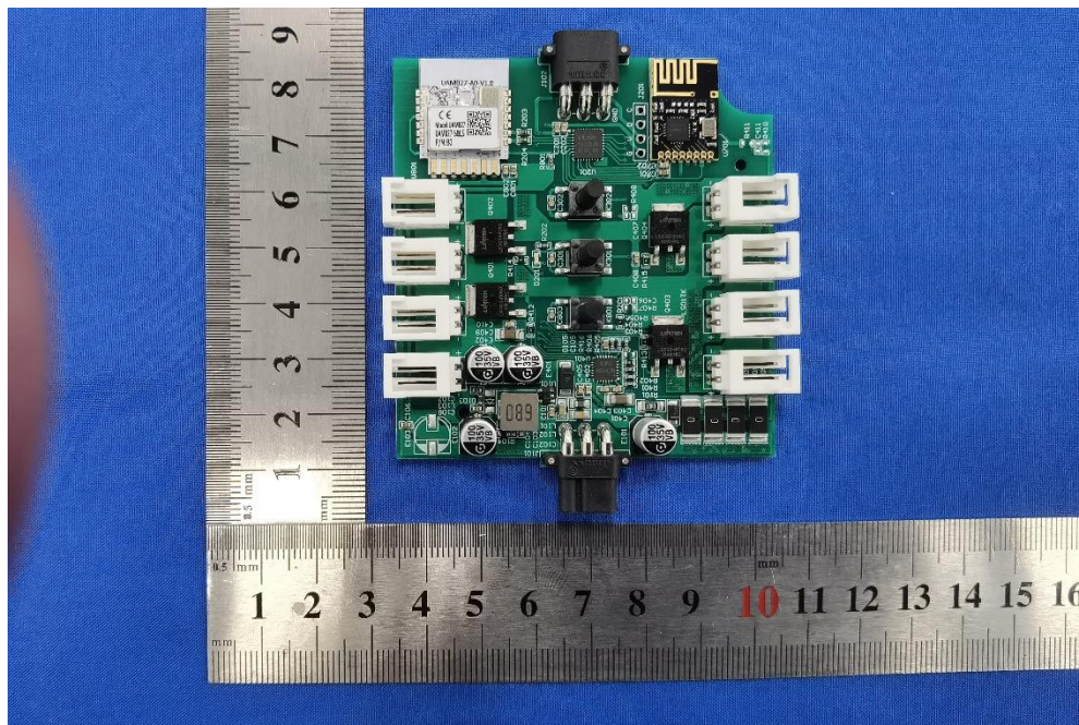
Photo 2: Internal View for PCB
