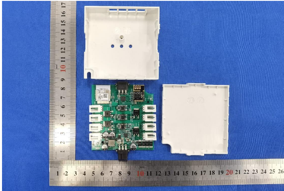
Photo 1: Internal View
