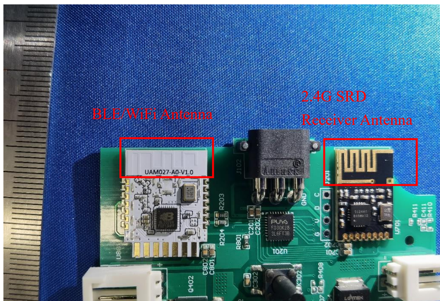
Photo 5: Antenna
