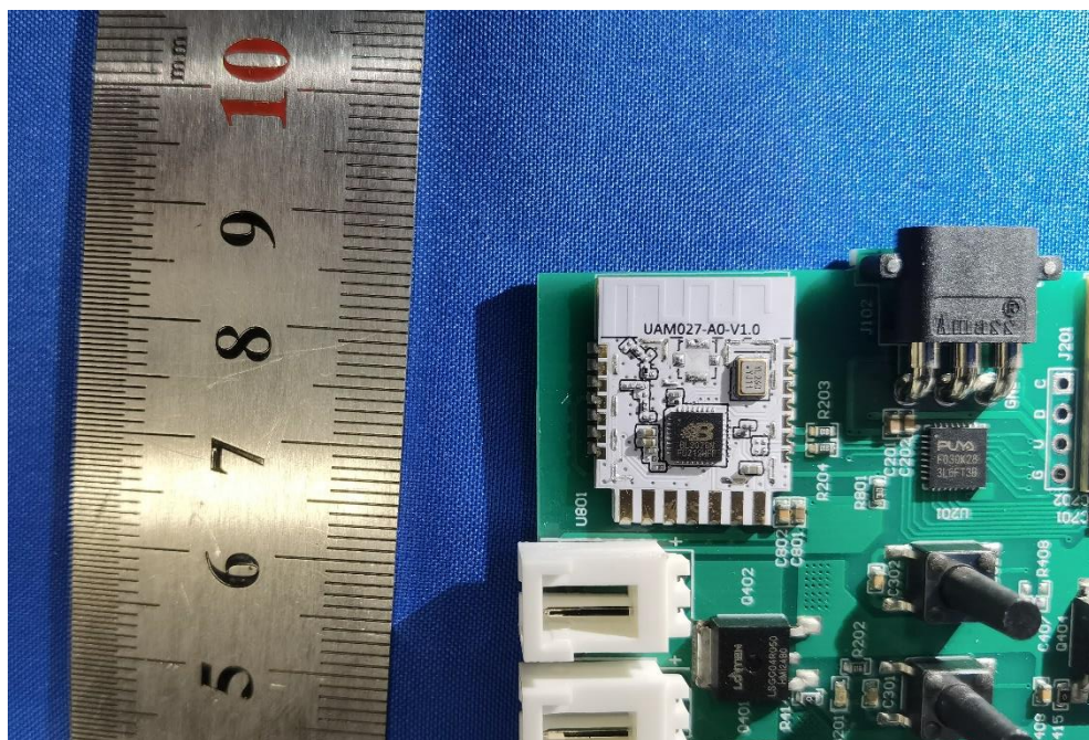
Photo 4: Internal View for PCB
