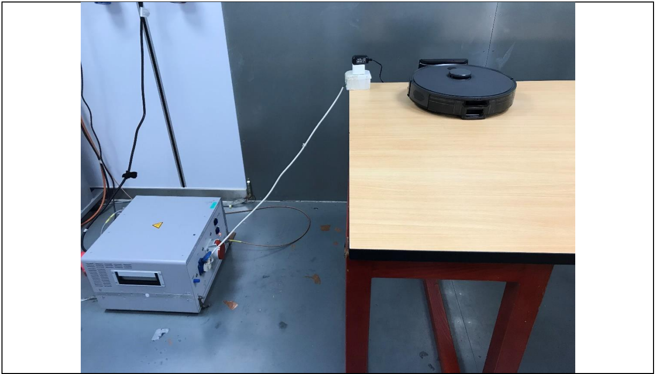
Conducted Emission test for X950
