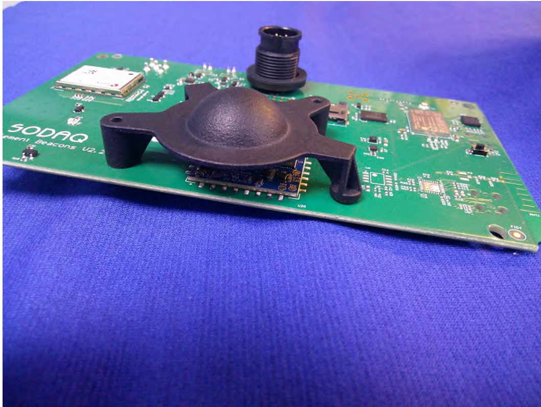
60GHz RADAR antenna with lens
